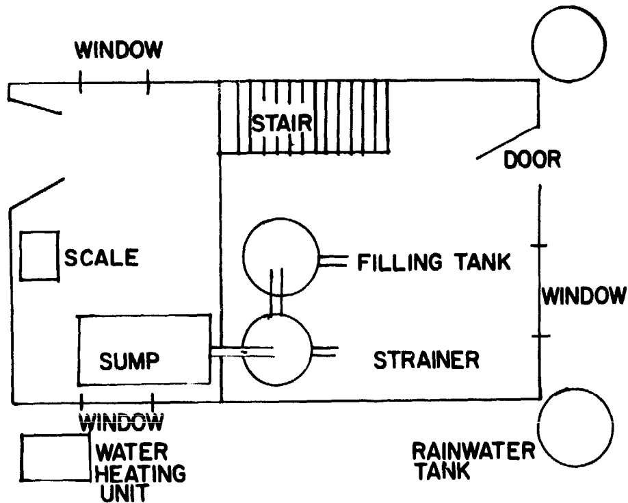
Fig. 6/4 Plan of a simple honey-collecting centre on a hillside. Two rain-water tanks (right) are at the lower end of the building, while the unloading door and scales are at the higher end.
