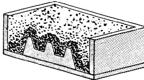
Filled with resin coated sand which cures against the hot pattern
