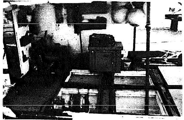
Fig. 4. View of Sandra Ann 's deck space just aft of the house. The small winch for hauling Kona crab gear is in the upper left and next to it is the box containing a propane stove. The forward hydraulic pulleys for bottom fishing are shown at bottom center, and the four live wells (covers removed) are in the center.
