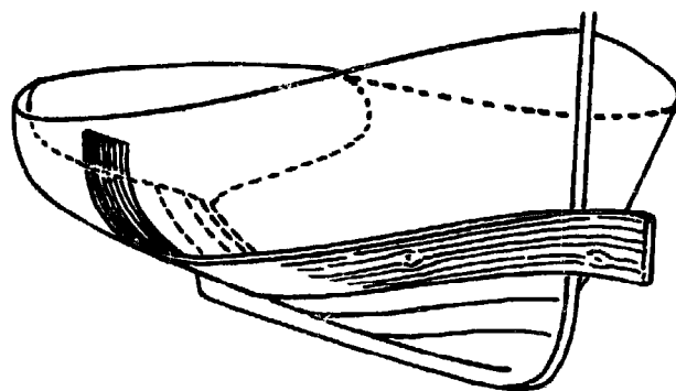
2. Plank shapes. (Left) The shape of a dory is largely governed by the natural bend taken by wide boards of uniform thickness. (Right) In some hull forms, the wood must be twisted, steamed, and tormented into place.
