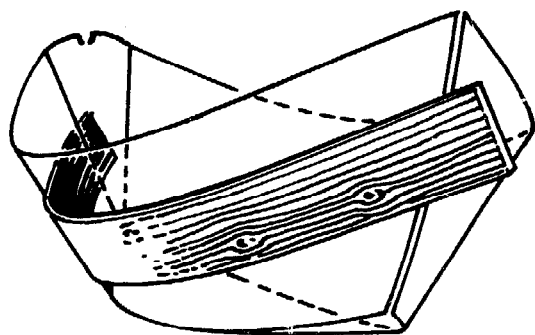
2. Plank shapes. (Left) The shape of a dory is largely governed by the natural bend taken by wide boards of uniform thickness. (Right) In some hull forms, the wood must be twisted, steamed, and tormented into place.
