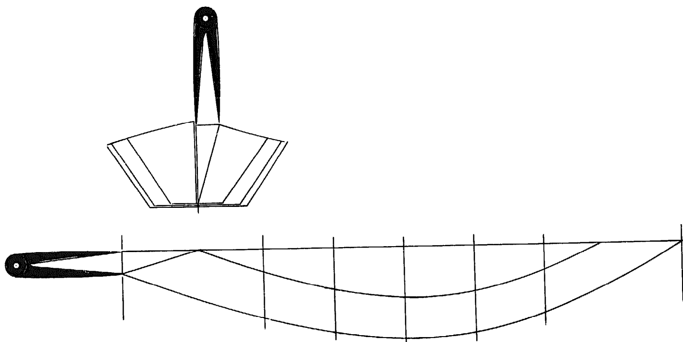
11(c). The width of the transom can be taken from either the halfbreadth or the section plan. Remember that only half the width of the transom is shown. It must be doubled.
