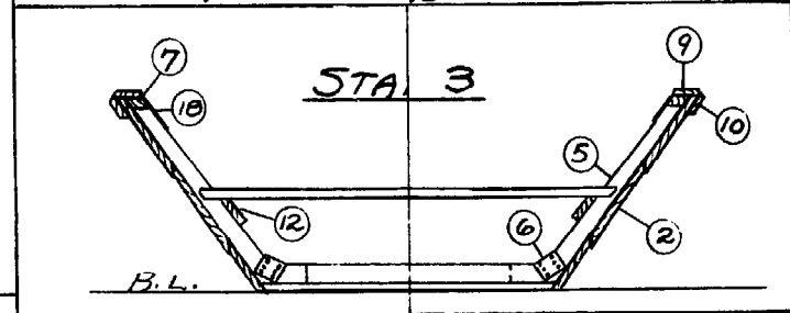
Lines and specifications for the Lowell-Coast Guard 15-foot fisherman's dory. The numbers in the parts list correspond to those in the drawing on page 145.
