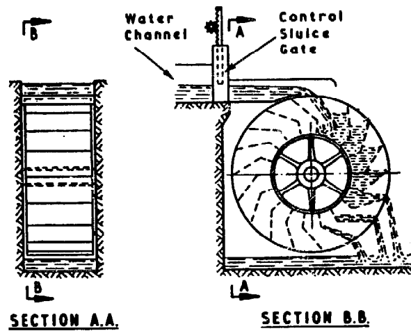
fig. 2 : Overshot wheel.
