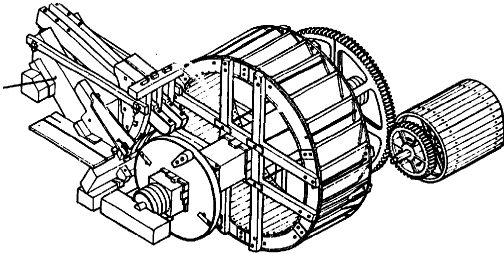
fig. 45: Fulling stocks.
