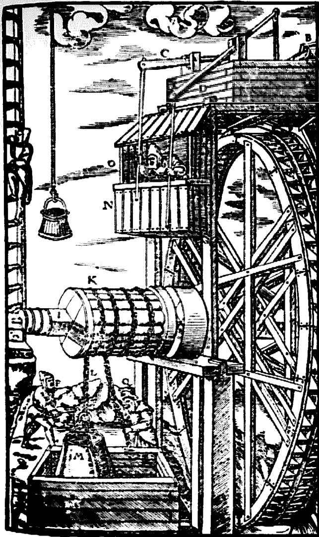
fig. 39: Axle used as a winding drum. A: Reservoir E: Race C, D: Levers I, J: Troughs under the water gates G, H: Double rows of buckets L: Axle K: Larger drum L: Drawing-chain M: Bag N: Hanging cage
