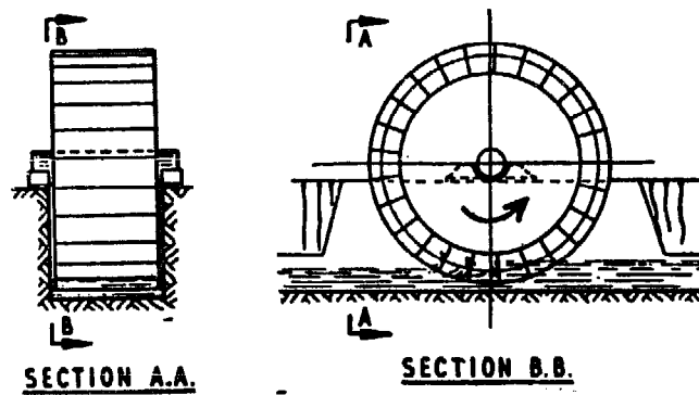
fig. 3 : Undershot wheel.
