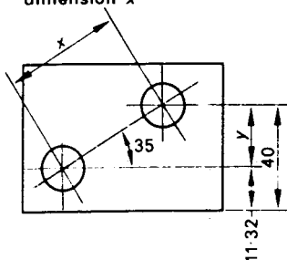
Fig 3.15 Use of trigonometry - sines
