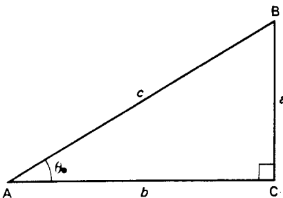
Fig.3.10 The trigonometrical ratios
