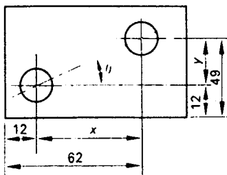
Fig 3.14 Use of trigonometry - tangents
