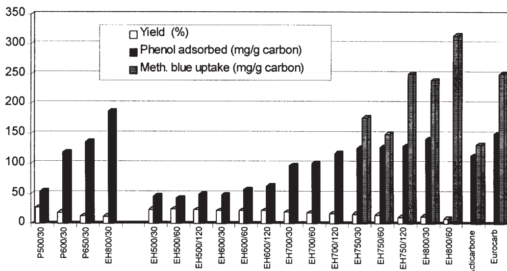
Figure 2. Yield and comparative adsorption properties of activated carbons. (Note that the first group of four values are derived from 0.2g samples of carbon and the rest from 0.5g samples)
