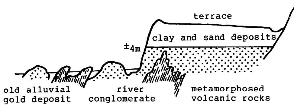
Fig. 6 River conglomerate forming a terrace as part of an old gold deposit (According to Brinck, 1955)
