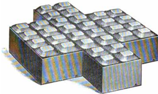
Fig. 149.—Vitrified Blue Paving Brick. 9 inches \times 4½ inches \times 3 inches deep (8 panels).
