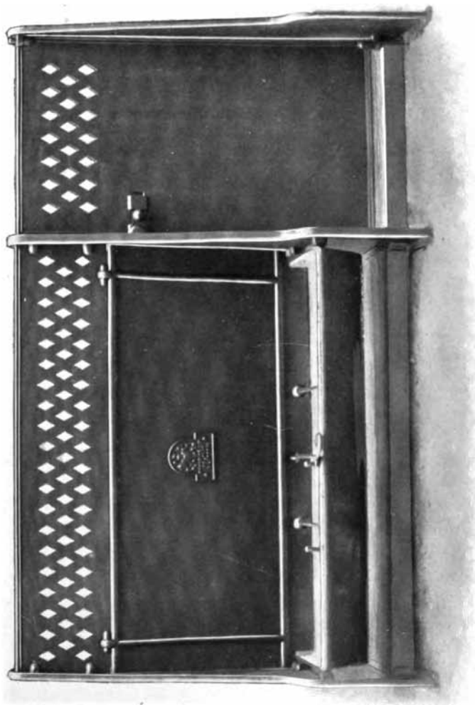
Fig. 141.—Iron Fittings for Piggeries (Musgrave). In the figure the swing flap over the trough is pushed back, thus cutting it off from the sty.
