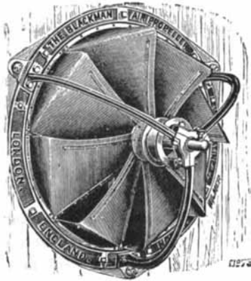
Fig. 25.—Blackman Air-Propeller.
