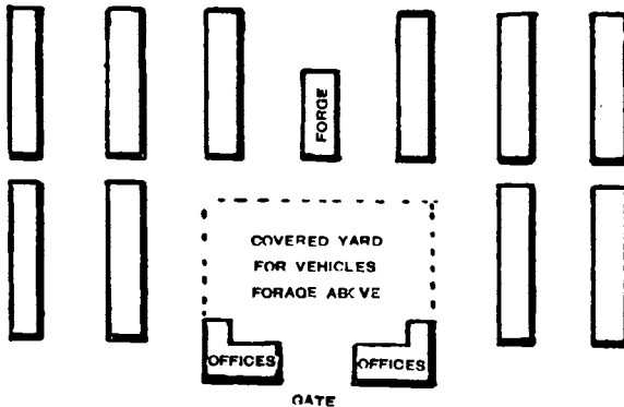
Fig. 120.—Pavilion system of stables for 480 horses.
