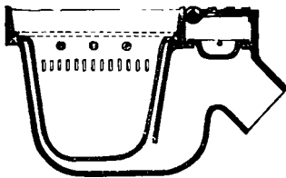
Fig. 165.—Fixed Syphon Trap for Stables, with removable bucket for catching solids.
