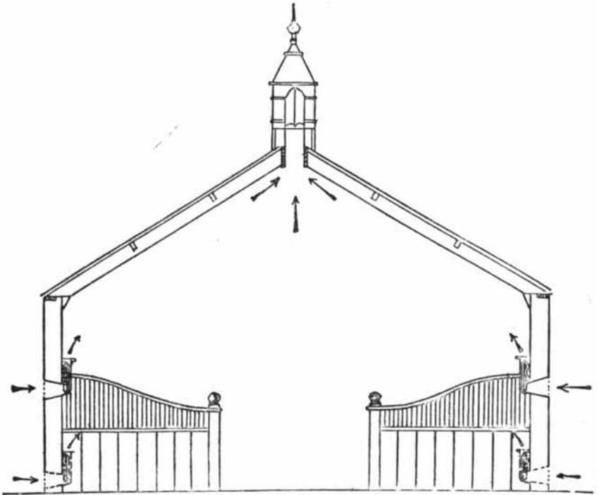
Fig. 3.—Section of a stable heated artificially by means of Boyle's gas-bracket. On the ridge may be seen the exhaust 'air-pump' of the same firm.
