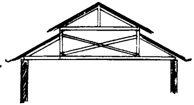
Fig. 85.—Open Roof.
