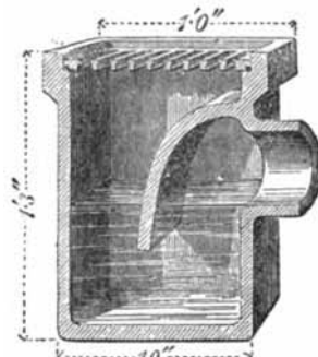
Fig. 166.—A Gully Trap.
