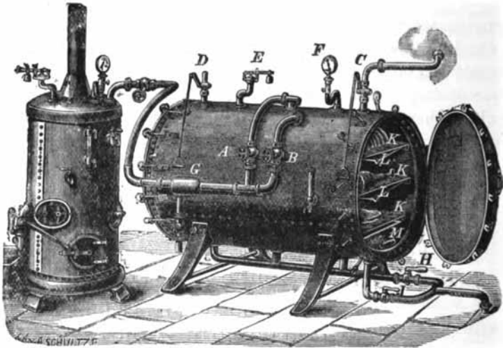
Fig. 194.—The Becker-Ullman Cooking or Destroying Apparatus.*
