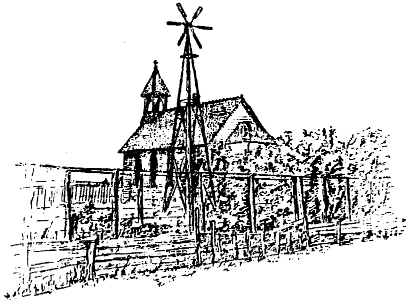
FIG. 73. The reconstructed Aermotor—a veritable toy—which cost nothing yet pumped water for the house, four head of horses, lawn, garden, and small fruit. By measurement it pumped, in a 15½-mile wind, 270 gallons in an hour, or at the rate of 6480 gallons in twenty-four hours; that is $1 worth of water in a day according to the rate of .0015 cents a gallon, as charged in Lincoln. Wheel eight feet in diameter. Depth of well twelve feet. Property of A. C. Walker, civil engineer.
