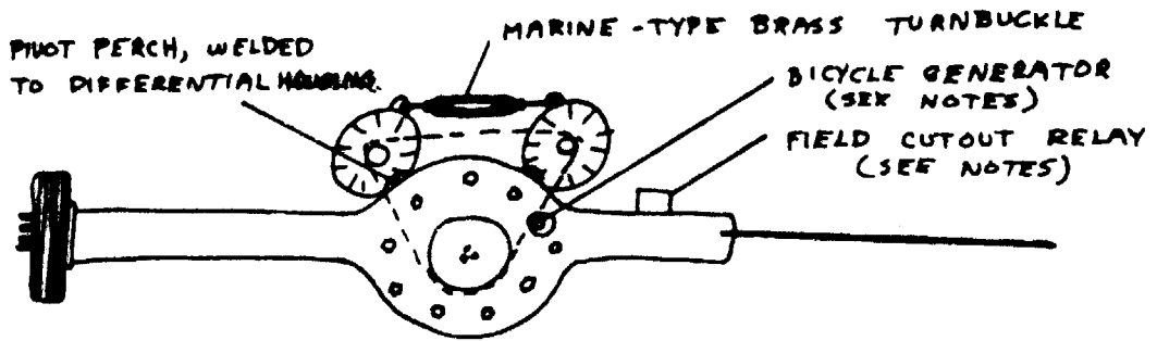
TOP VIEW 2 ALTERNATOR UNIT
