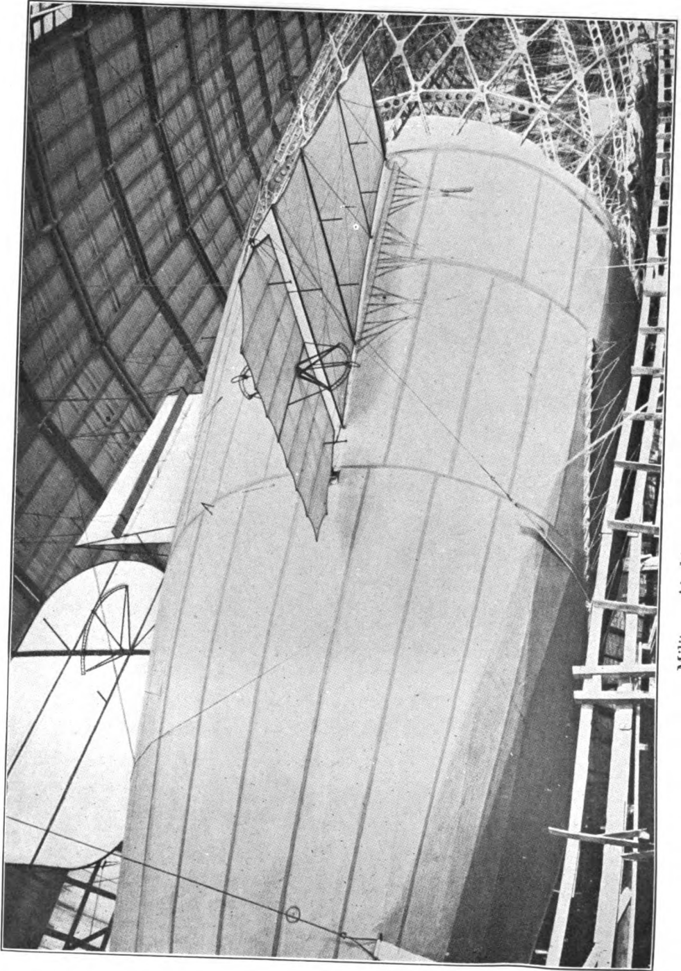
Military Airship in Process of Construction
