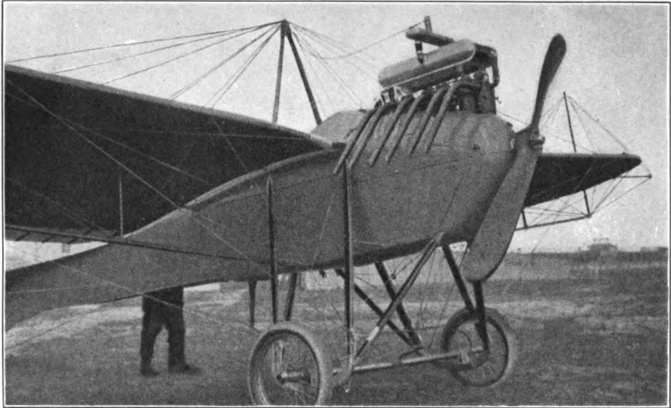
Albatross-Taube Model 1914
