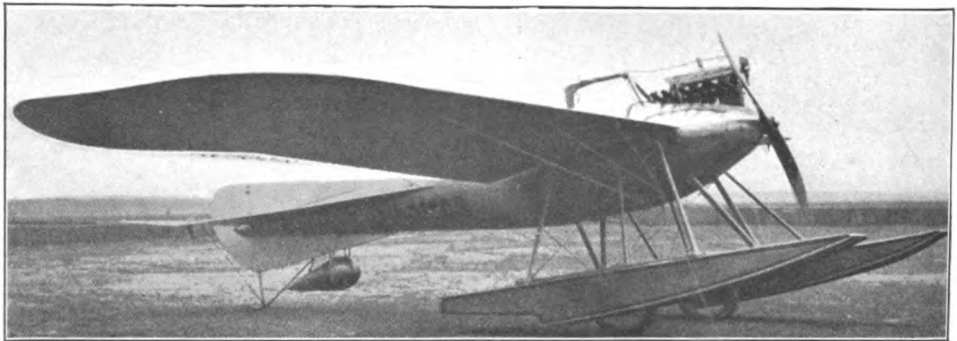
Combination Hydro and Aeroplane
