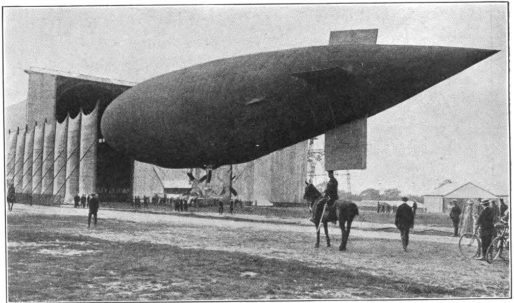
Airship Parseval
