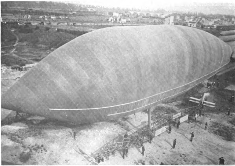
THE FIRST TRIAL OF "VILLE DE PARIS"
