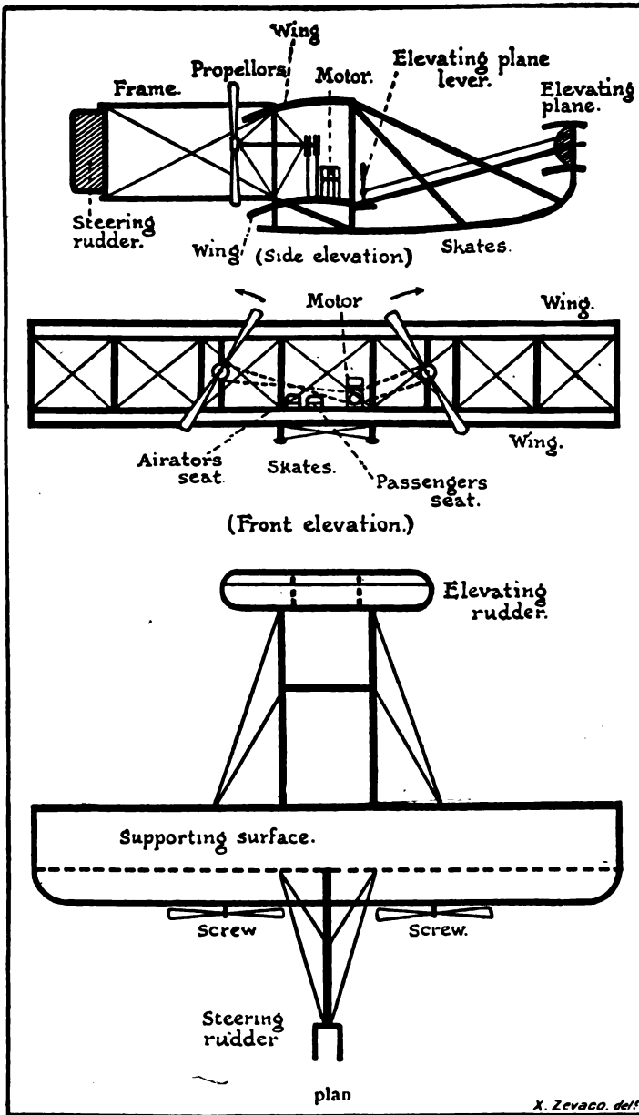
DIAGRAM OF THE WRIGHT BROTHERS AEROPLANE.
