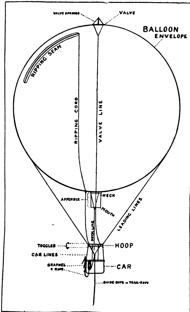
DIAGRAM SHOWING ESSENTIAL PARTS OF A BALLOON.
