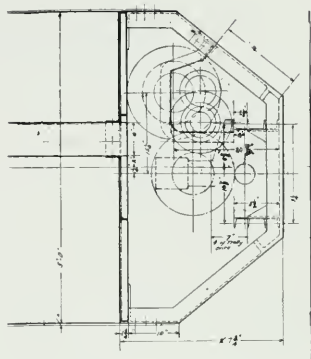
END VIEW SHOWING GEARING OFFICE OF ENGRS. H. YOUNG STEELTON CALIF.
