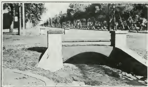
A 46-inch by 12-inch part circle corrugated iron culvert, 14 gauge, installed by city of Ontario
