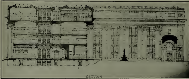
Section, San Francisco City Hall
