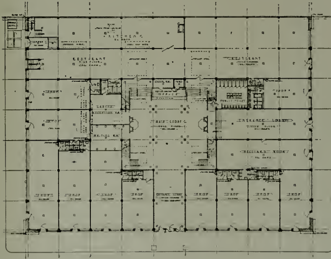
Ground Floor Plan, Workingmen's Hotel, San Diego
