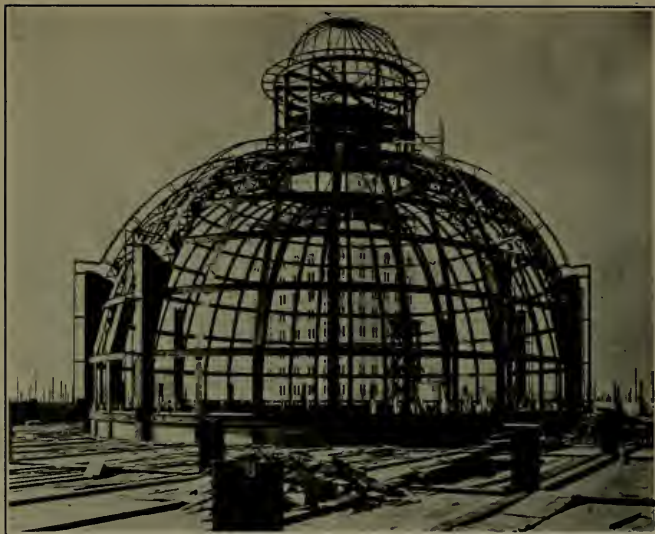
Structural Steel Dome, Kahn Department Store Building, Oakland, California Dyer Bros., Fabricators and Erectors
