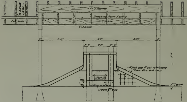
Elevation Looking from Inside of Tank
