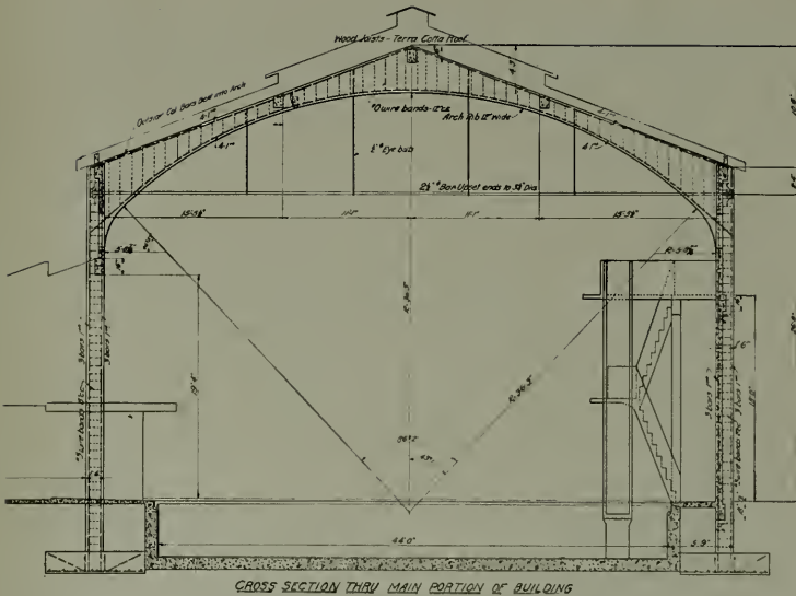
Fig. 7. Municipal Natatorium, San Jose, California
