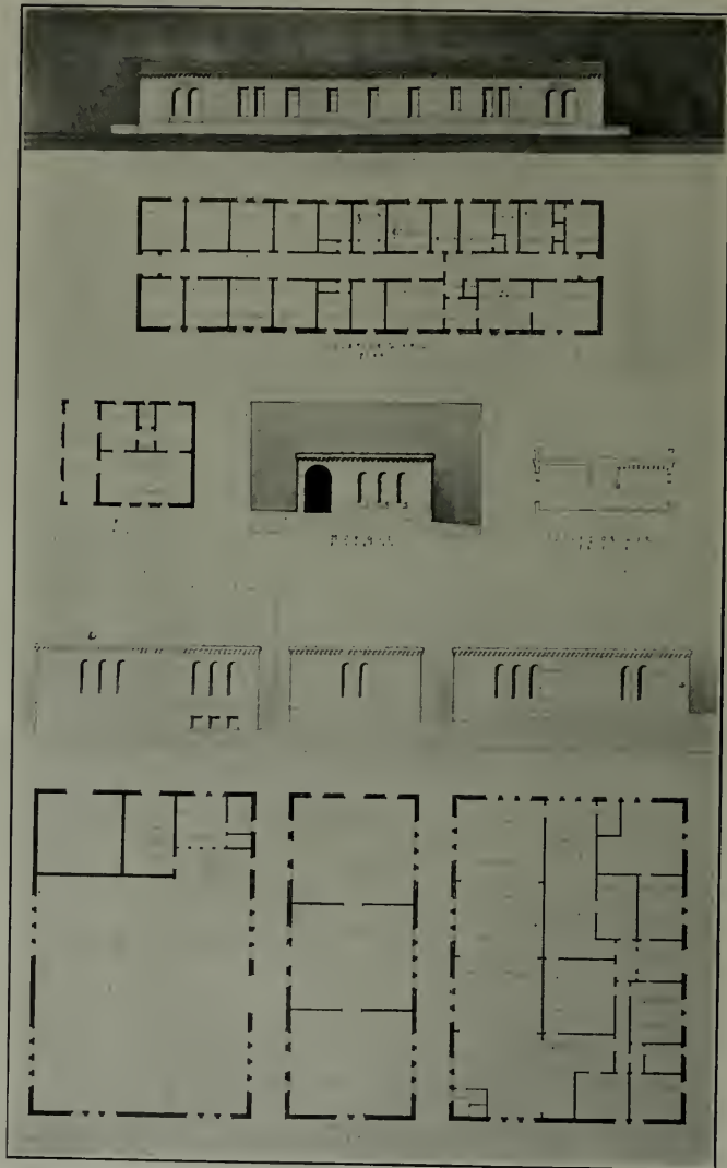
Isolation Ward, Alameda County Hospital Group Charles Peter Weeks, Architect
