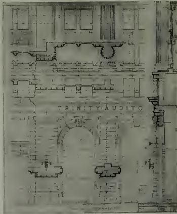
Scale Detail—Trinity Auditorium Building, Los Angeles Fitzhugh, Krucker & Deckbar, Architects
