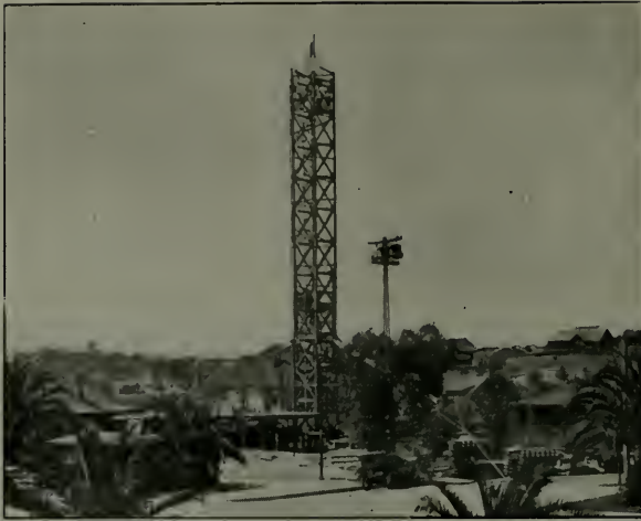
G. Y. Gravity Tower used for Pouring Concrete on all Three Buildings
