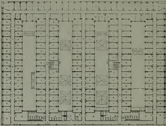
Typical Floor Plan, Workingmen's Hotel, San Diego
