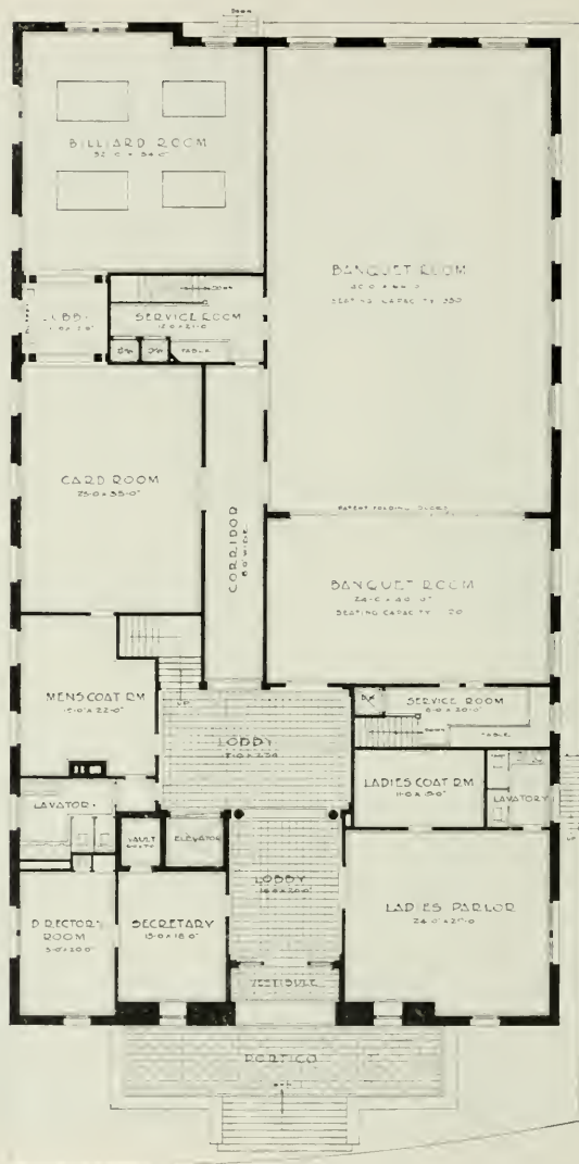
FIRST FLOOR PLAN, BUILDING FOR SCOTTISH RITE BODIES, SACRAMENTO CARL WERNER, ARCHITECT
