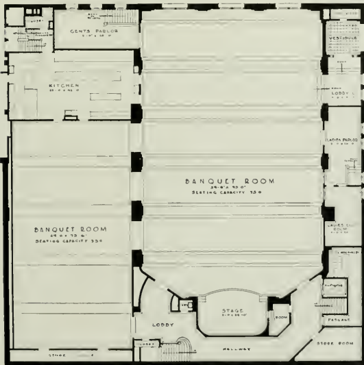
BASEMENT AND SECOND FLOOR PLANS, BUILDING FOR SCOTTISH RITE BODIES, S. IN FRANCISCO O'BRIEN & WERNER, ARCHITECTS
