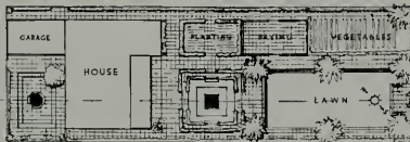
PLOT PLAN SCALE 1/4" = 1'-0"
