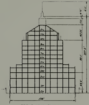
TRANSVERSE SECTION
