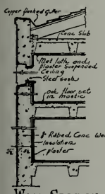
WALL SECTION
