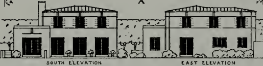
SOUTH ELEVATION
