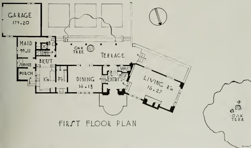
PLANS, HOUSE FOR MR. AND MRS. MICHEL MARCULESCU, HILLSBOROUGH
