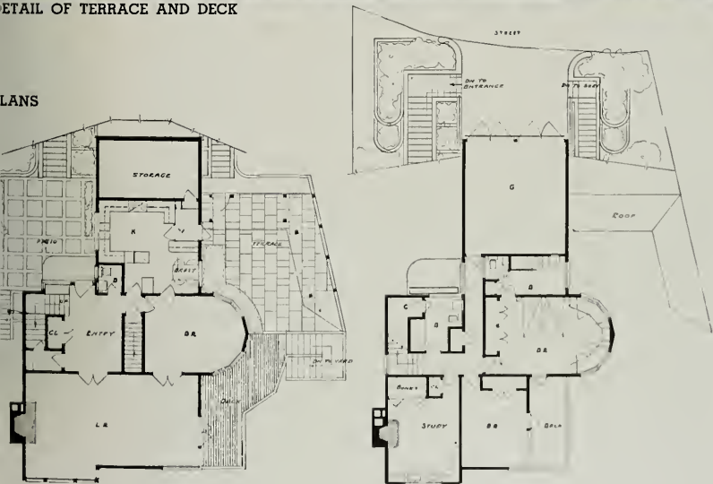
DETAIL OF TERRACE AND DECK
