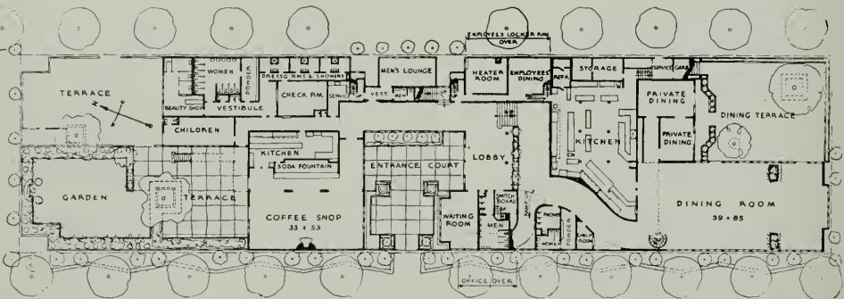
FIRST FLOOR PLAN SCALE IN FEET 0 10 20 30 40
