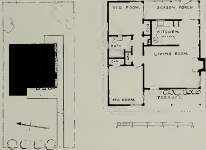
plans
