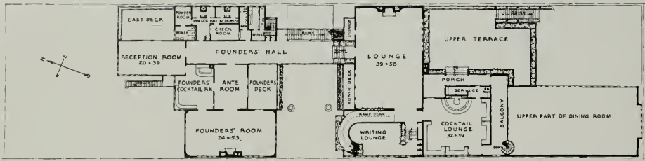
SECOND FLOOR PLAN SCALE IN FEET 0 10 20 30 40
