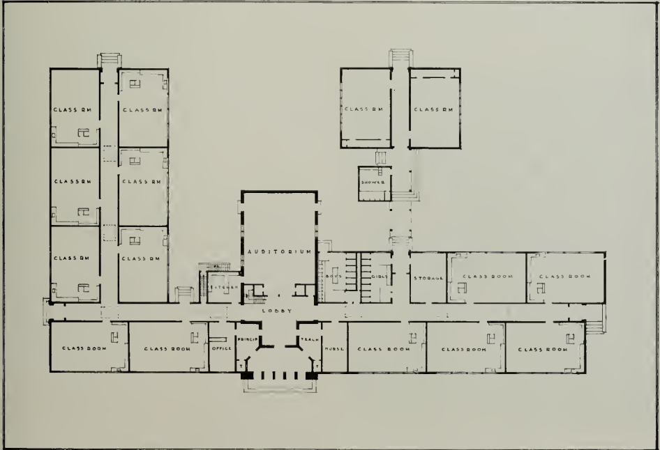
PLAN, DEER VALLEY UNION SCHOOL, BRENTWOOD, CALIFORNIA
