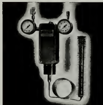
One of the Johnson line of Extended Tube Thermostats. Various types of bulbs adopted to a variety of uses in automatic air conditioning control.
