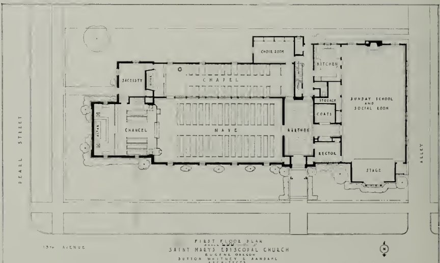
ST. MARY'S EPISCOPAL CHURCH, EUGENE, OREGON
