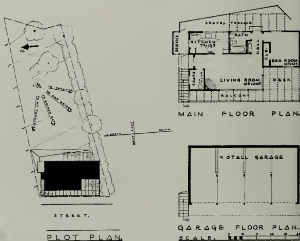
APARTMENT AND GARAGES FOR MISS ELEANOR GARDNER, BERKELEY, CALIF. william wilson wurster, architect
