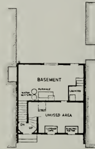
BASEMENT PLAN
