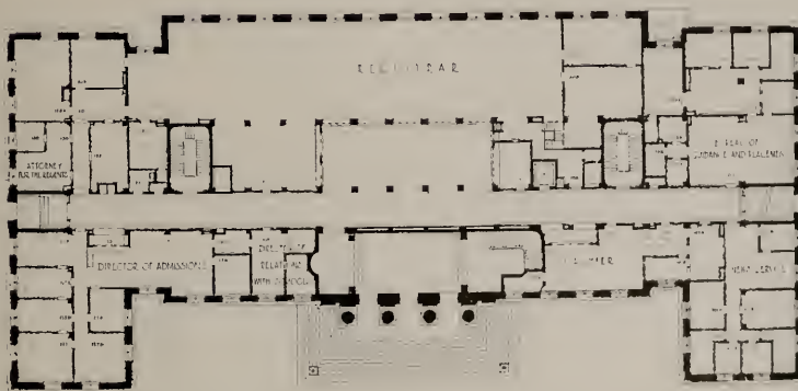
PLANS—FIRST, SECOND AND THIRD FLOORS
