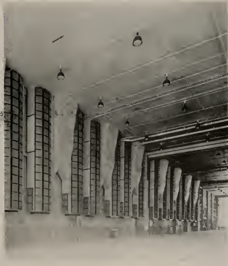
Glass fiber air filters arranged in 912 cells, each cell containing four filters, line the wall through which the washed, warmed and filtered air enters the enclosure
