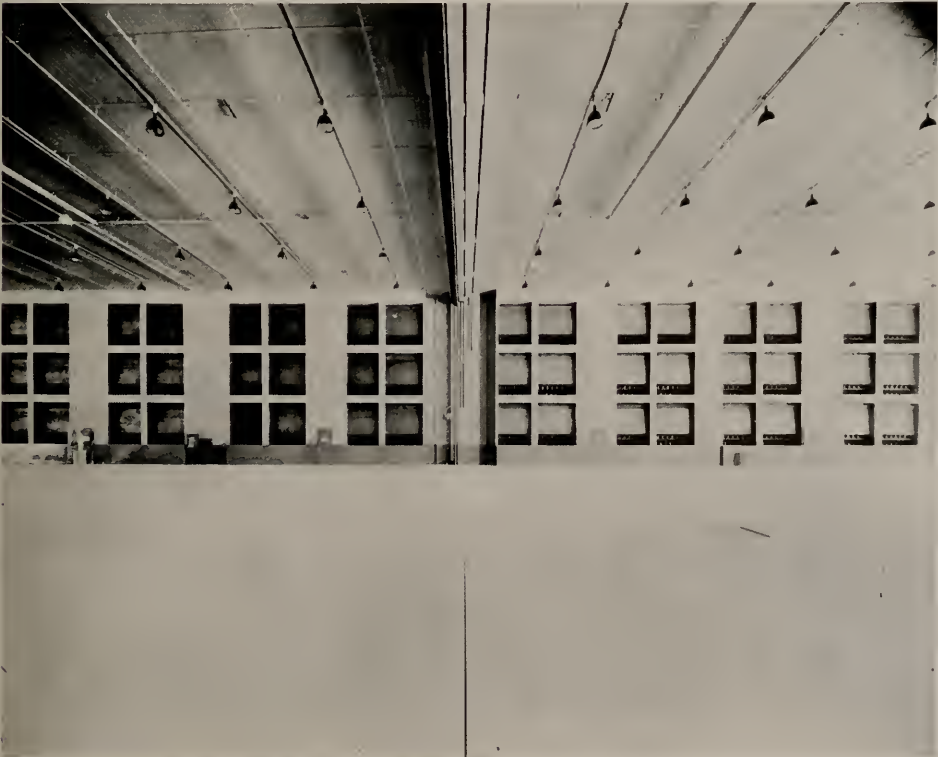
The exhaust units which clean the paint-laden air and discharge it into the outside atmosphere.
