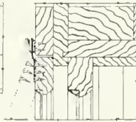
SECTION AT HEAD.
