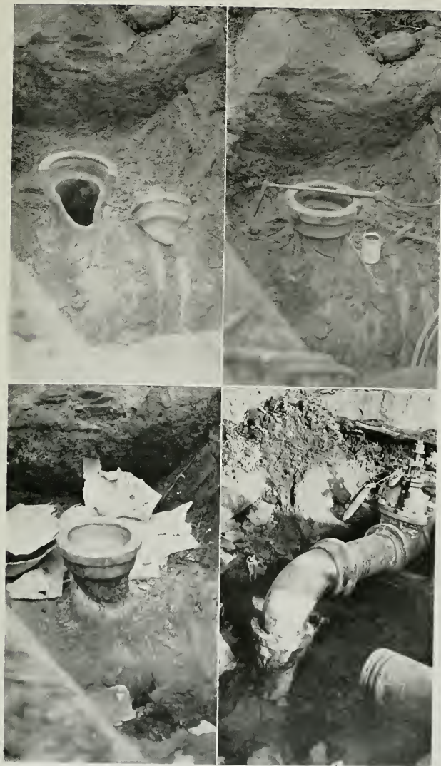
EMERGENCY REPAIR OF A CAST IRON WATER MAIN, LONG BEACH Left to right top of page— Figs. 1 and 2; left to right bottom of page, Figs. 3 and 4. For description see page 111, second column.
