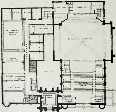
BALCONY FLOOR PLAN, GLENDALE PRESBYTERIAN CHURCH Robert H. Orr, Architect
