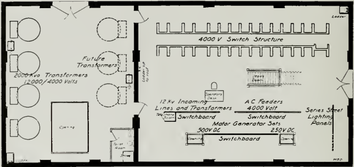
MAIN FLOOR PLAN, SUB-STATION C., SAN DIEGO CONSOLIDATED GAS AND ELECTRIC CO. Requa and Jackson, Architects
