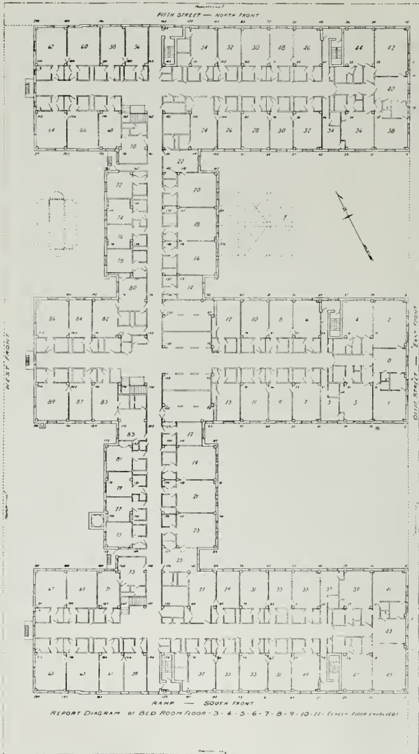
TYPICAL FLOOR PLAN, LOS ANGELES BILTMORE ARCHITECTS SCHULTZE AND WEAVER.
