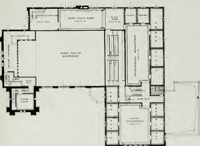
BALCONY FLOOR PLAN, FIRST BAPTIST CHURCH, SAWTELLE Robert H. Orr, Architect
