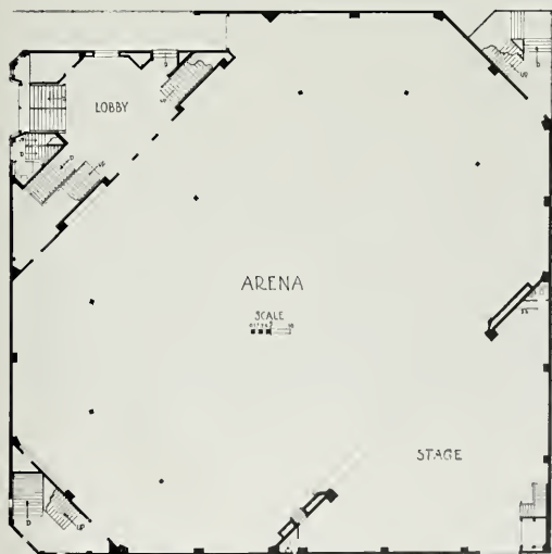
ARENA FLOOR PLAN, CLUB HOUSE AND ARENA FOR GOLDEN GATE POST NO. 10, AMERICAN LEGION, SAN FRANCISCO Morrow & Garren, Architects. (See frontispiece)
