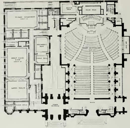
FIRST FLOOR PLAN, GLENDALE PRESBYTERIAN CHURCH Robert H. Orr, Architect
