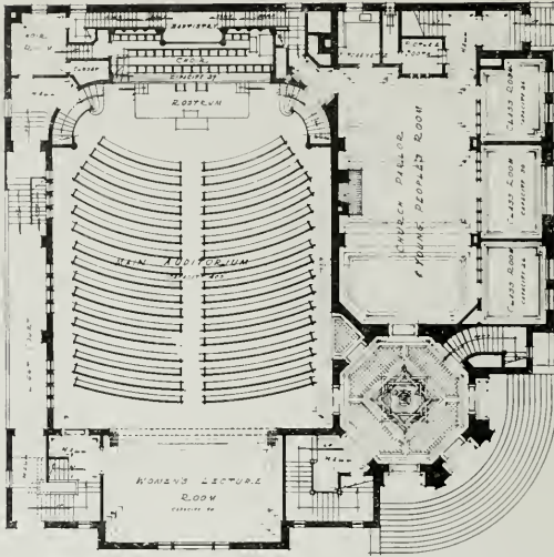
FIRST FLOOR PLAN, FIRST CHRISTIAN CHURCH, STOCKTON Robert H. Orr, Architect
