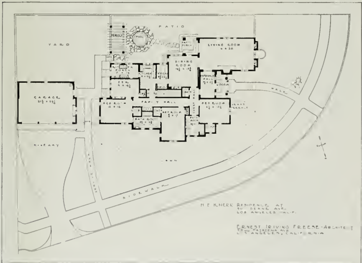
PLAN, BUNGALOW FOR MR. H. E. KNERR, LOS ANGELES Ernest Irving Freese, Architect
