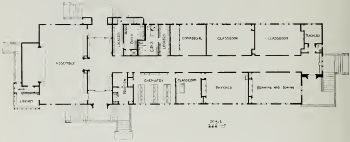
PLAN, CLEAR LAKE UNION HIGH SCHOOL, LAKEPORT, CALIFORNIA Morrow & Garren, Architects. (See page 57)
