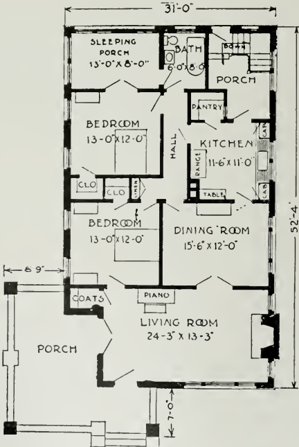
PLAN, BRICK BUNGALOW
