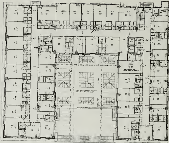
THIRD FLOOR PLAN, THE CALIFORNIAN HOTEL, FRESNO H. Rafael Lake and R. F. Felchin and Co., Architects
