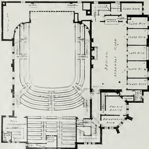
BALCONY FLOOR PLAN, FIRST CHRISTIAN CHURCH, STOCKTON Robert H. Orr, Architect
