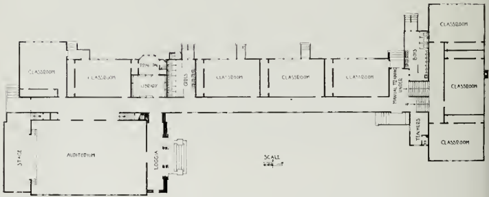
PLAN, LAKEPORT UNION SCHOOL, LAKEPORT, CALIFORNIA Morrow & Garren, Architects. (See page 56)
