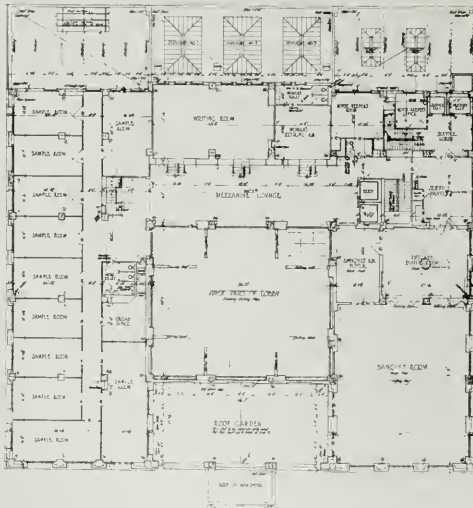
SECOND FLOOR PLAN, THE CALIFORNIAN HOTEL, FRESNO H. Rafael Lake and R. F. Felchin and Co., Architects
