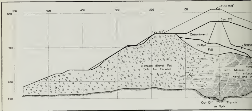
CROSS-SECTION OF CALAVERAS DAM, ONE OUTLINE SHOWING THE DAM AS NOW DAM WHEN FUTURE CONSTRUCTION WILL CARRY
