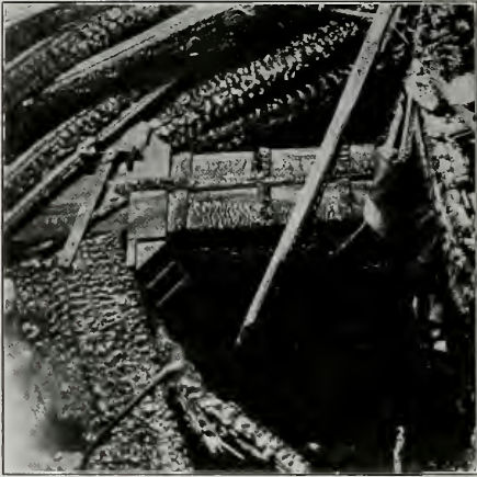
NOTE: TIMBER COLUMNS REMAIN INTACT THUS MAINTAINING STRUCTURAL INTEGRITY OF FRAME OF THE BUILDING
