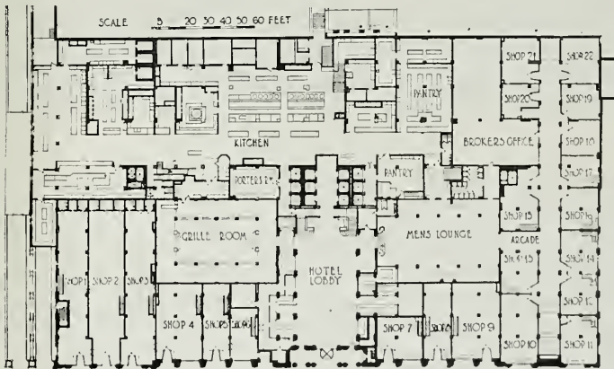
GROUND FLOOR PLAN, LOS ANGELES BILTMORE Schultze and Weaver, Architects
