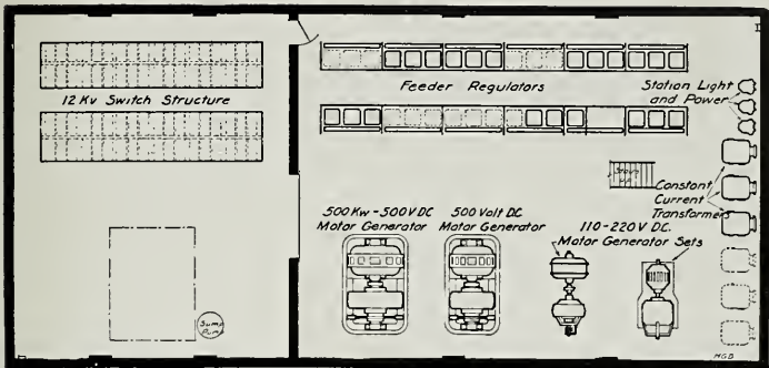
PLAN OF BASEMENT, SUB-STATION C., SAN DIEGO CONSOLIDATED GAS AND ELECTRIC CO. Requa and Jackson, Architects
