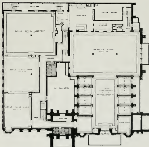
BASEMENT PLAN, GLENDALE PRESBYTERIAN CHURCH Robert H. Orr, Architect
