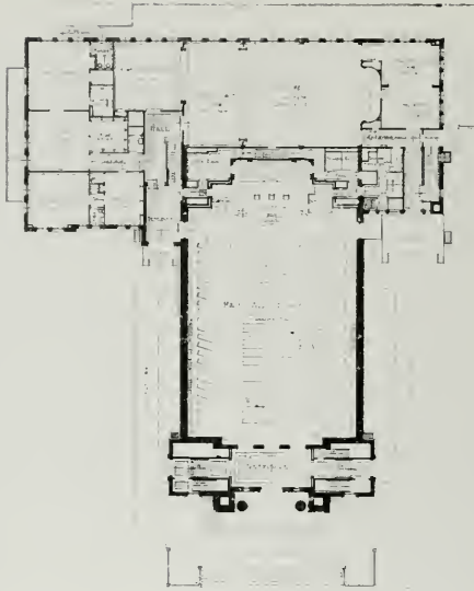
FIRST FLOOR PLAN, HOLLYWOOD CHRISTIAN CHURCH Robert H. Orr, Architect
