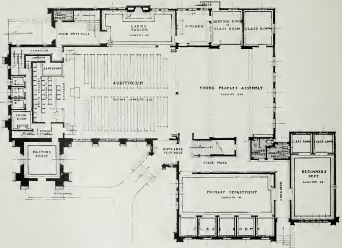
FIRST FLOOR PLAN, FIRST BAPTIST CHURCH, SAWTELLE Robert H. Orr, Architect
