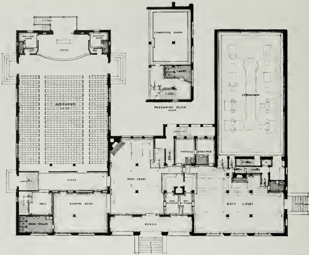
MAIN FLOOR, POMONA Y. M. C. A. BUILDING Robert H. Orr, Architect
