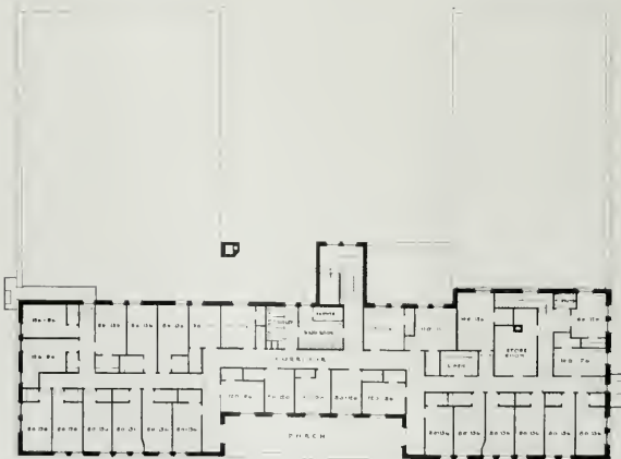
TYPICAL DORMITORY FLOOR PLAN, POMONA Y. M. C. A. BUILDING Robert H. Orr, Architect
