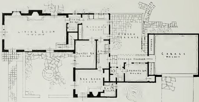
FIRST FLOOR PLAN, HOUSE OF MR. AND MRS. JOHN BYERS, SANTA MONICA John Byers, Architect. (See page 102)
