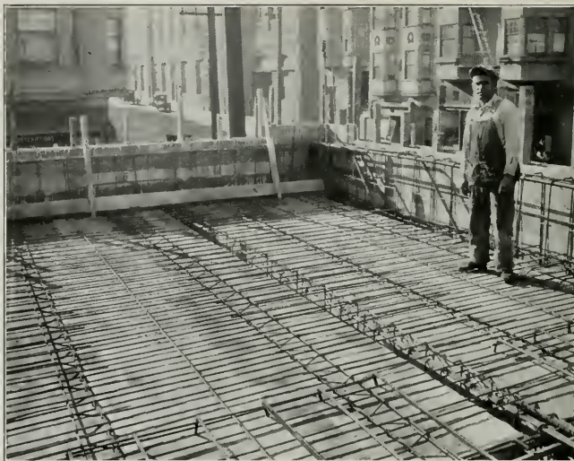
PLACEMENT OF STEEL BAR UNITS, FLOOR OF BUILDING AT JACKSON AND MASON STREETS, SAN FRANCISCO
