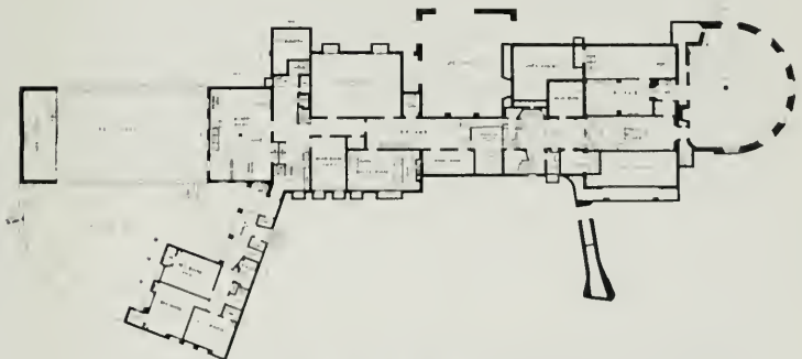
BASEMENT PLAN, HOUSE OF MR. THOMAS H. INCE, BEVERLY HILLS, CALIFORNIA Roy Seldon Price, Architect. (See page 110-114)
