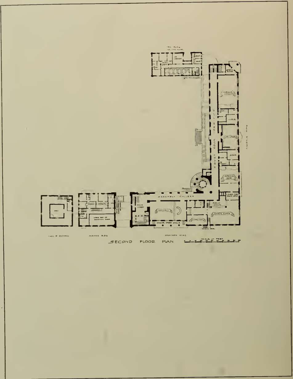
PLAN, SECOND STORY, COURT HOUSE, SANTA BARBARA WILLIAM MOOSER CO., ARCHITECTS
