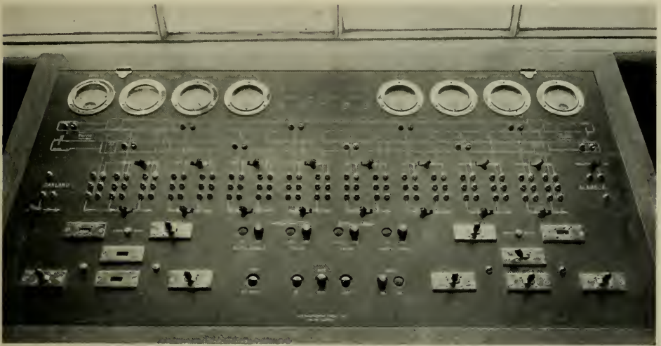
OPERATOR'S INDICATOR BOARD, GEO. A. POSEY TUBE Showing Status of All Signals, Fans and Motors
