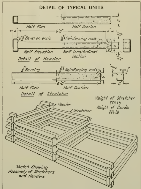
TYPICAL UNITS OF CRIBBING
