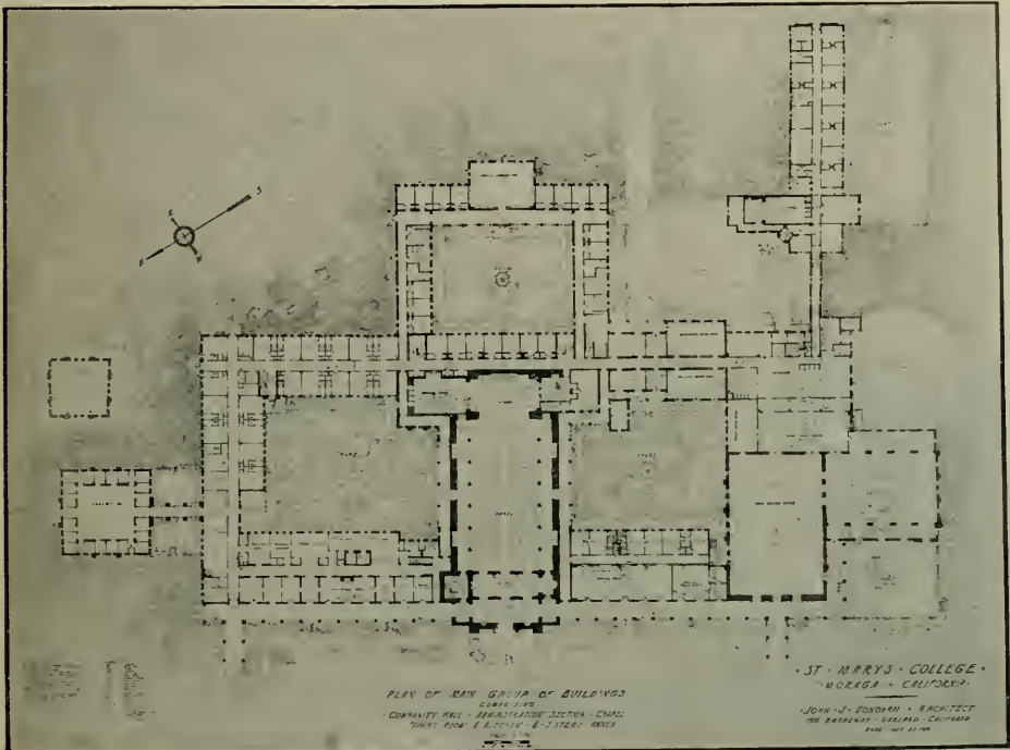
PLAN, MAIN GROUP OF BUILDINGS, ST. MARY'S COLLEGE John J. Donovan, Architect
