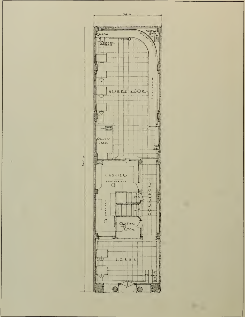
PLAN, BUILDING FOR WILLIAM CAVALIER AND CO., OAKLAND HUGH C. WHITE, ARCHITECT
