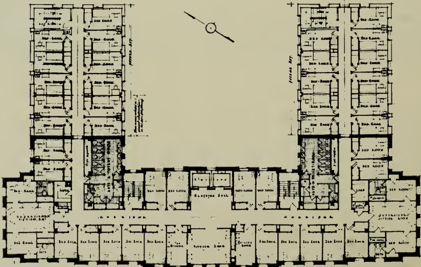
MAIN FLOOR AND TYPICAL PLAN, NURSES' HOME, KING COUNTY HOSPITAL, SEATTLE
