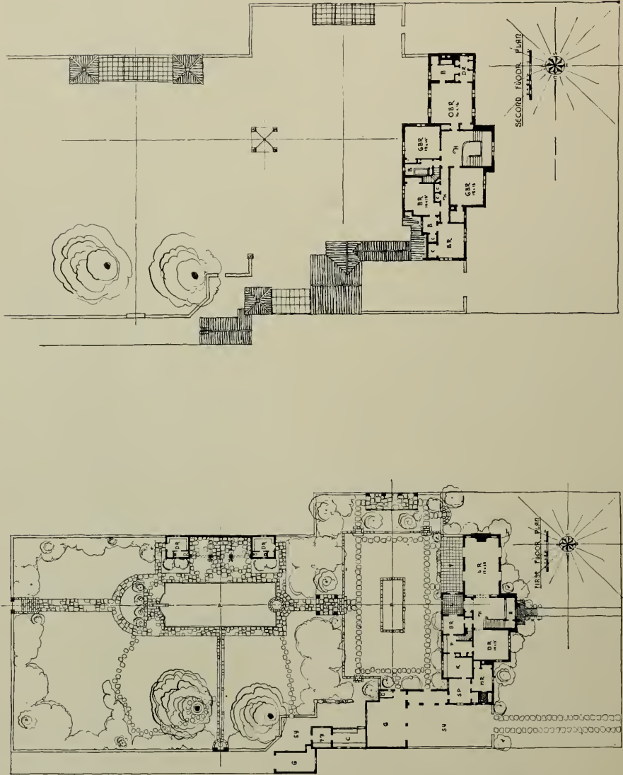
PLANS, HOUSE OF GEORGE G. POLLOCK, SACRAMENTO, CALIFORNIA DEAN AND DEAN, ARCHITECTS
