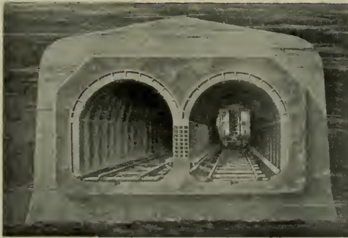
SECTION SHOWING DOUBLE TRACK TUBE TO BE SUNK INTO PLACE AT BOTTOM OF BAY OR RAISED ABOVE THE BOTTOM ON PIERS
