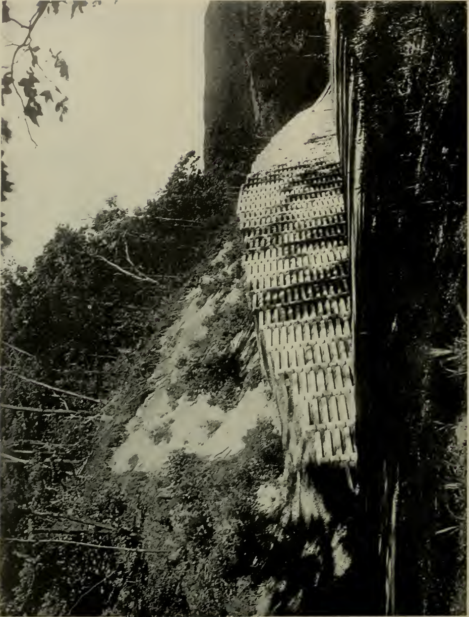
FIG. 2.—CONCRETE CRIBBING, RETAINING STEEP SLOPES ALONG STATE HIGHWAY IN MASSACHUSETTS
