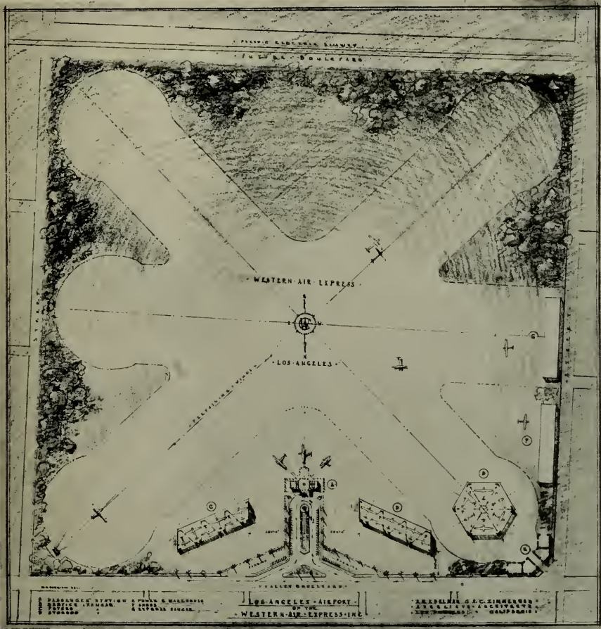
PLOT PLAN FOR LOS ANGELES AIRPORT, LOS ANGELES, CALIFORNIA A. R. Edelman and A. C. Zimmerman, Associate Architects
