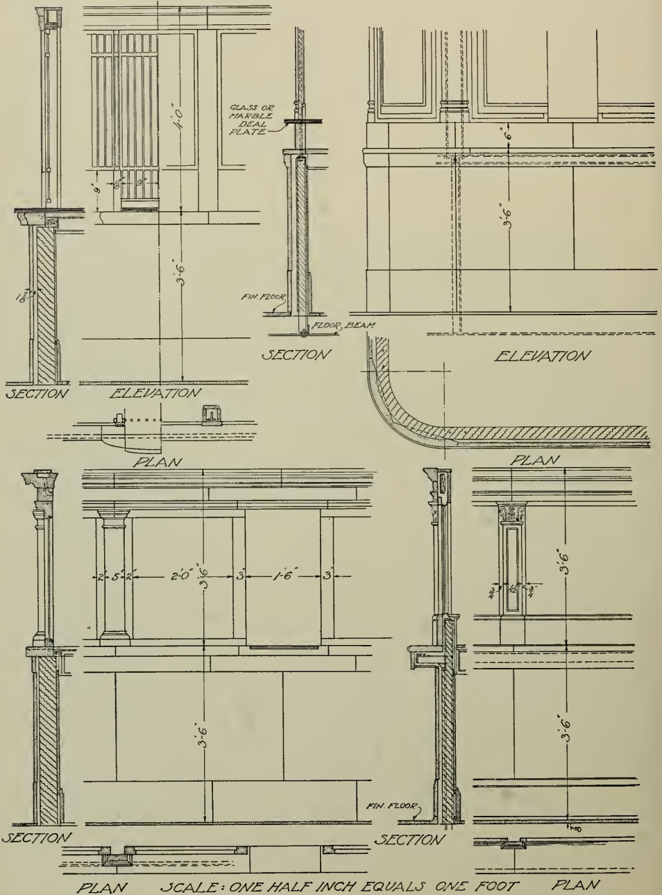
DETAILS FOR MARBLE BANK SCREENS
