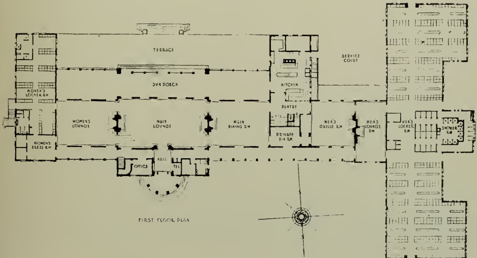
PLAN, CALIFORNIA GOLF CLUB, SAN MATEO COUNTY, CALIFORNIA Willis Polk and Company, Architects
