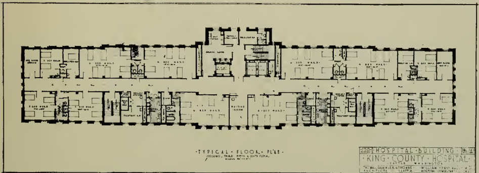
TYPICAL PLAN, KING COUNTY HOSPITAL, SEATTLE, WASHINGTON
