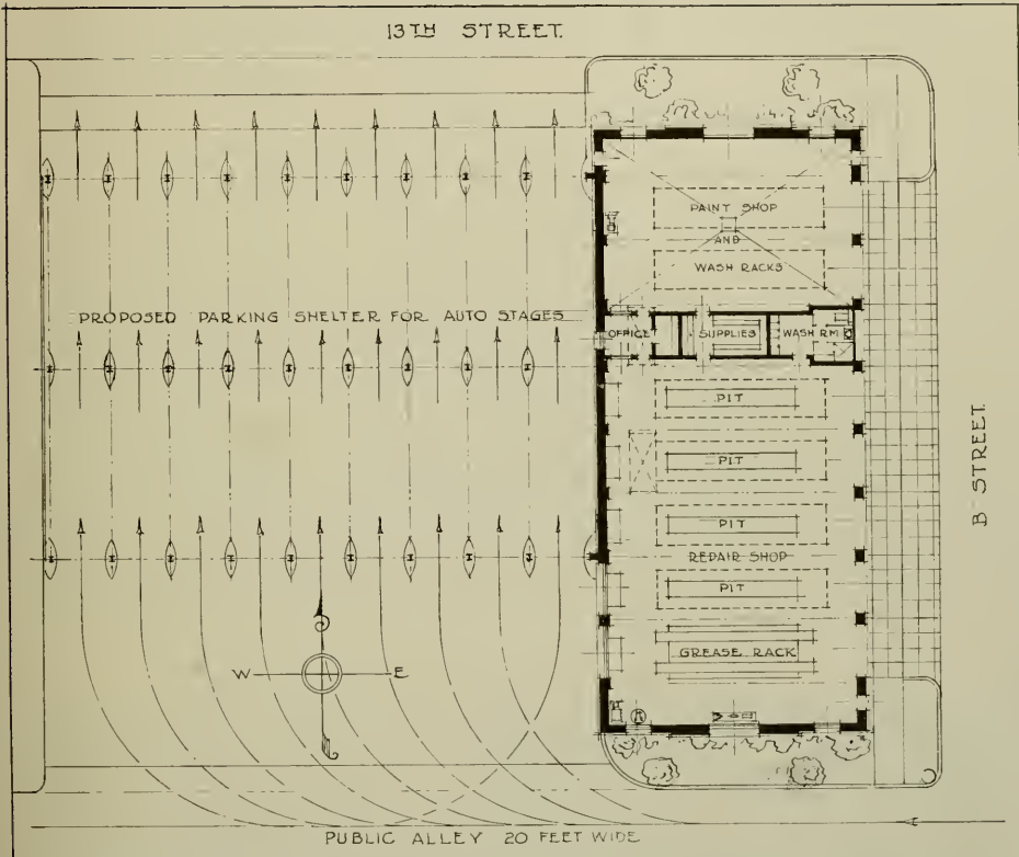
FIRST UNIT OF TRANSPORTATION BUILDING KERN CO UNION H.S. BAKERSFIELD, KERN CO., CALIF. SYMMES & CULLIMORE, ARCHITECTS
