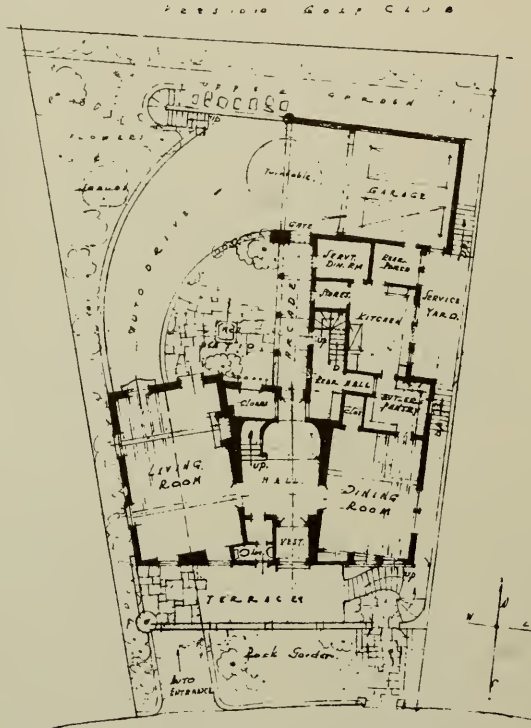
RESIDENCE OF W. H. LOWE, E. J. ALBERT FARR, ARCHITECT J. FRANCIS WARD, ASSOCIATE
