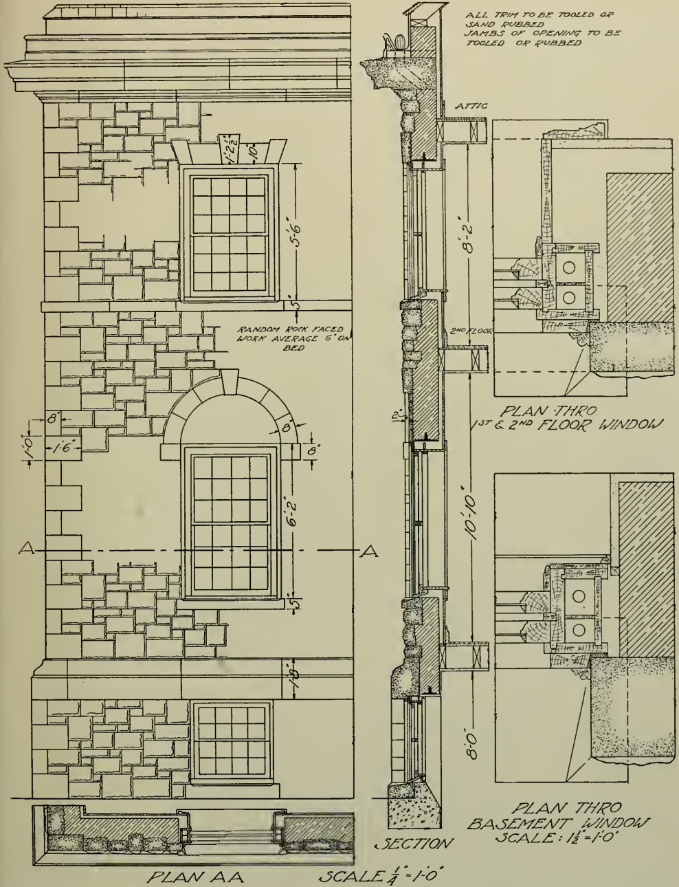
DETAILS, MARBLE EXTERIOR, MAIN OFFICE BUILDING, VERMONT MARBLE CO., PROCTOR, VERMONT R. CLIPSTON STURGIS, ARCHITECT
