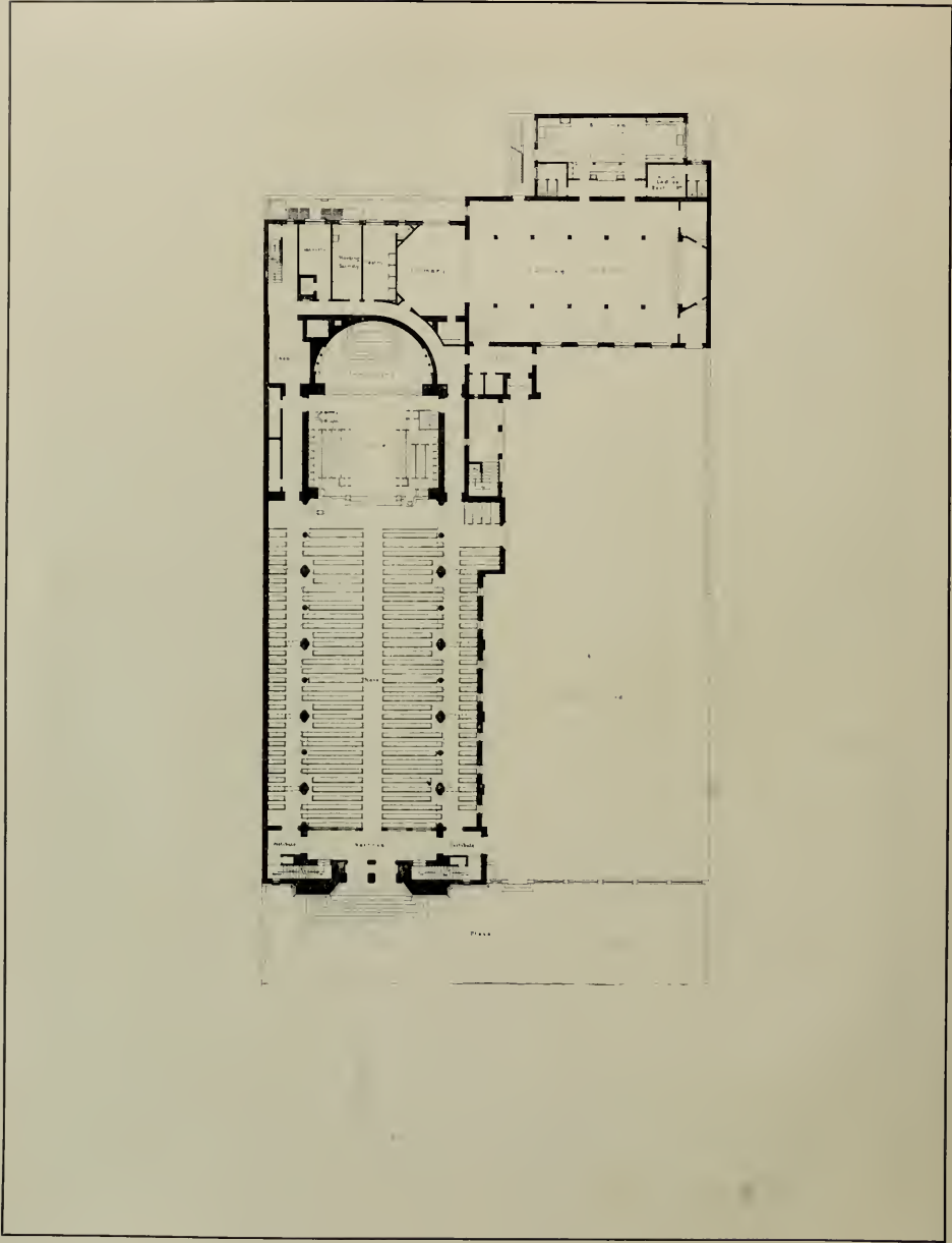
PLAN, SAINT PAUL'S CATHEDRAL, LOS ANGELES JOHNSON, KAUFMANN & COATE, ARCHITECTS
