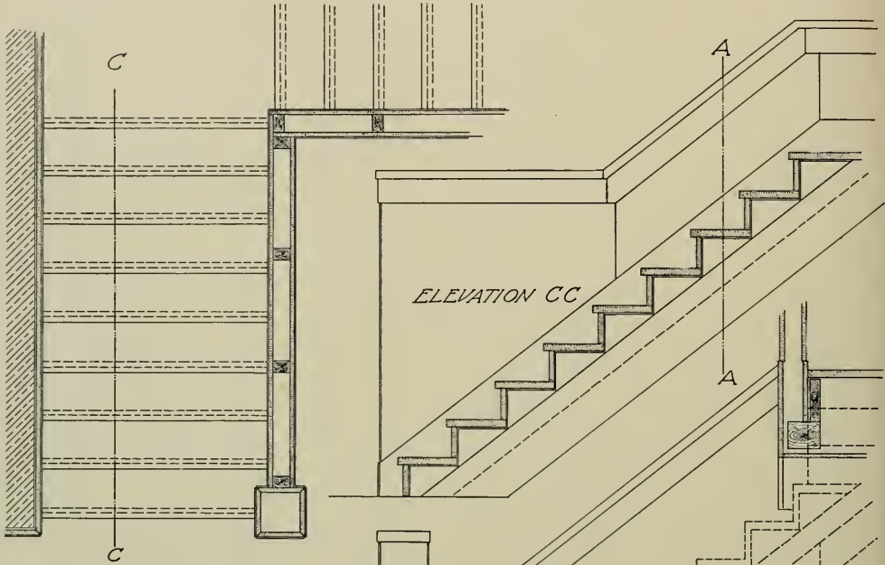
PLAN OF STAIRS
