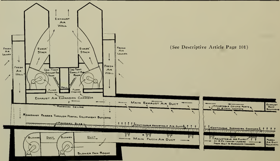
ESTUARY SUBWAY CONTINUOUS TRANSVERSE VENTILATION SYSTEM
