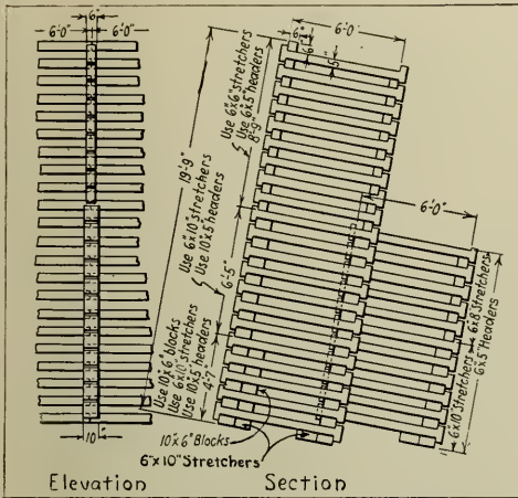
ELEVATION AND SECTION OF CRIBBING
