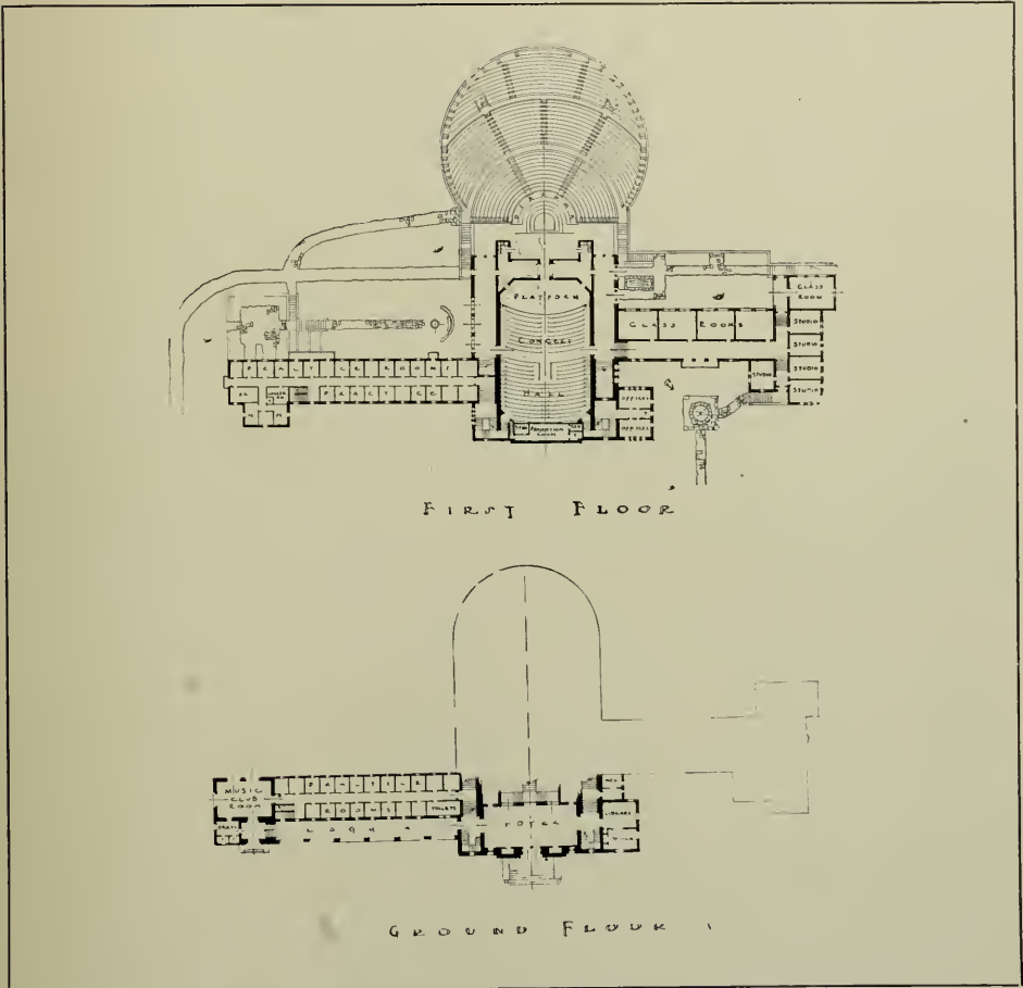
PLANS, MUSIC BUILDING, MILLS COLLEGE, OAKLAND W. H. RATCLIFF, JR., ARCHITECT
