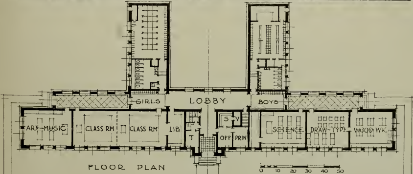
McFARLAND HIGH SCHOOL McFARLAND KERN CO SYMMES & CULLIMORE ARCHITECTS BAKERSFIELD CALIF
