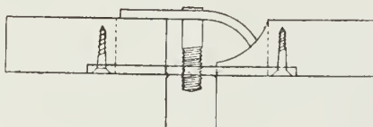
Detail showing Center Stop for Double Doors
