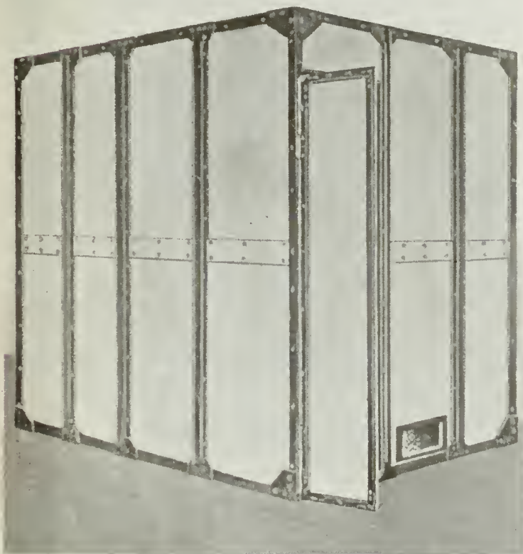
Stationary Fire-proof Moving Picture Booth Constructed of Ambler Asbestos Building Lumber
