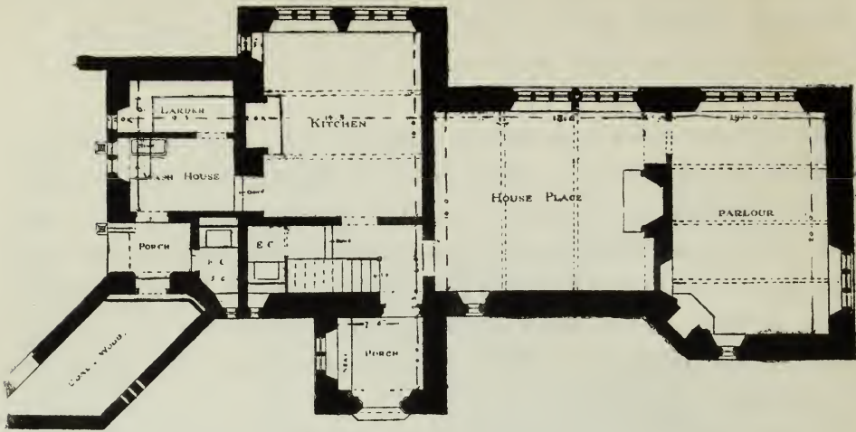
GROUND PLAN
