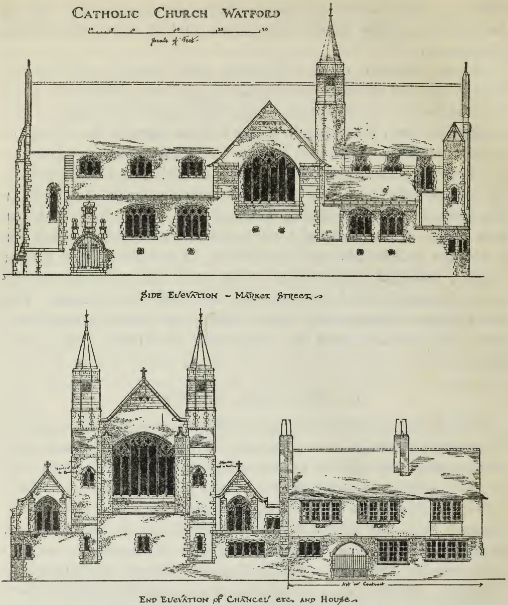
FIG. 38.—CHURCH OF THE HOLY ROD, WATFORD: SOUTH AND EAST ELEVATIONS.
