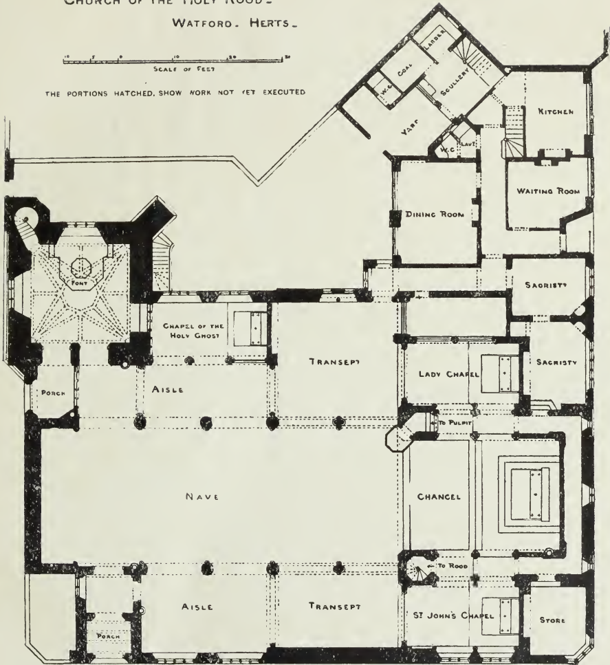
PLATE LIV.—CHURCH OF THE HOLY ROAD, WATFORD: GROUND PLAN (1879).
