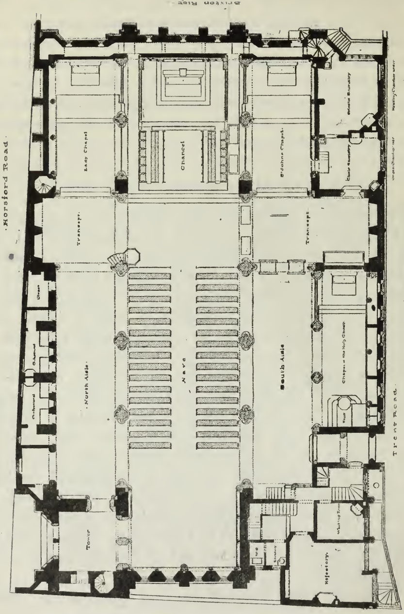
Ground Plan.
