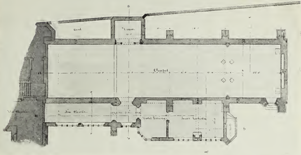
PLATE LXX.—S. THOMAS'S SEMINARY, HAMMERSMITH. A. ORIGINAL GROUND PLAN OF MAIN BUILDING. B. CHAPEL PLAN, SHOWING ADDITIONS TO ORIGINAL CLOISTER.
