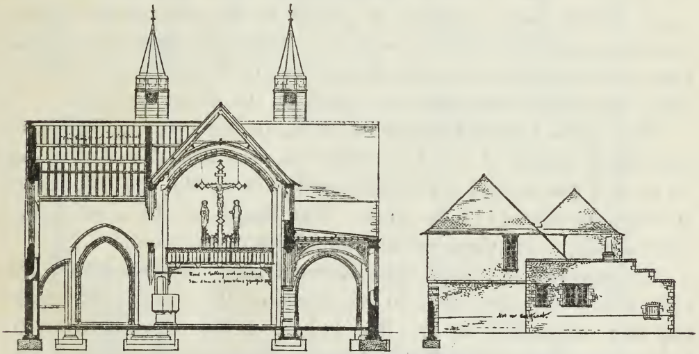
FIG. 39.—CHURCH OF THE HOLY ROAD, WATFORD : (1) LONGITUDINAL SECTION. 2. TRANSVERSE SECTION.
