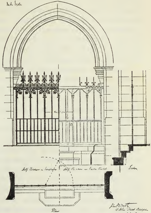
FIG. 43.—PAUL'S HOUSE CONVENT, TAUNTON: SANCTUARY SCREEN.
