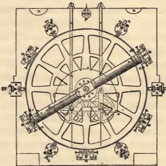
Fig. 21.—Mural Circle.
