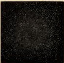
Fig. 77.—Globular Cluster.
