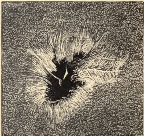
Fig. 36.—Solar Spot, by Langley.
