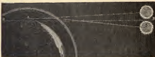
Fig. 12.—Atmospherical Refraction.
