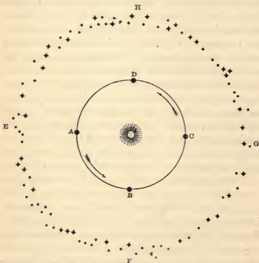
Fig. 42.—Showing the Sun's Movement among the Stars.
