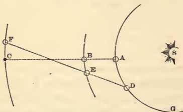
Fig. 47.—Illustrating Movements of a Superior Planet.
