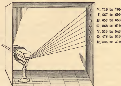
Fig. 6.—White Light resolved into Colors.
