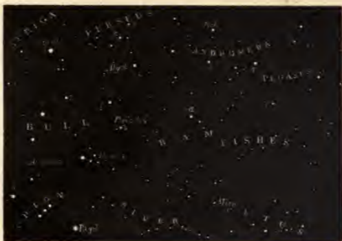
Algora is on the Meridian, 51^\circ South of Pole.—At 10 o'clock, December 7th; 9 o'clock December 22d; 8 o'clock, January 5th.
