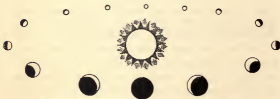
Fig. 53.—Phases of Venus, and Various Apparent Dimensions.
