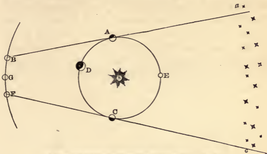
Fig. 46.—Apparent Movements of an Inferior Planet.
