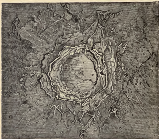
Fig. 60.—Lunar Crater "Copernicus," after Secchi.
