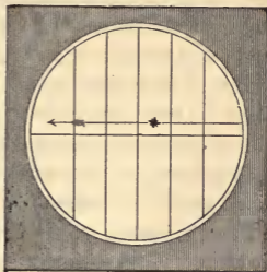
Fig. 23.—Transit of a Star noted.
