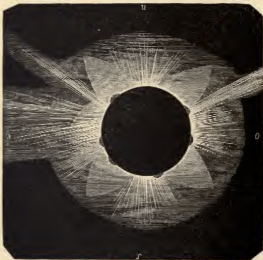
Fig. 32.—The Corona in 1858, Brazil.
