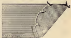
Fig. 59.—Illumination of Craters and Peaks.
