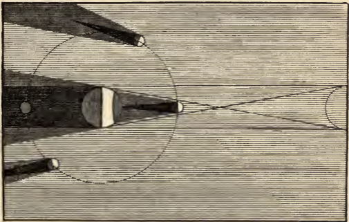
Fig. 61.—Eclipses; Shadows of Earth and Moon.
