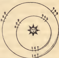
Fig. 3.—Changes of orbit by mutual attraction.
