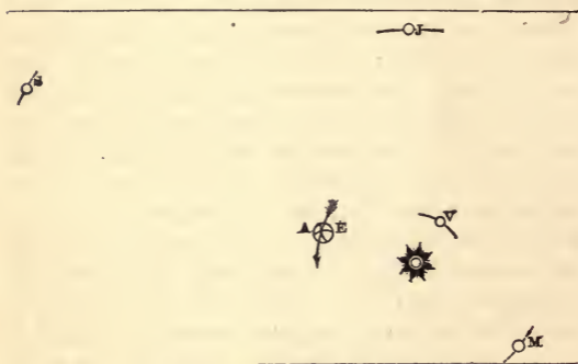
Fig. 45.—Showing Position of Planets.
