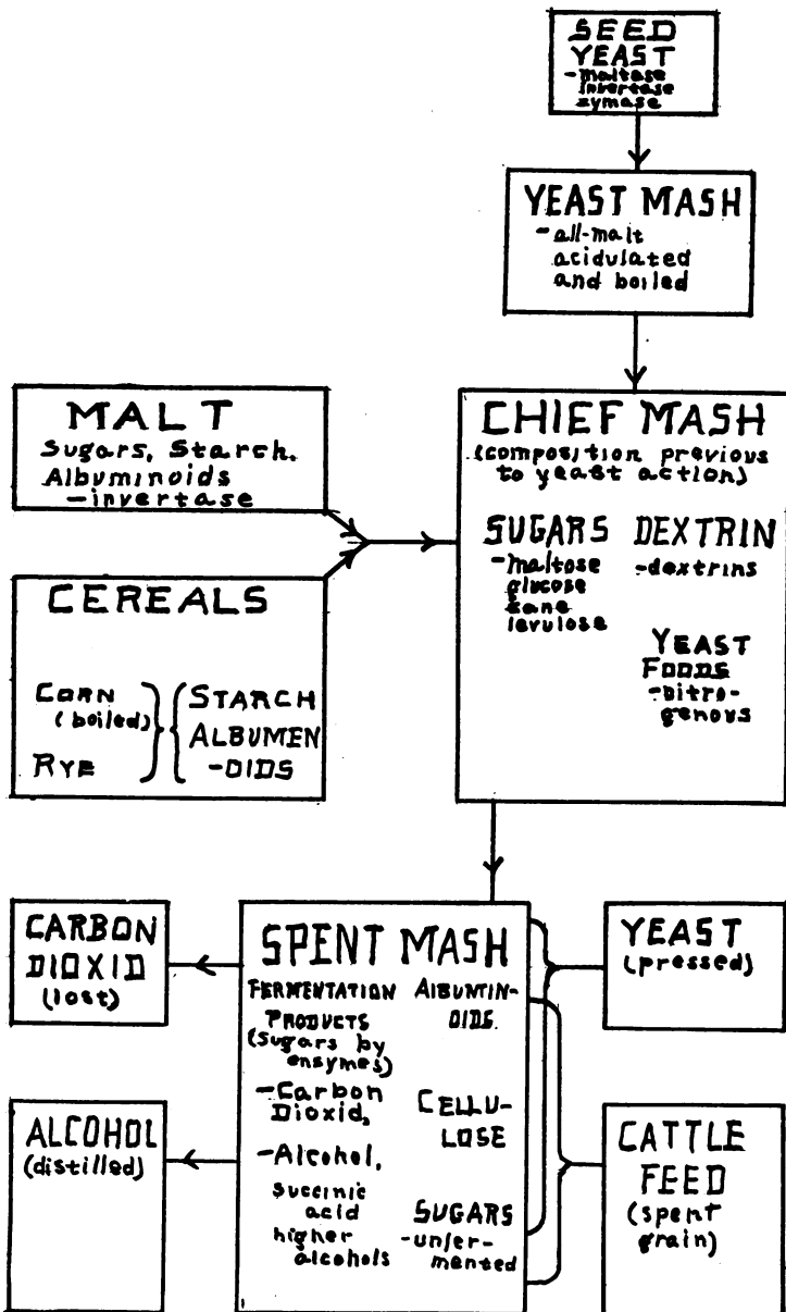
Fig. 4.—Diagram of the mass action in yeast manufacture.
