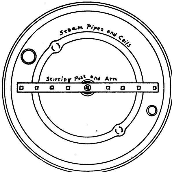
Fig. 7.—Diagram of mash tub.
