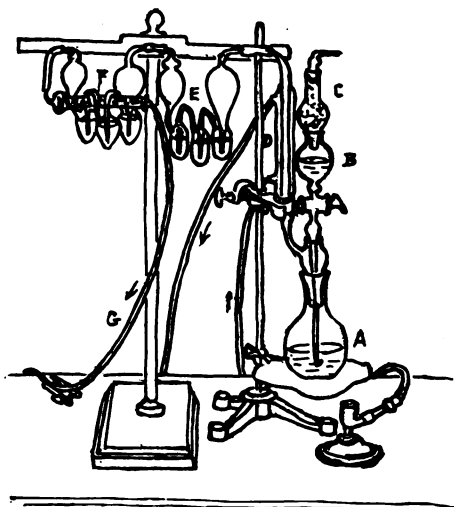
Fig. 11.—Knorr's apparatus for the determination of \text{CO}_2 . A—Distilling flask fitted to condenser by a ground-glass stopper; B—Reservoir containing acid; C—Soda-lime tube fitted to acid reservoir by a ground-glass stopper; D—Condenser; E—Liebig bulb with a solution of KOH for the absorption of \text{CO}_2 and followed by a CaCl tube. An additional guard tube filled with soda lime should follow the tube F, though not shown in the cut. From U. S. D. A., Bur. of Chem., Bull. 107.
