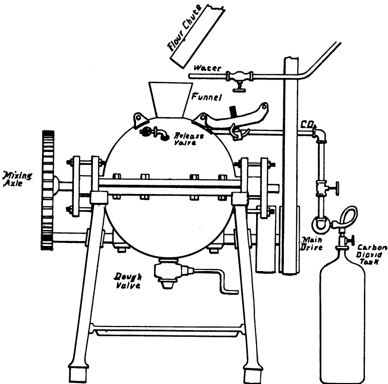
Fig. 12.—Aerated bread machine. (Courtesy Meek-Barnes Baking Co., Los Angeles.)
