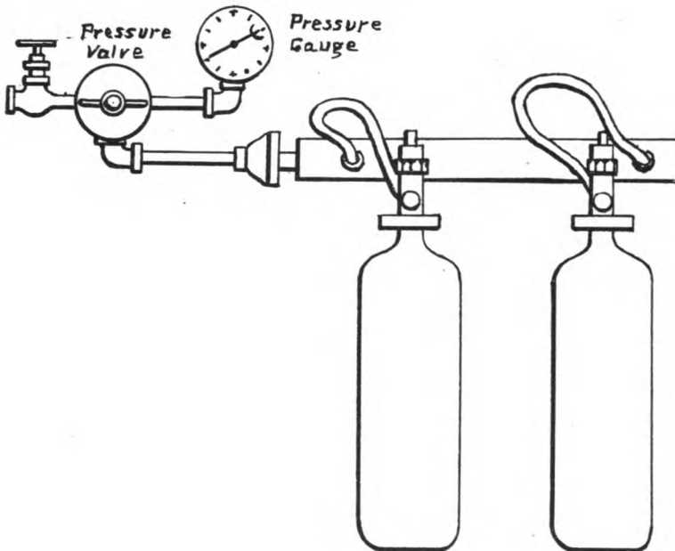
Fig. 13.—Carbon dioxide attachment for aerated bread apparatus.
