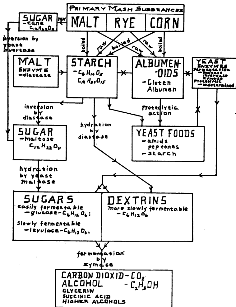
Fig. 3.—Diagram of the enzymic reactions in yeast manufacture.
