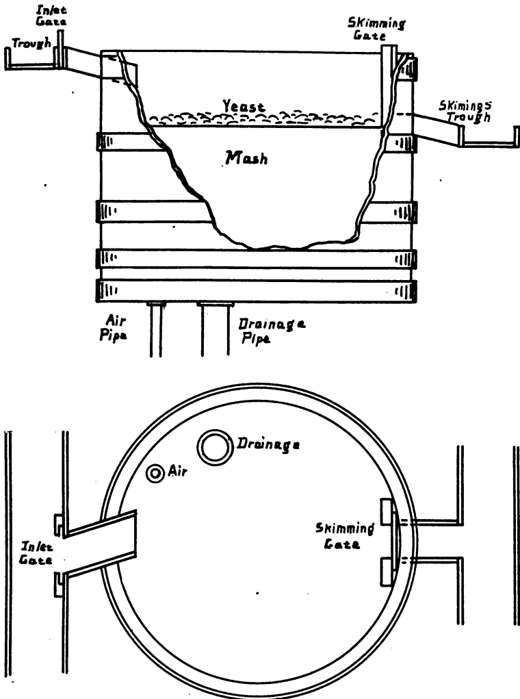
Fig. 8.—Diagram of fermenter.
