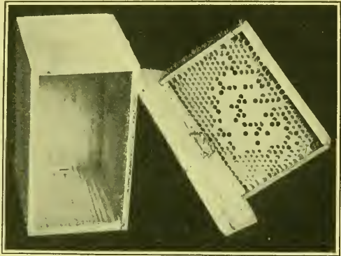
FIG. 14.—“Swarthmore” nucleus with one frame removed to show construction (original).
