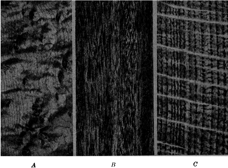
FIG. 54. A , plain-sawn bird's-eye maple. B , ribbon effect of quarter sawing "Philippine mahogany." C , quarter-sawn oak. Photographs by the Forest Products Laboratory, Madison, Wis.
