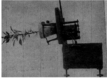
FIG. 126. An apparatus (clinostat) for rotating plants slowly about a horizontal axis, constantly changing their relation to the direction of the stimulus of gravity.
