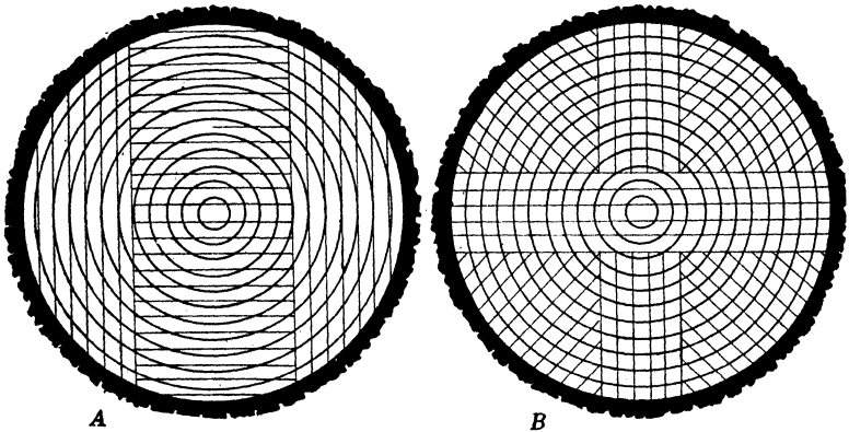
FIG. 53. Methods of sawing a log. A , plain sawing. B , quarter sawing.
