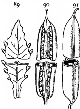
Figs. 89-91.—Single carpels.
