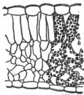
FIG. 32.—Section of a leaf.
