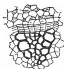
FIG. 27.—Open collateral vascular bundle.
