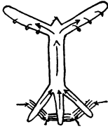
FIG. 39.—Course of water into, and through a land plant.
