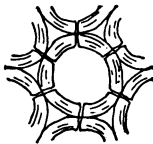
FIG. 2.—Thickened cell walls.
