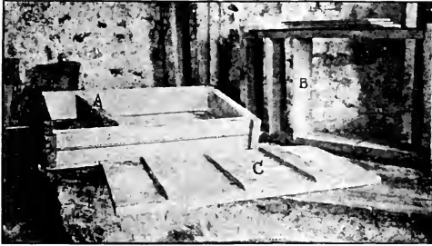
Block Swiss moulds. A, the adjustable end, moved by a screw. B, the partition which fits into the grooves, making the right sized molds after the blocks are cut. C, the cover or follower.
