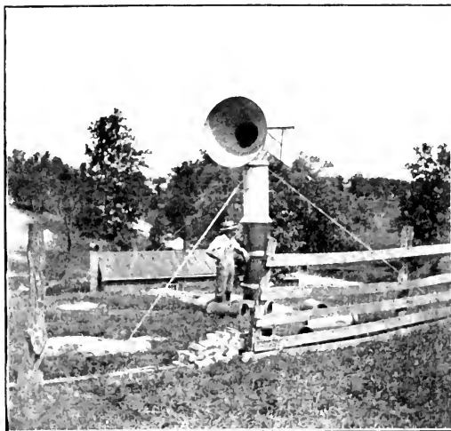
Eighteen-inch cowl to sub-earth duct at B. B. Herrick's factory, Wellington, O. The duct runs down a hill and the factory is seen at the foot of the hill.
