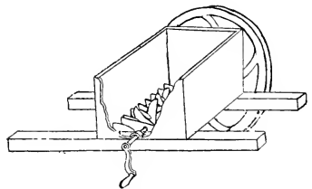
Common Knife Curd Mill
