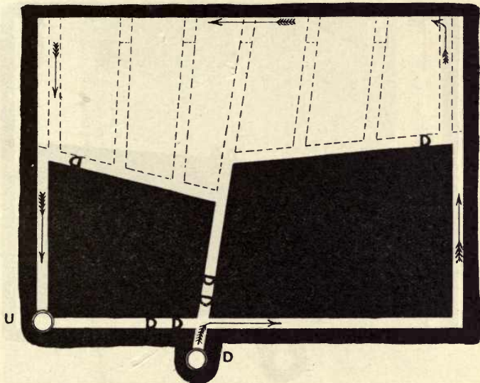
FIG. 31.—Plan showing method of ventilating a mine by a continuous current of air.
