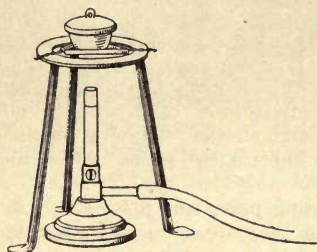
FIG. 3.—Apparatus for showing that exclusion of air stops combustion.
