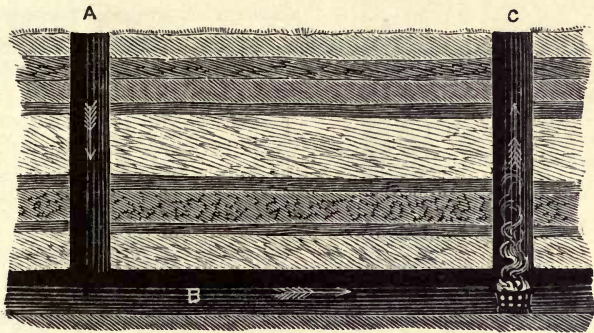
FIG. 25.—Illustrating mine ventilation by furnace: A, C, are the shafts; B, the main airway.
