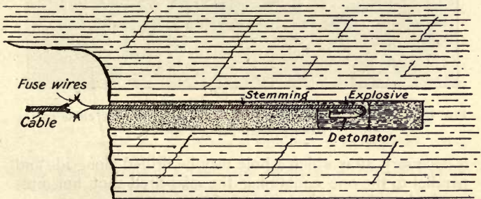
FIG. 92.—Showing method of fixing detonator in charge, and method of attaching cable to detonator wires.
