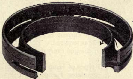
FIG. 62.—Photograph of lamp ring, showing air inlets and baffle plate. The ring is cut in order to show section.
