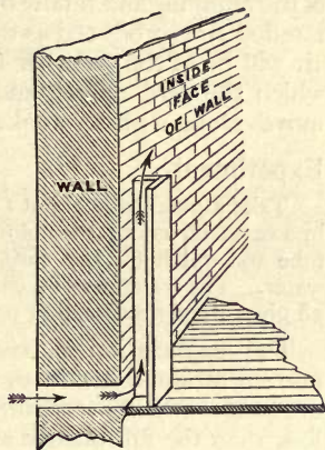
FIG. 27.—Tobin's tube.
