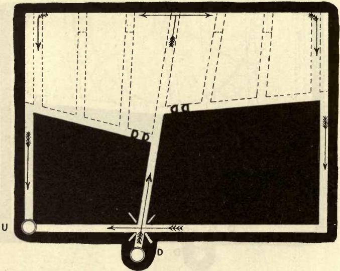
FIG. 32.—Plan showing method of splitting the air current.
