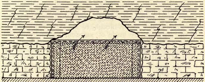
FIG. 70.—Hurdle sheet—front view.
