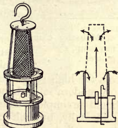
FIG. 59.—Clanny lamp, photograph and diagram.
