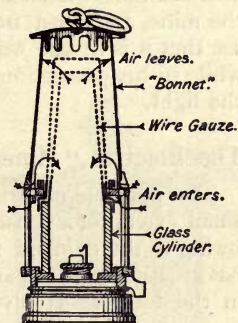
FIG. 61.—Diagram of lamp, showing air currents and construction.
