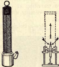
FIG. 57.—Davy lamp, photograph and diagram.
