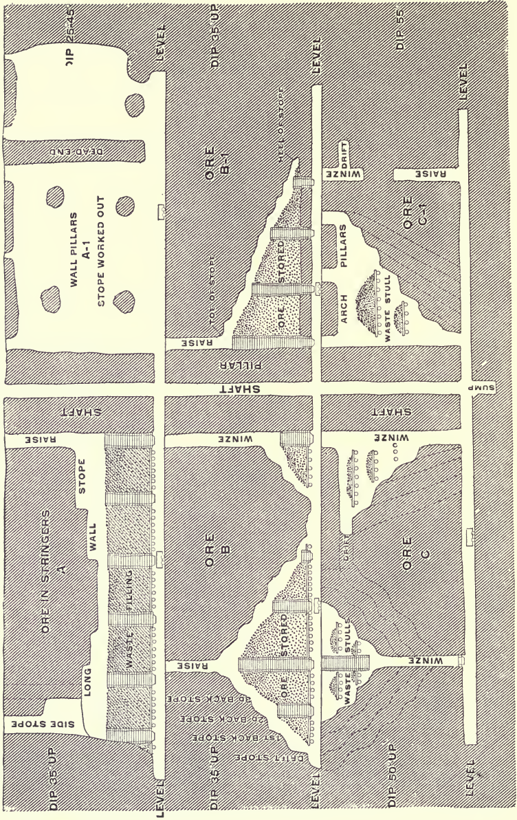
Fig. 6.—Methods of Stopping and Handling Ore. A Composite Sketch.
