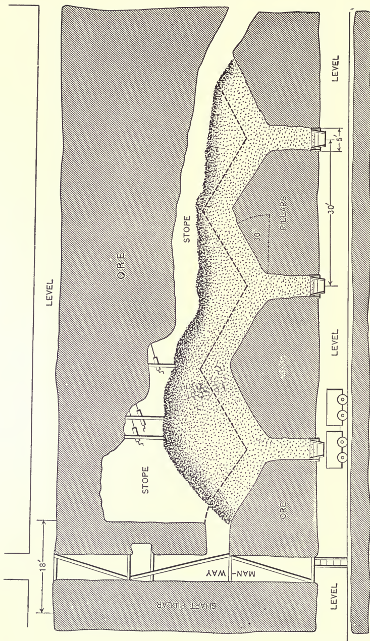
FIG. 26.— Longitudinal Section through Stope showing Method of Working by Shrinkage Stoping.
