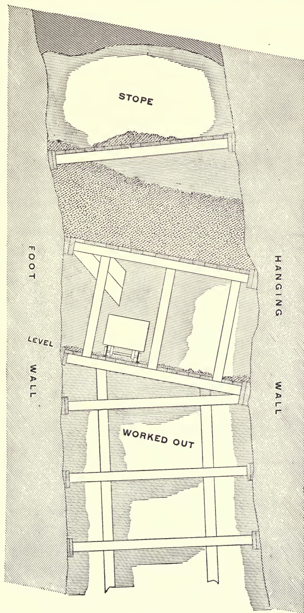
FIG. 15.—Application of Stulls to Moderately Wide Veins.
