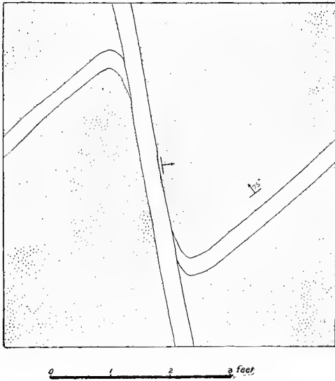
FIG. 54.—Plan of South Klingender vein faulted by the South Klingender cross vein.
