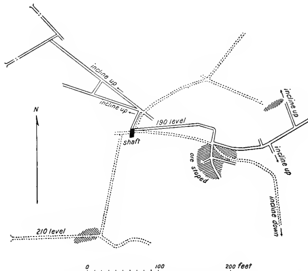
FIG. 58.—Sketch plan of the principal workings of the Union-Carbonate mine.
