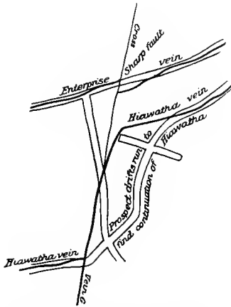
FIG. 48.—Relations of Hiawatha and Enterprise veins, as interpreted by John B. Farish.
