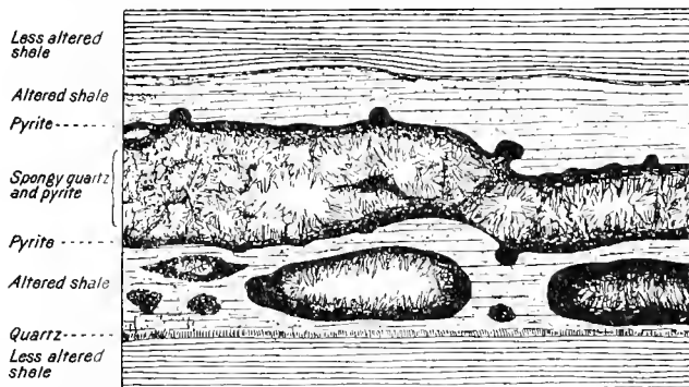
FIG. 60.—Replacement of a layer of shale by pyrite (black) and spongy quartz, showing characteristic small vugs with outer shells of pyrite and inner lining of quartz crystals.
