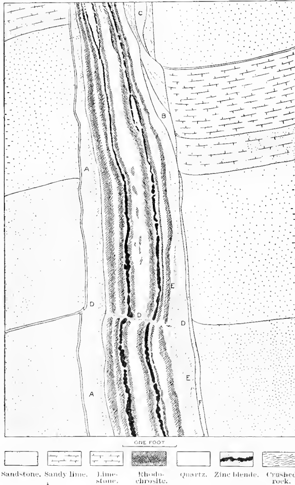
FIG. 46.—Section across the Eureka vein (after T. A. Rickard).
