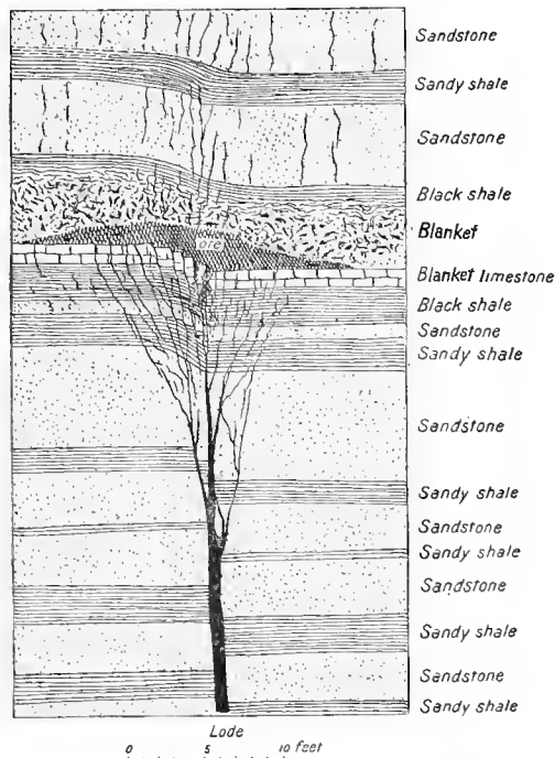
FIG. 43.—Diagrammatic section across a northeasterly lode and its blanket pay shoot.
