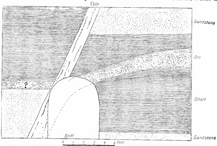
FIG. 64.—Cross section of the Sambo vein and blanket ore body, on the line A-A of fig. 63.
