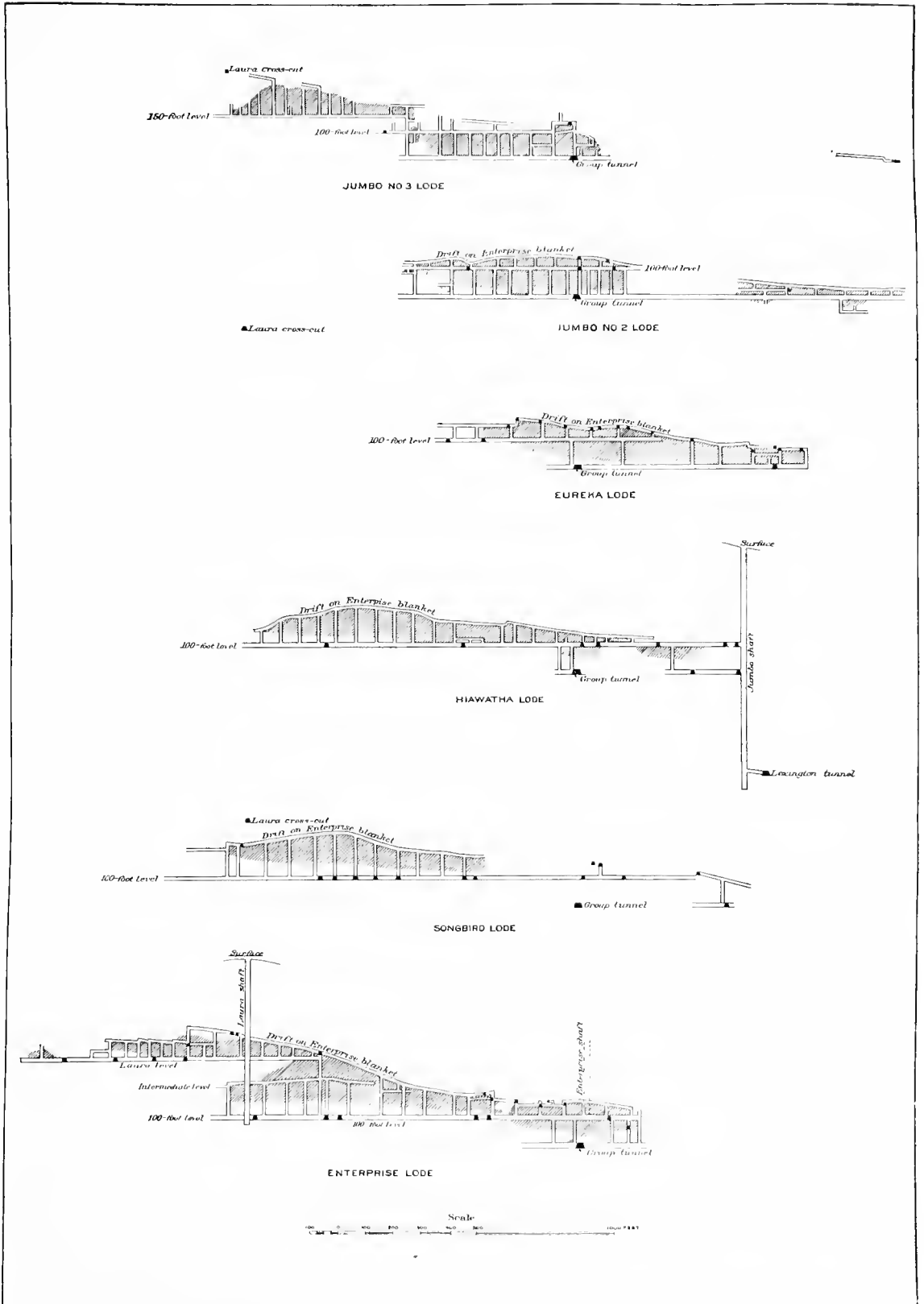
LONGITUDINAL SECTIONS OF THE PRINCIPAL NORTHEASTERLY LODES OF THE ENTERPRISE MINE. Showing undulations and faults in the overlying Enterprise blanket and the extent of the lode ore bodies. Shaded areas indicate steps
