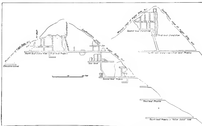
FIG. 67.—Longitudinal sections through the Grand View and Phoenix veins.
