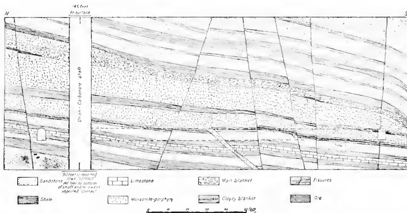
FIG. 59.—Diagrammatic north-south section through the Union-Carbonate mine, illustrating the general structure of the country rock, and showing some of the northwesterly fissures and their relation to the blankets and ore bodies.
