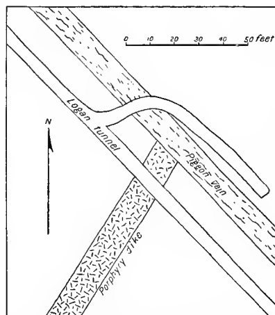
FIG. 70.—Diagram illustrating faulting of a porphyry dike by the Pigeon lode fissure in Logan mine.
