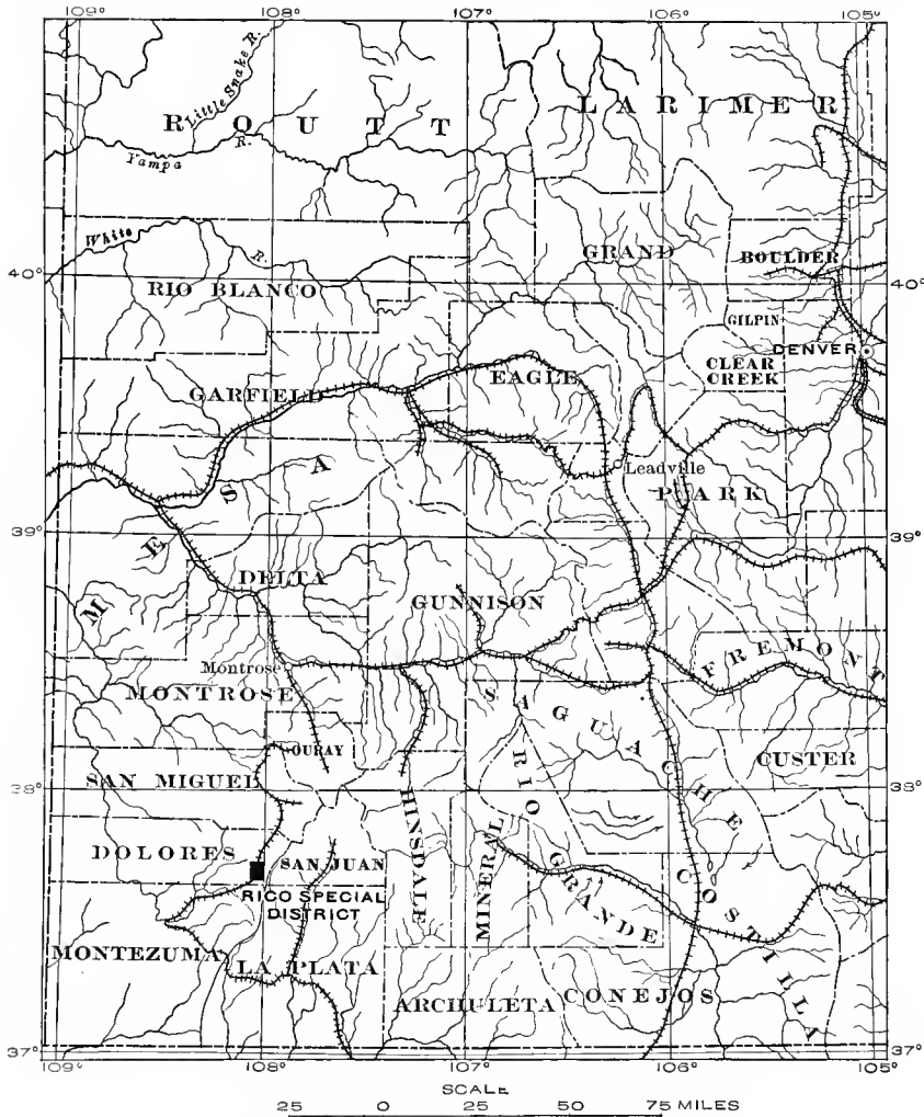
FIG. 39.—Index map showing position of Rico district.
