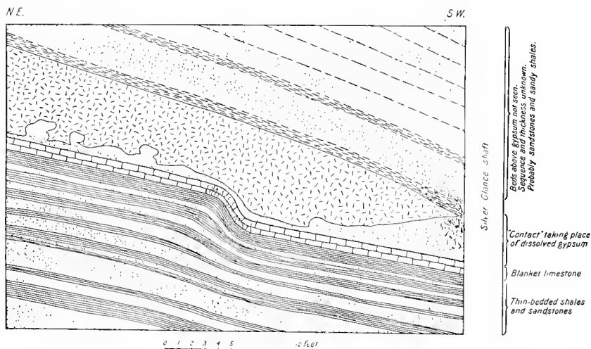
FIG. 56.—Partly diagrammatic sketch of the gypsum "contact" and inclosing beds at the Silver Glance shaft, Rico-Aspen mine.
