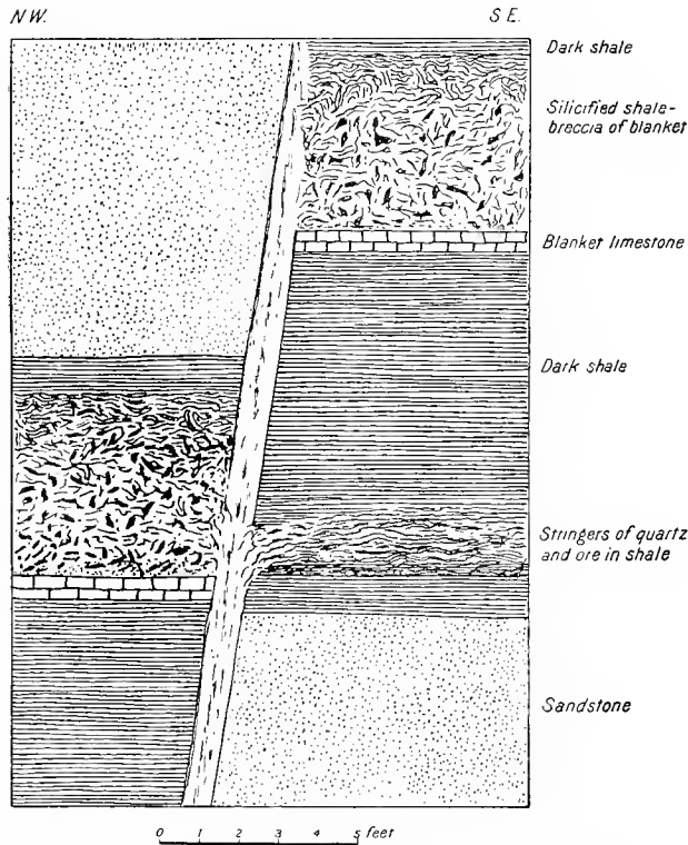
FIG. 55.—Diagrammatic section through the Montezuma vein, showing faulting of blanket and occurrence of a second ore-bearing horizon below the blanket limestone.
