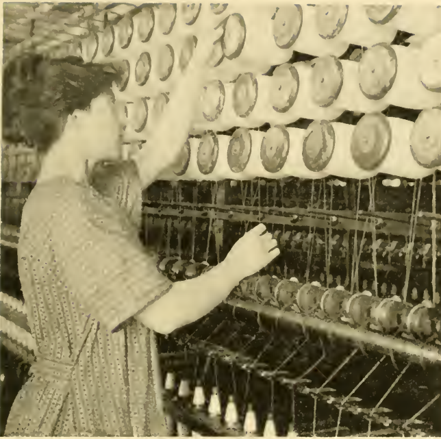
Ring Twister.
