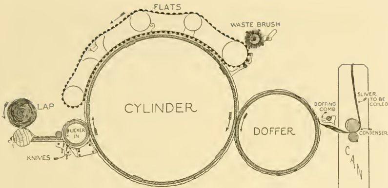
PRINCIPLE OF THE FLAT CARD
