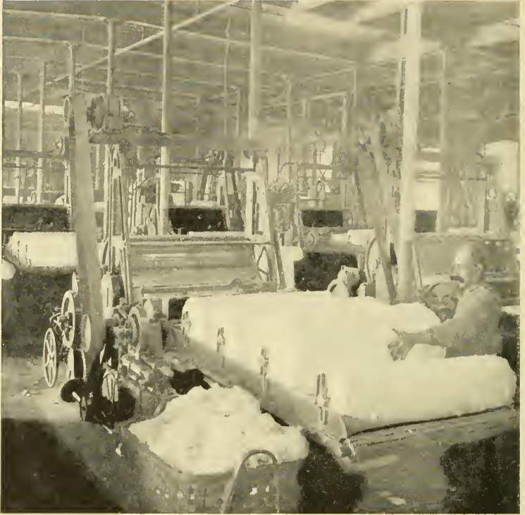
Picker Room.
