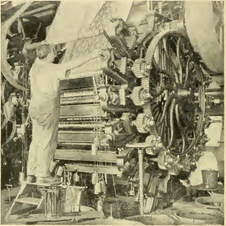
Printing Machine.
