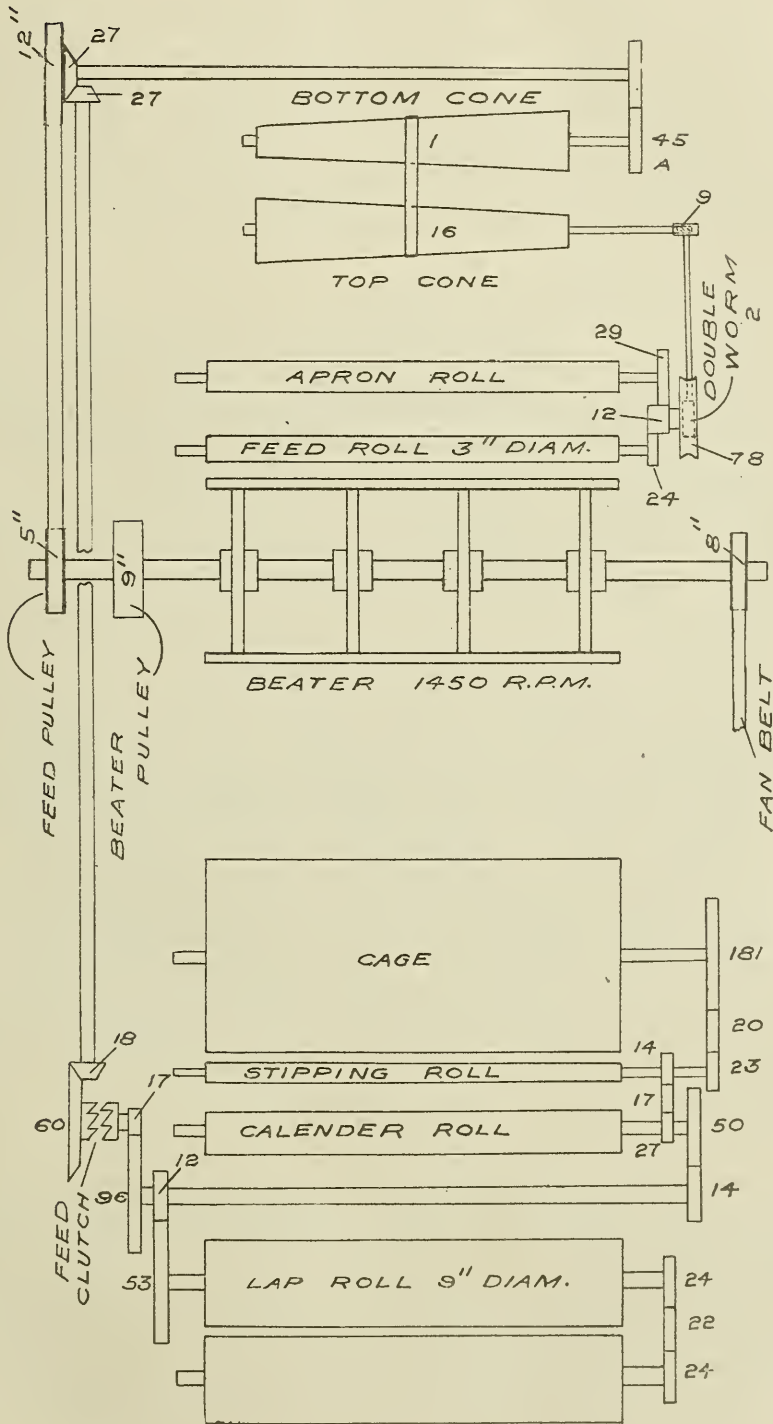
FIG. 9. GEARING PLAN OF HOWARD & BULLOUGH FINISHER PICKER.
