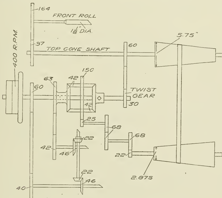
FIG. 38. SPINDLE AND BOBBIN GEARING. LOWELL 7 BY 3½ INCH FLY FRAME.
