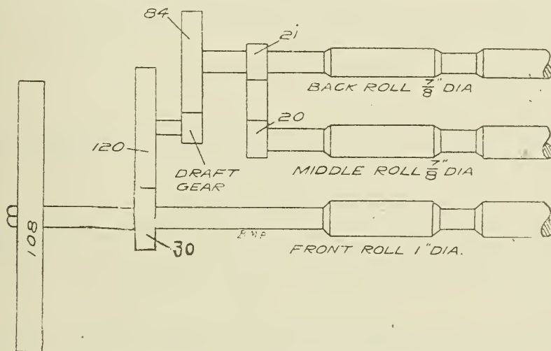
FIG. 41. DRAFT GEARING OF FALES & JENKS SPINNING FRAME.
