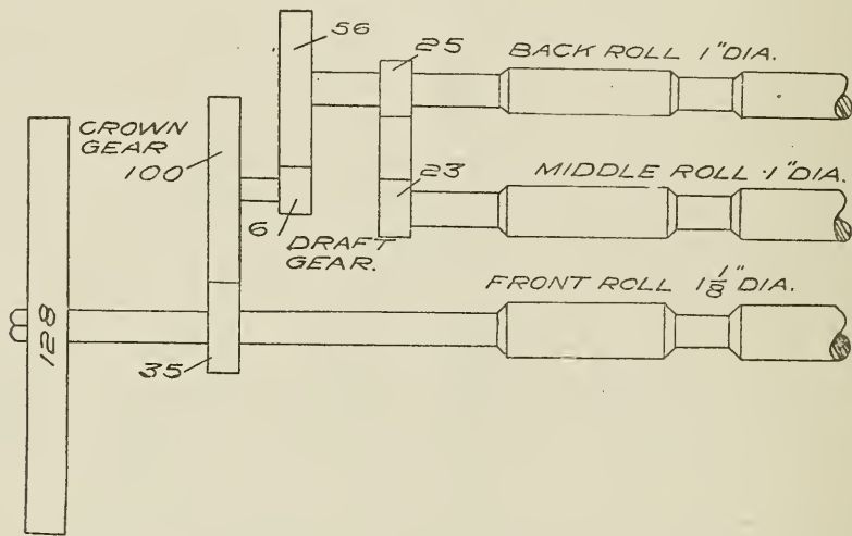
FIG. 34. DRAFT GEARING ON WOONSOCKET FLY FRAMES.
