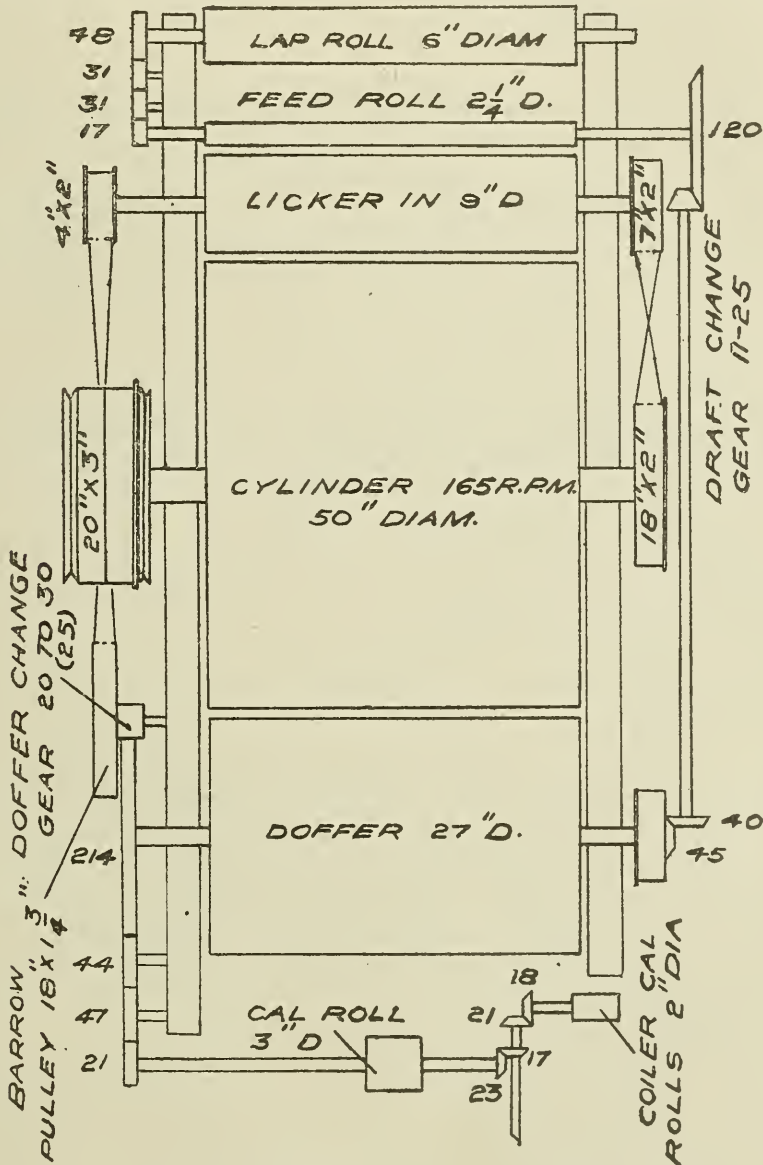
FIG. 12. PLAN OF GEARING ON THE SACO-PETTEE CARD.
