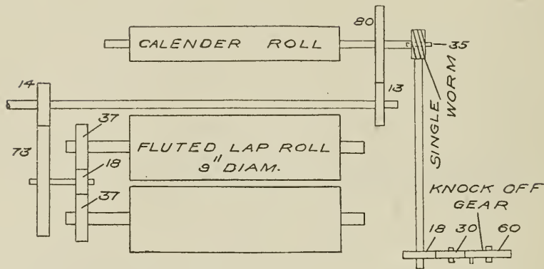
FIG. 6. DIAGRAM OF KNOCK-OFF GEARING.
