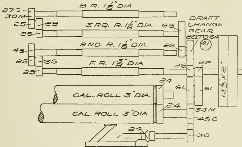
FIG. 28. GEARING PLAN OF LOWELL DRAWING FRAME.
