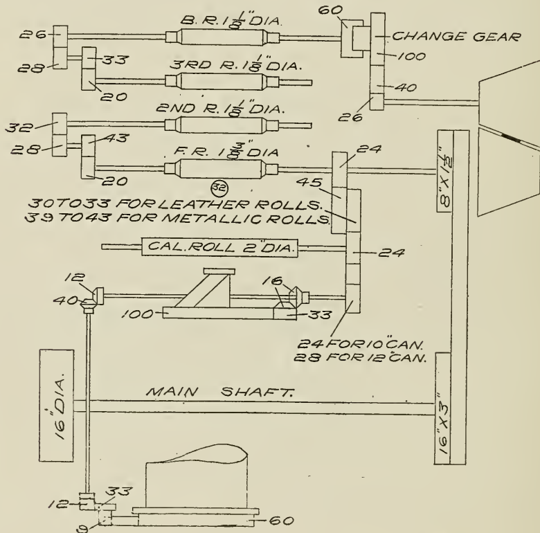
FIG. 27. GEARING PLAN OF SACO-PETTEE RAILWAY HEAD.
