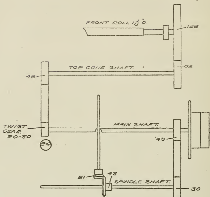
FIG. 35. TWIST GEARING ON WOONSOCKET FLY FRAMES.
