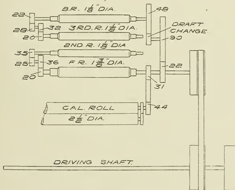
FIG. 32. GEARING PLAN OF MASON DRAWING FRAME.
