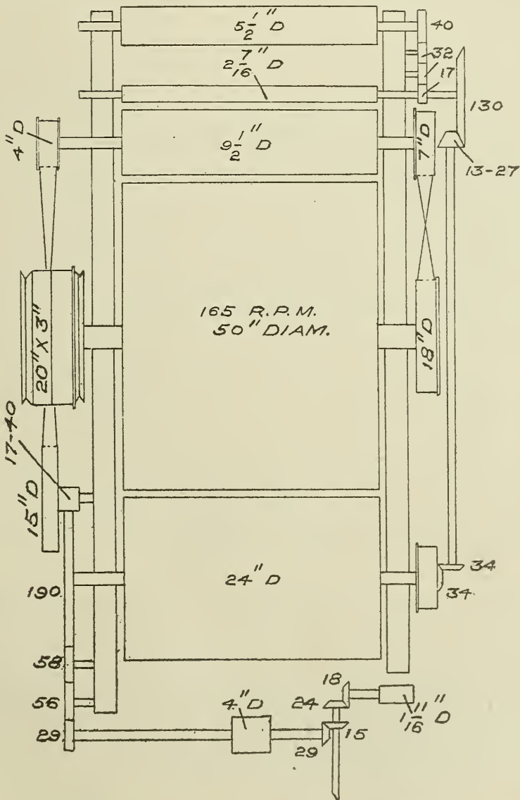
FIG. 13. PLAN OF GEARING ON THE MASON CARD.
