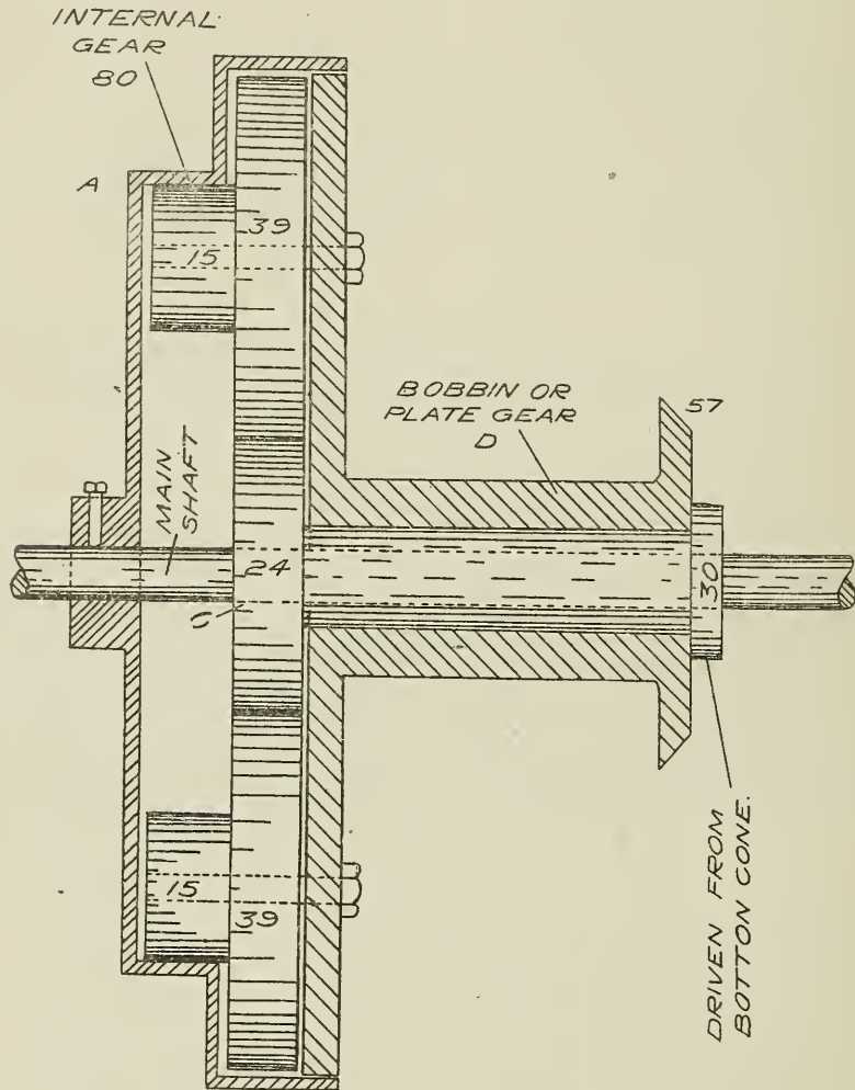
FIG. 37. DALY DIFFERENTIAL.
