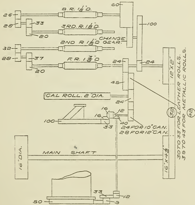
FIG. 30. GEARING PLAN OF SACO-PETTEE DRAWING FRAME.
