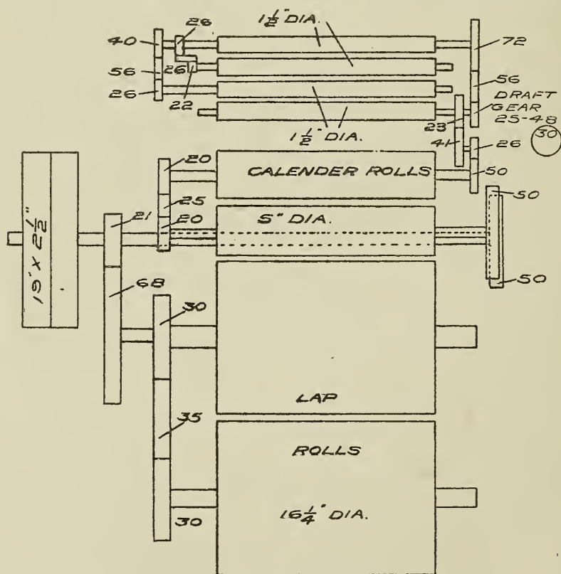
FIG. 19. GEARING PLAN OF WHITIN SLIVER LAPPER.
