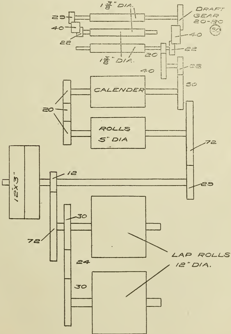
FIG. 20. PLAN OF GEARING ON MASON SLIVER LAPPER.
