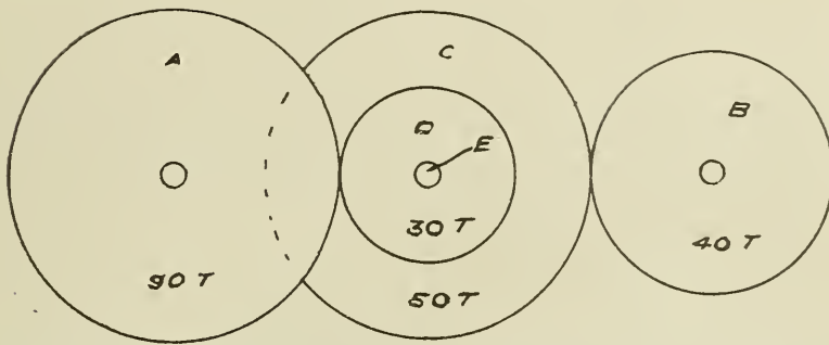
FIG. 2. DIAGRAM ILLUSTRATING A COMPOUND TRAIN OF GEARING IN MESH.
