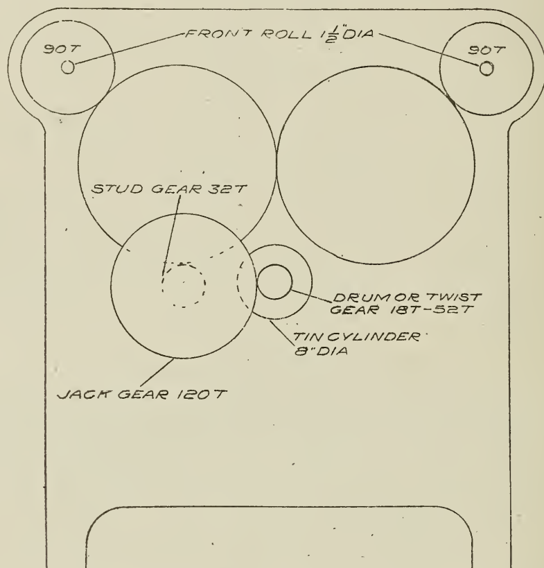
FIG. 45. TWIST GEARING ON THE DRAPER TWISTER.
