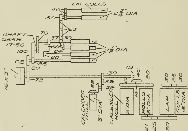
FIG. 22. GEARING PLAN OF MASON RIBBON LAPPER.
