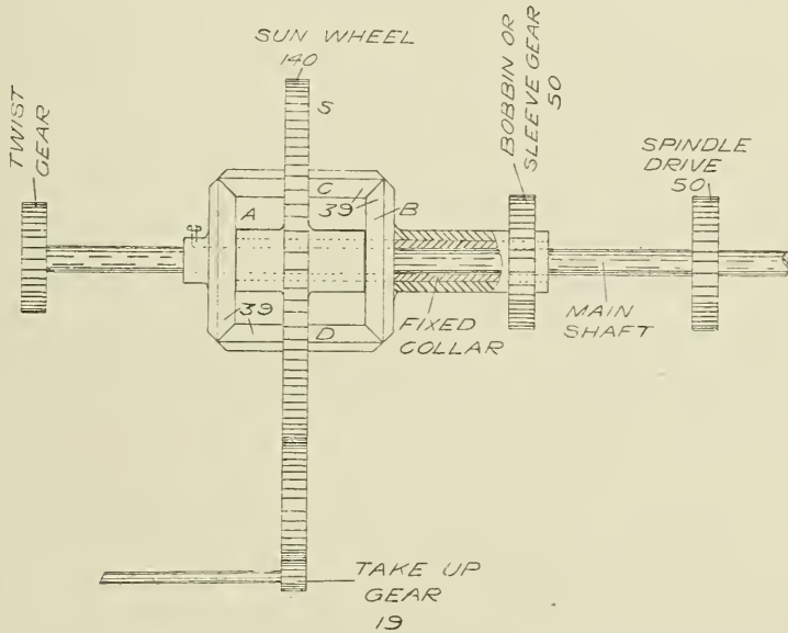
FIG. 36. THE BEVEL GEAR DIFFERENTIAL MOTION OR COMPOUND.
