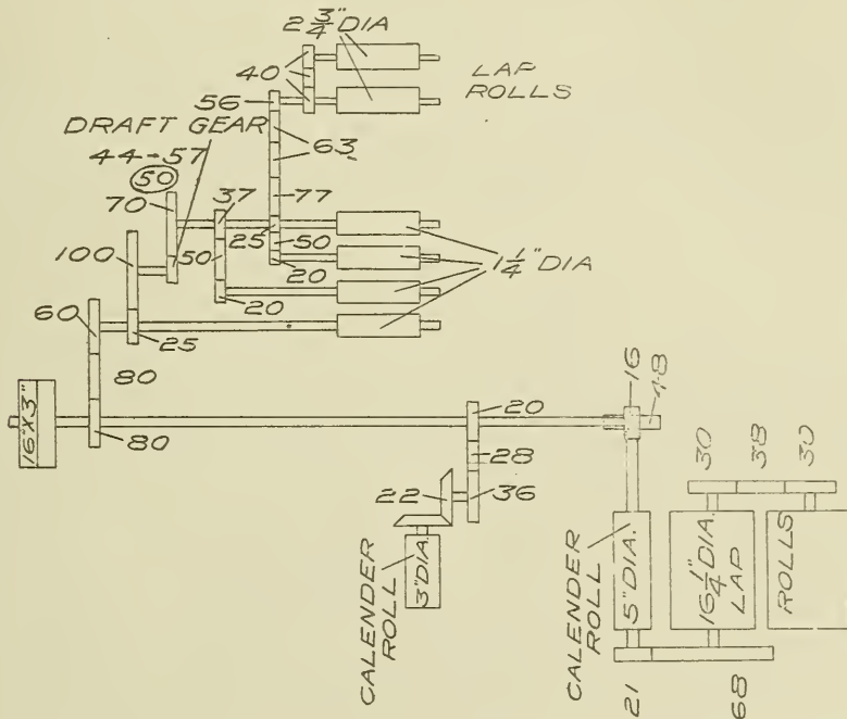
FIG. 21. GEARING PLAN OF WHITIN RIBBON LAPPER.
