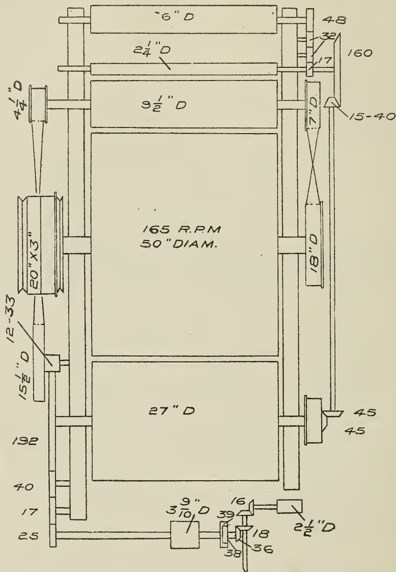
FIG. 14. PLAN OF GEARING ON THE WHITIN CARD.
