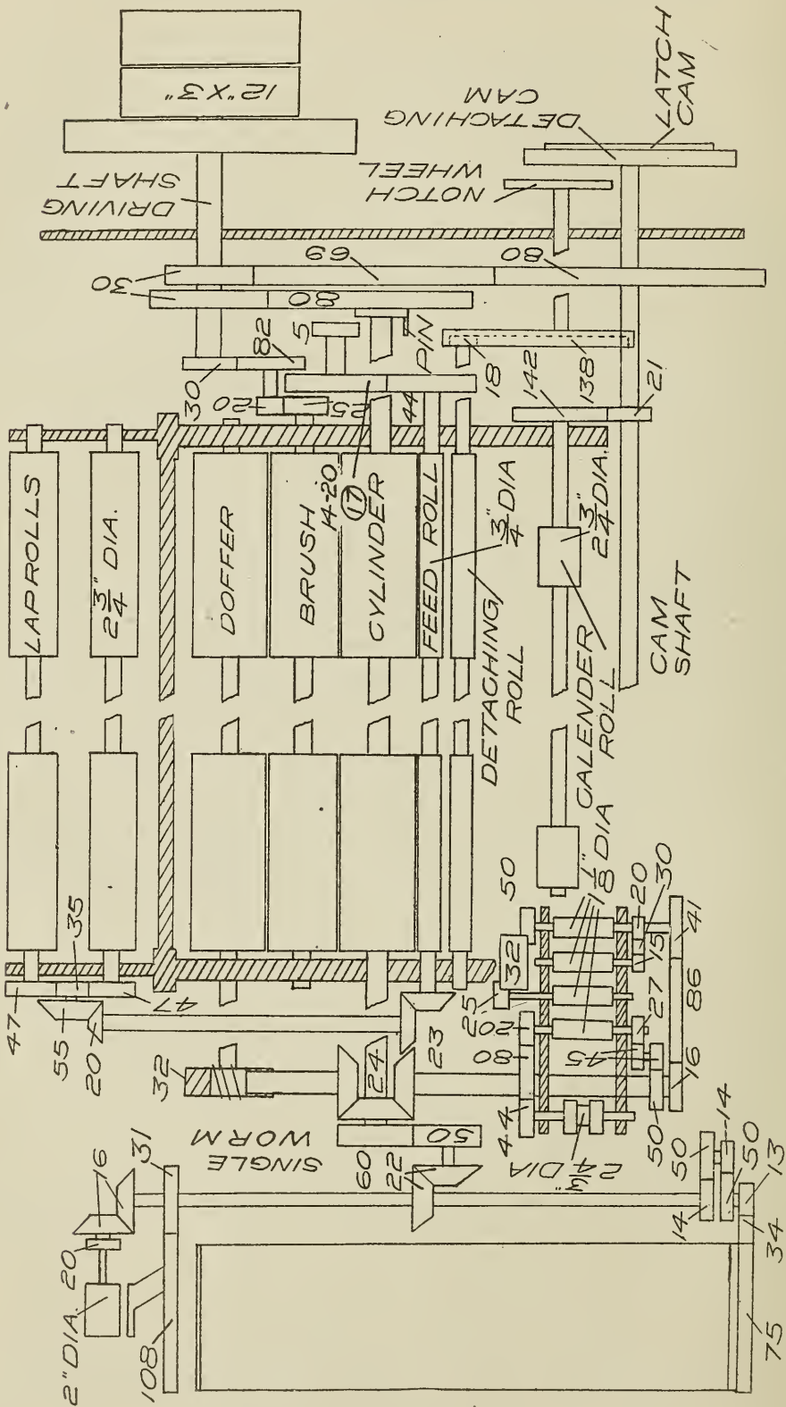
FIG. 23. GEARING DIAGRAM OF WHITIN COMBER.
