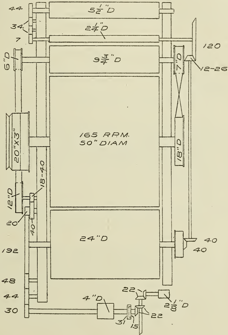
FIG. 15. PLAN OF GEARING ON THE LOWELL CARD.
