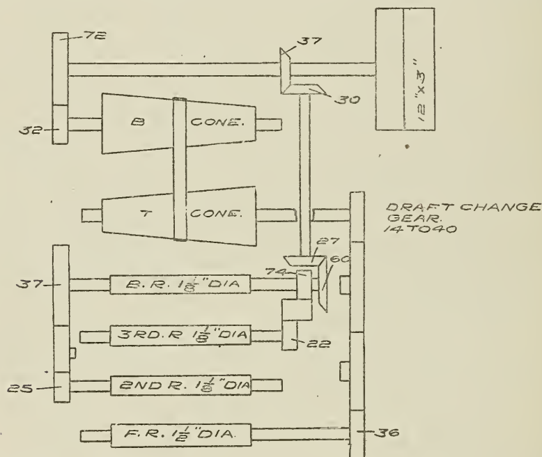
FIG. 25. GEARING PLAN OF LOWELL RAILWAY HEAD.
