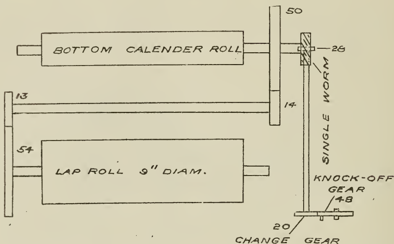
FIG. 8. DIAGRAM OF KNOCK-OFF GEARING ON ATHERTON PICKER.
