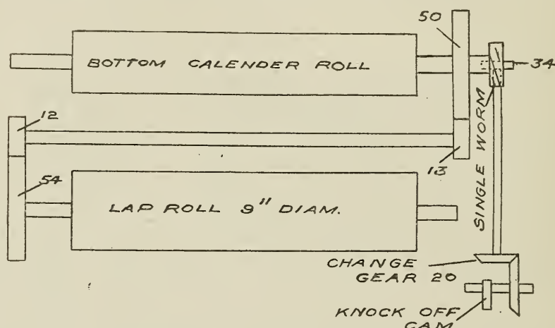
FIG. 11. KNOCK-OFF GEARING ON POTTER & JOHNSTON PICKER.
