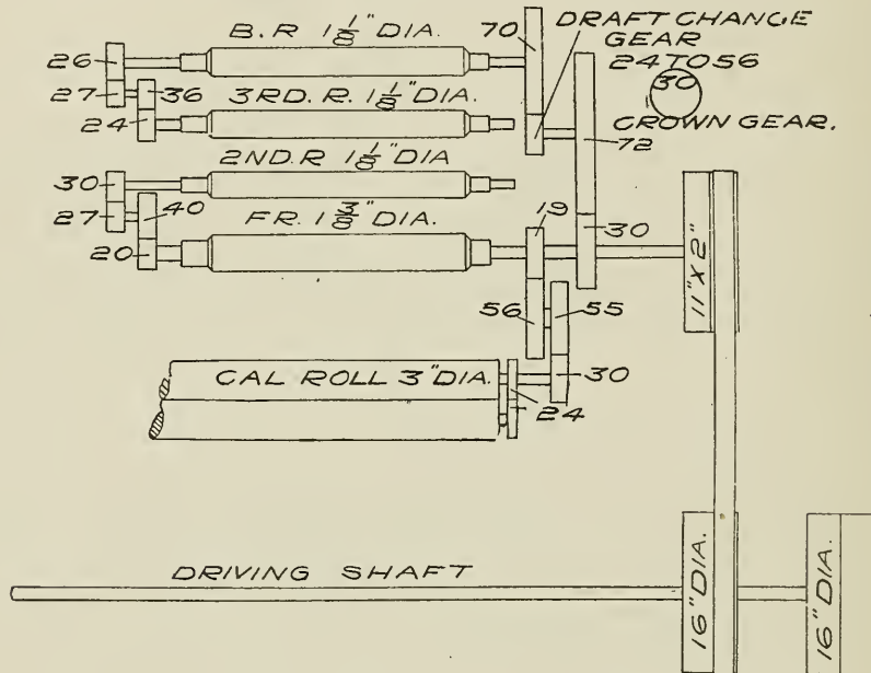
FIG. 29. GEARING PLAN OF WHITIN DRAWING FRAME.
