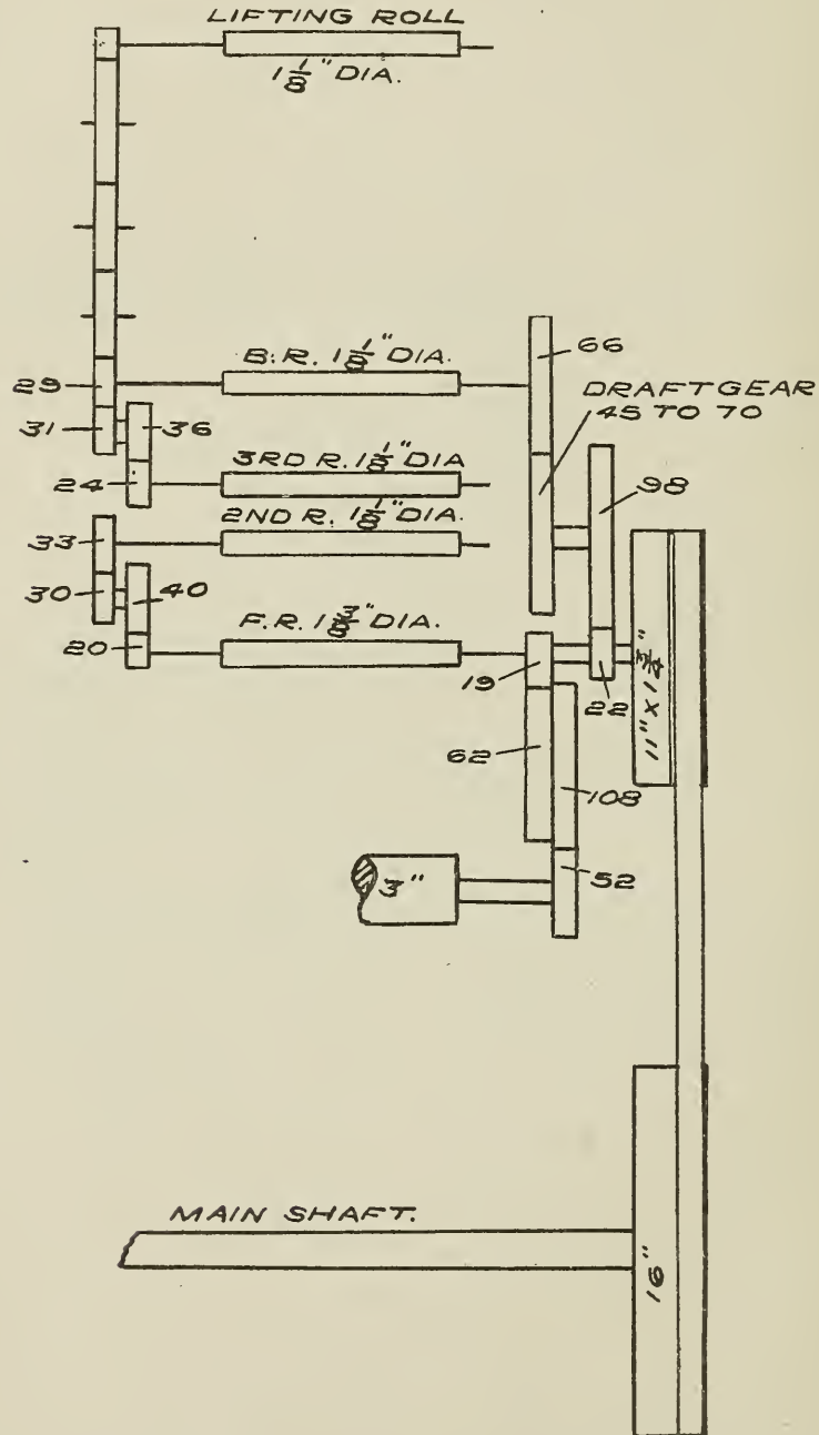
FIG. 31. GEARING PLAN OF HOWARD & BULLOUGH DRAWING FRAME.
