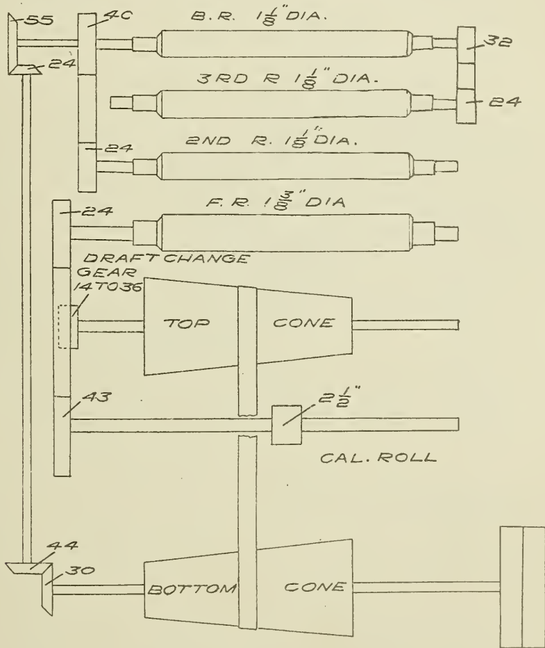
FIG. 26. GEARING PLAN OF WHITIN RAILWAY HEAD.
