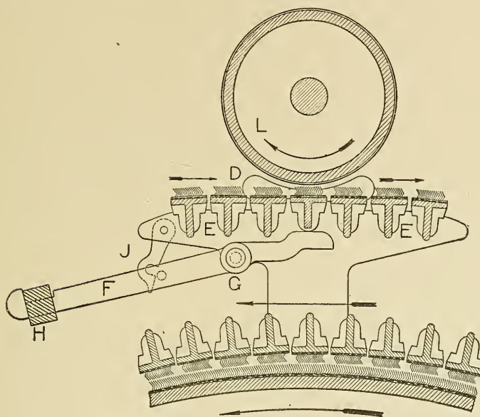
Fig. 95. Section Showing Flat Grinder.
