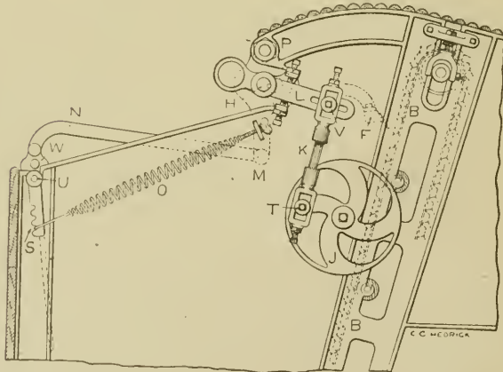
Fig. 30. Elevation Showing Evener Parts.
