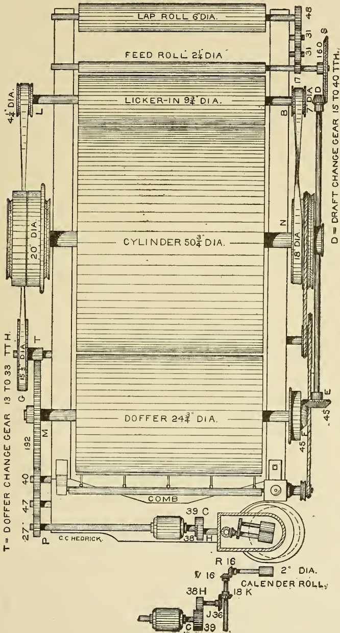
Fig. 105. Diagram of Gearing. Whittin Machine Works Revolving Flat Card.
