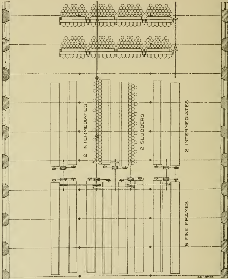
Fig. 150. Plan of Card Room Showing Fly Frames.
