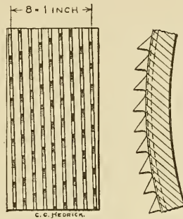
Fig. 73. Saw tooth clothing.
