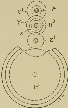
Fig. 63. Plan of turn-table gearing.
