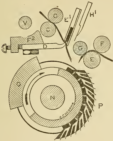
Fig. 121. Sections showing Detaching Rolls and Cylinder.
