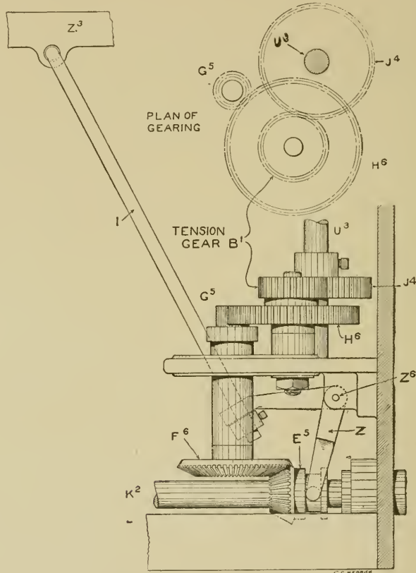
Fig. 173. Tension Gearing.
