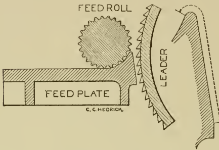
Fig. 52. Feed Plate for Egyptian Cotton.
