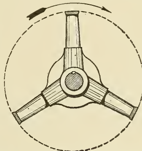
Fig. 12. Three-bladed Beater.
