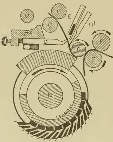
Fig. 123. Sections showing Detaching Rolls and Cylinder.
