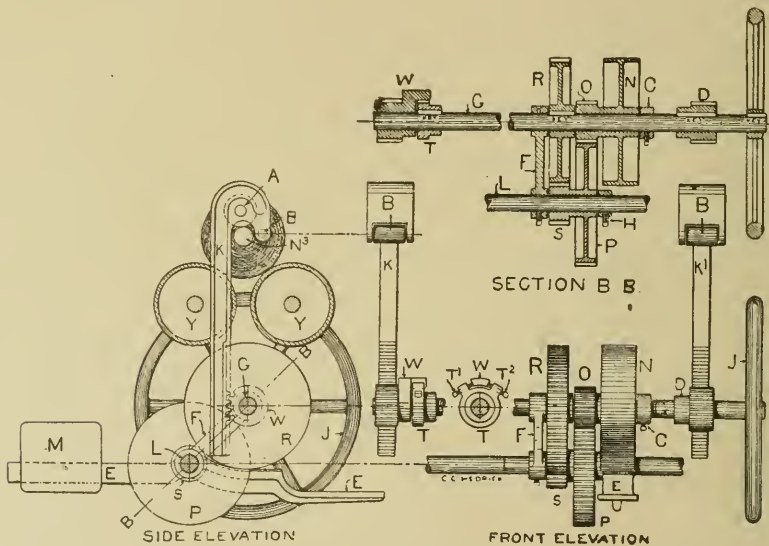
Fig. 43. Friction Let-off.
