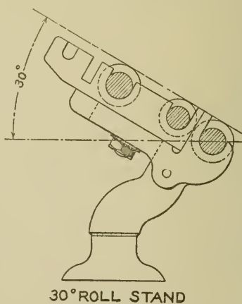
Fig. 199. Roll Stand, 30° Pitch, for Overhanging Front Rolls.
