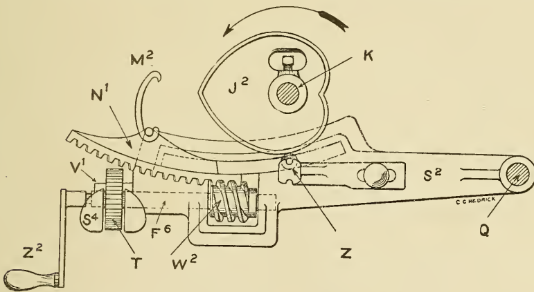
Fig. 210. Warp Builder.
