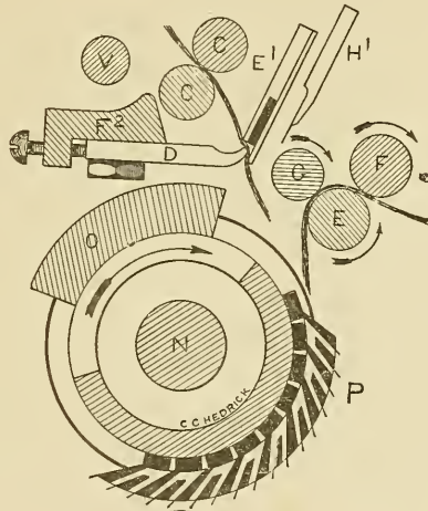
Fig. 121. Sections showing Detaching Rolls and Cylinder.
