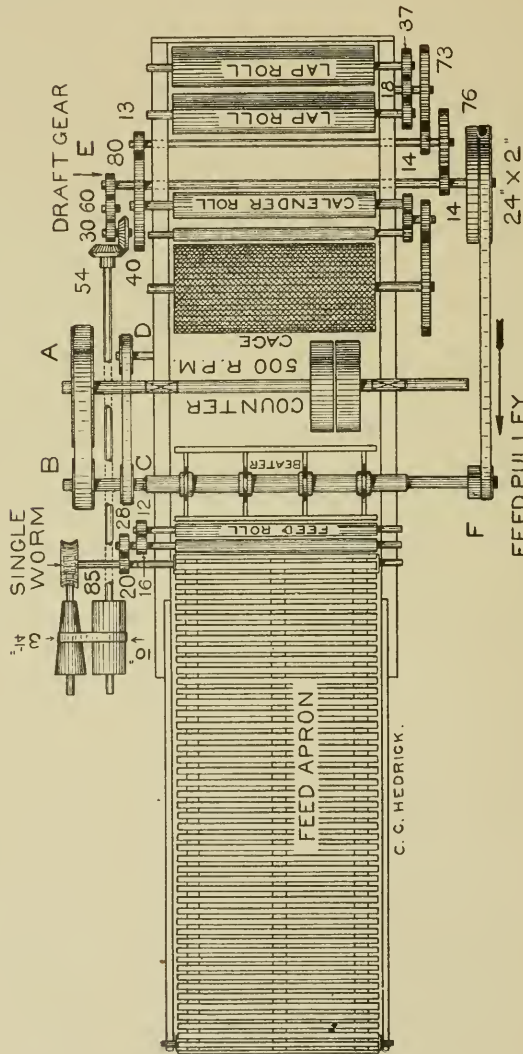
Fig. 46 Diagram of Gearing of Finishing Picker.
