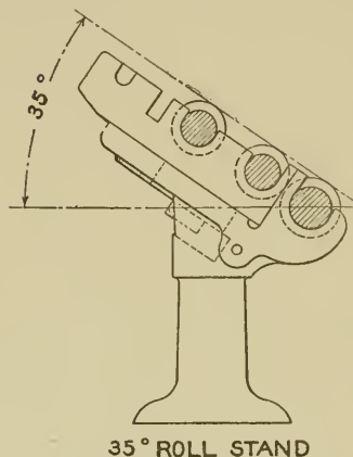
Fig. 198. Filling Roll Stand, 35° Pitch.
