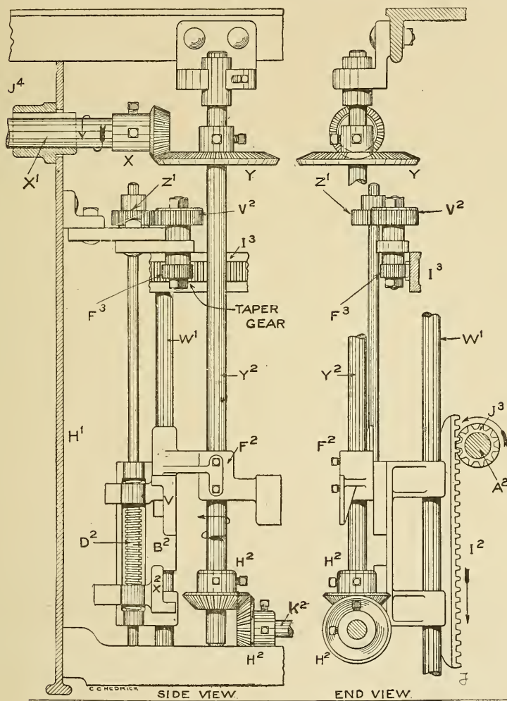
Fig. 170. Builder.
