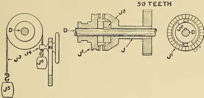
Fig. 241. Snarling Motion.
