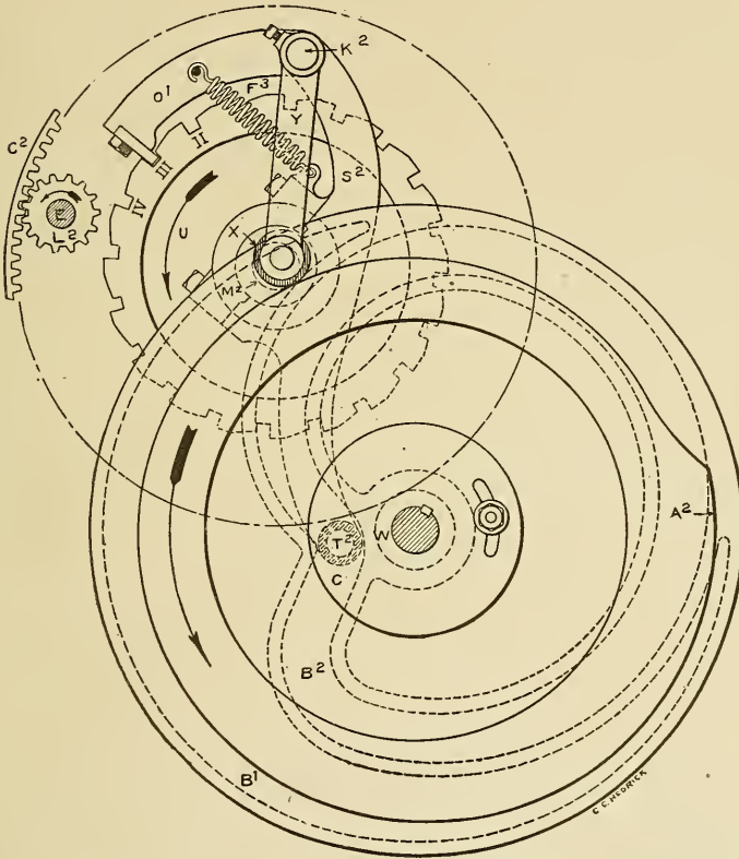
Fig. 126. Elevation Showing Detaching Roll Cams.
