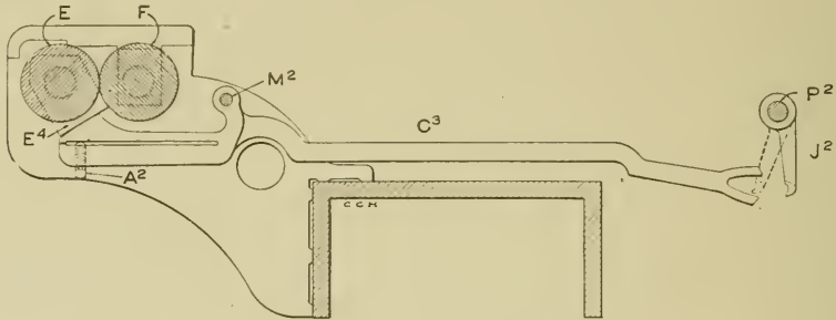
Fig. 149. Calendar Roll Stop Motion.
