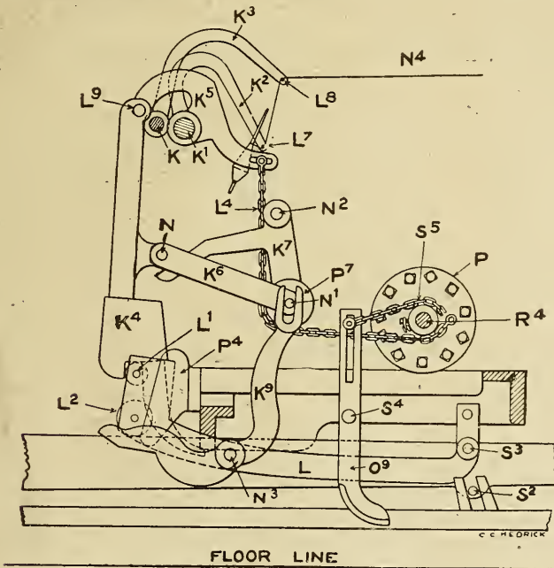
Fig. 226. Elevation Showing Details of Mule Carriage.
