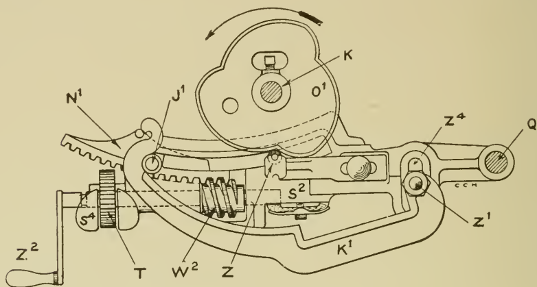
Fig. 215. Combination Builder.
