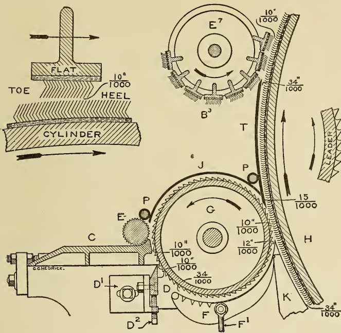
Fig. 57. Section of cylinder, leader and flat.
