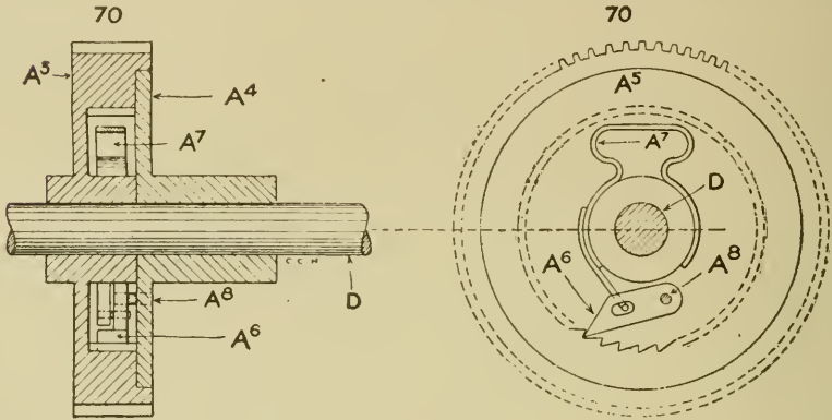
Fig. 240. Roller Motion.
