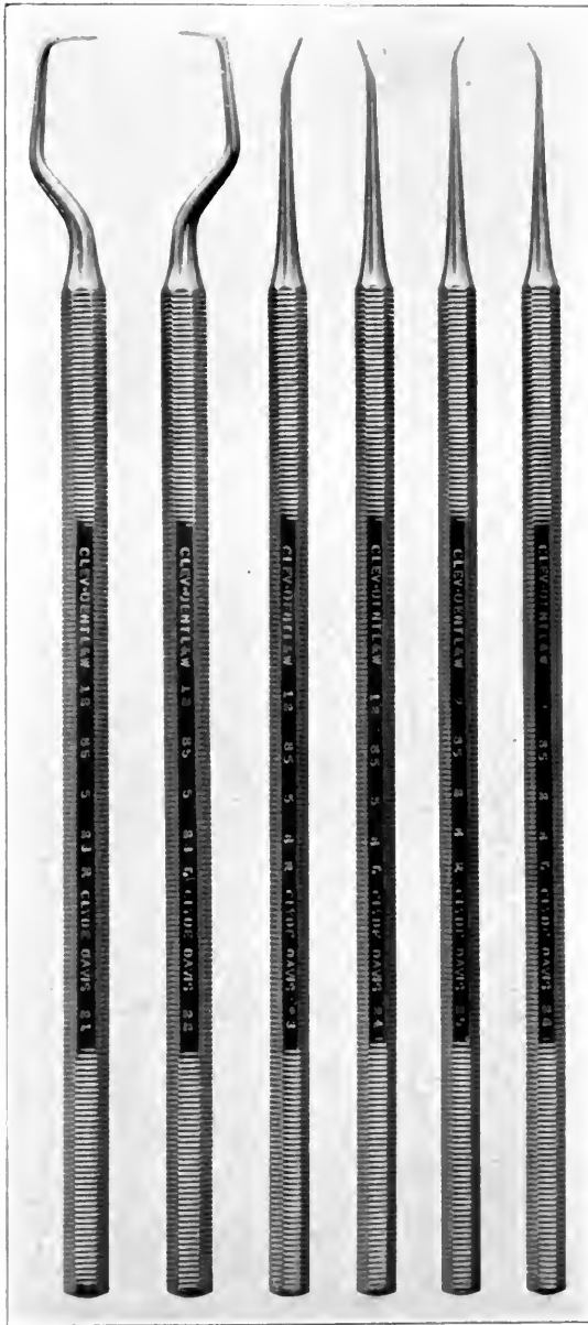
Fig. 173.—Excavators, group four. Instruments for cutting point angles and sharpening base line angles.
