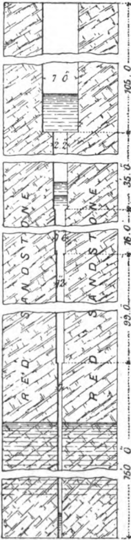
NEW ENGINE WELL, BIRKENHEAD WATERWORKS.
