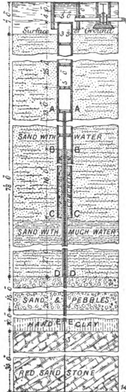
WELL AT ASPINALL'S BREWERY, BIRKENHEAD.
