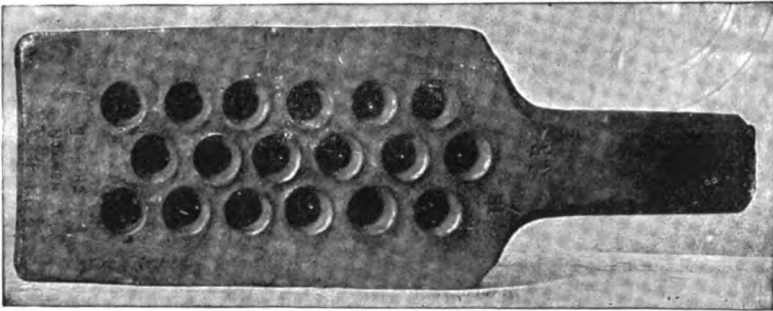
Drawplate for Wire-drawing.
