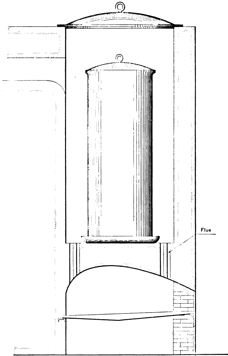
Annealing Pot and Furnace.
