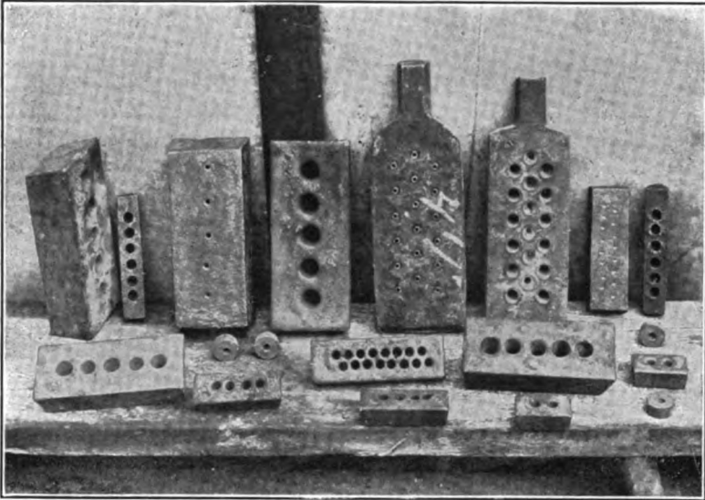
Steel and Cast-iron Dies.
