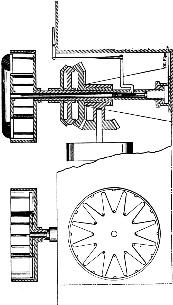
Morgan Reel.
