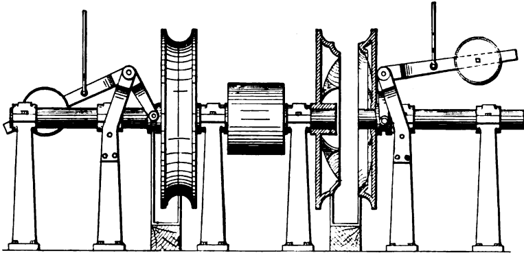
Direct-traction Reel.
