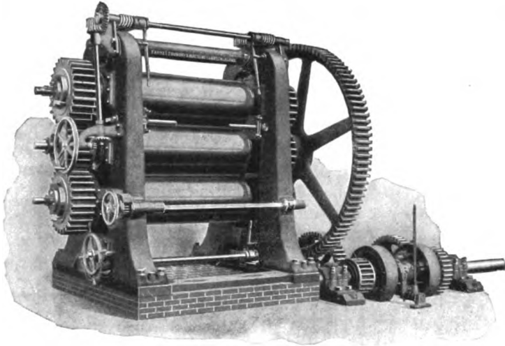
Calender Rolls.
