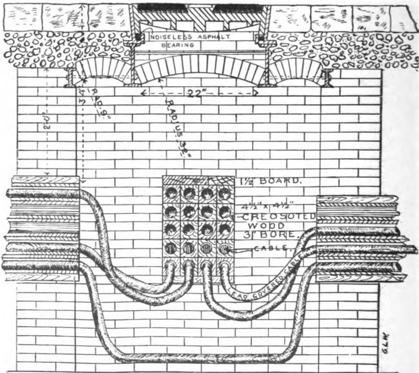
4'-13" x 4'-6" x 13" SECTION OF MANHOLE, WITH CREOSOTED WOOD CONDUITS.
