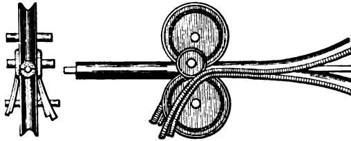
Rubber-covering Wheels.
