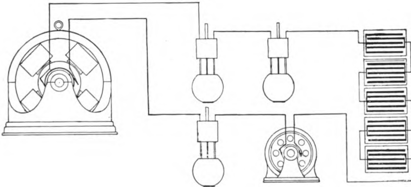
Series Connection.
