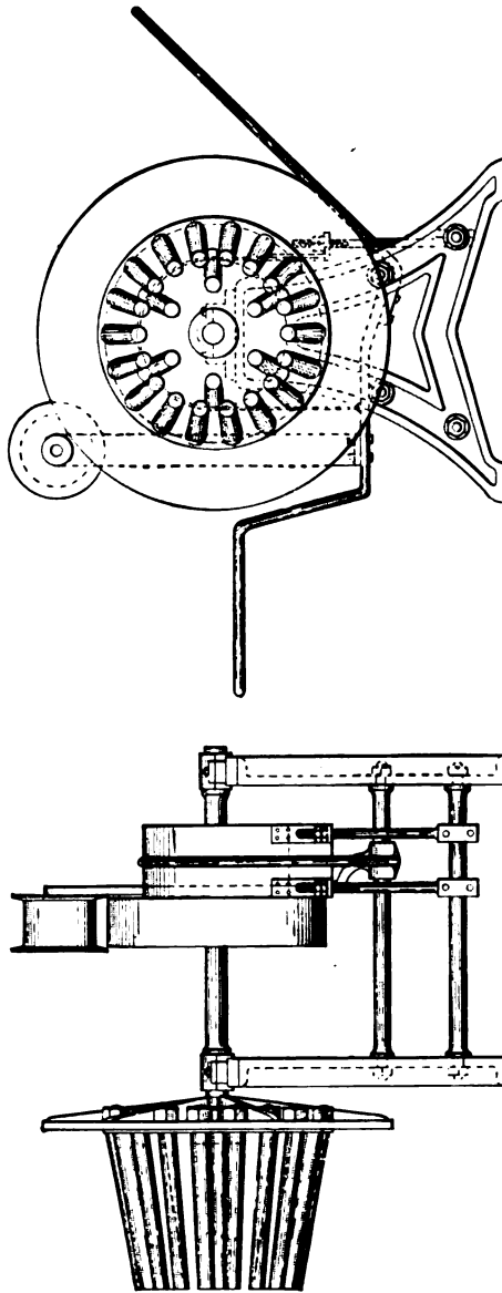
Loose Belt-reel.
