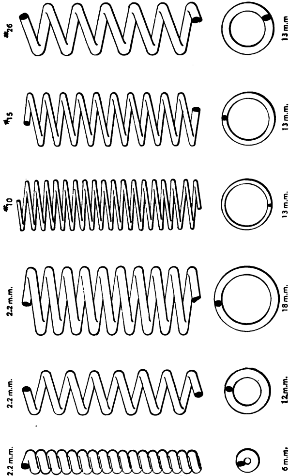
The Coils of Herr Dettmar, full size.
