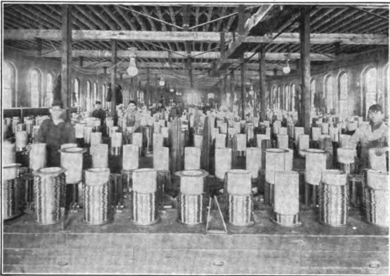
Fine Wire-room.
