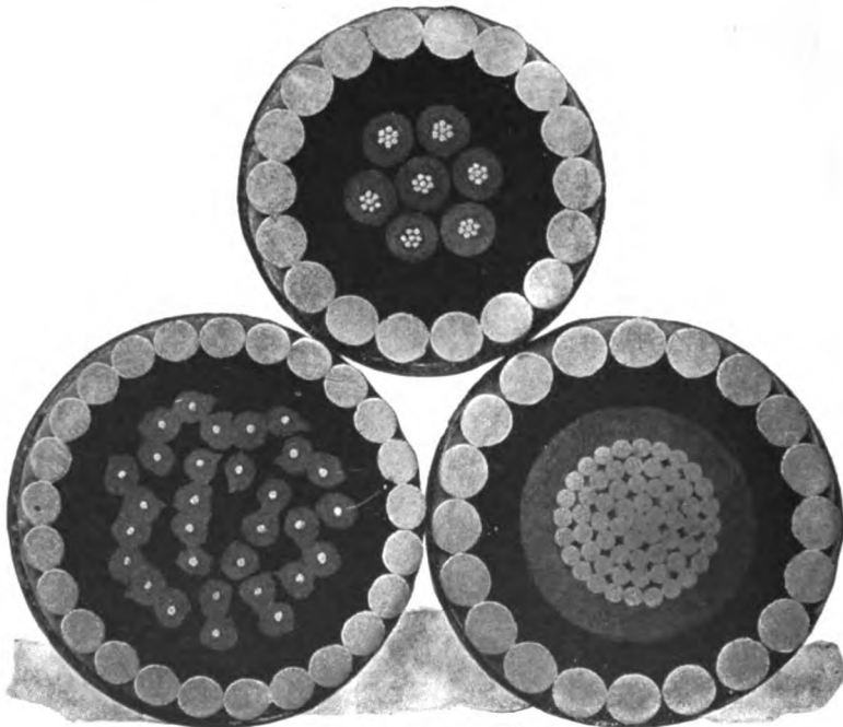
Cables for Bays and Rivers. Submarine Telegraph Cable, 7-Conductor.
