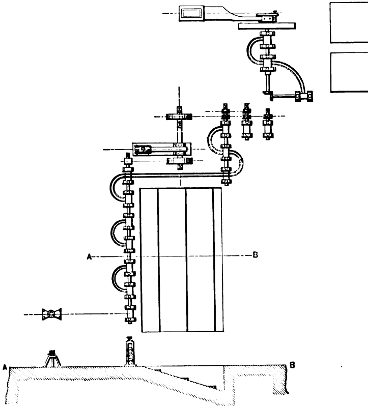
Garrett Rod-mill.
