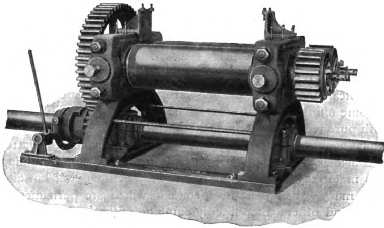
Grinding Rolls for Mixing Rubber.
