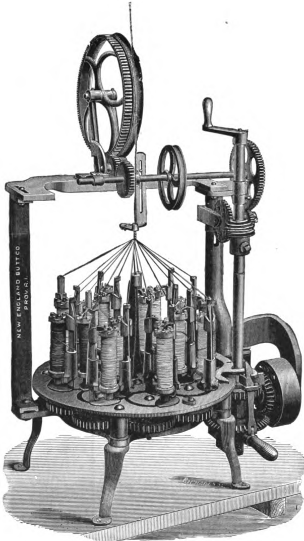
Braiding Machine.
