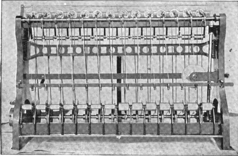
Fine Wire Insulating Machine.
