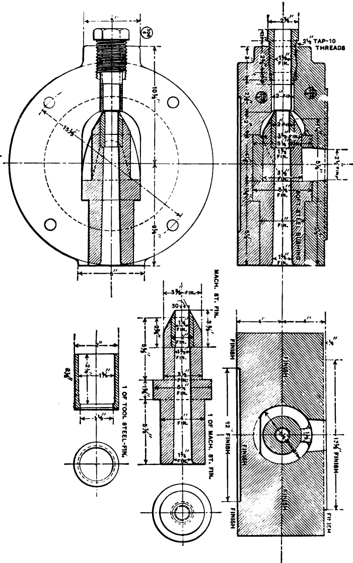
Core-box with Core and Die.
