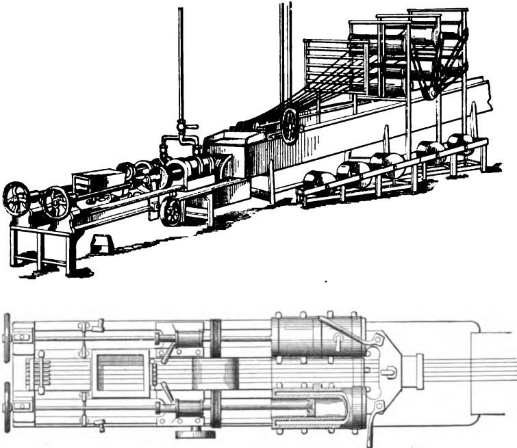
Gutta-percha Covering Machine.
