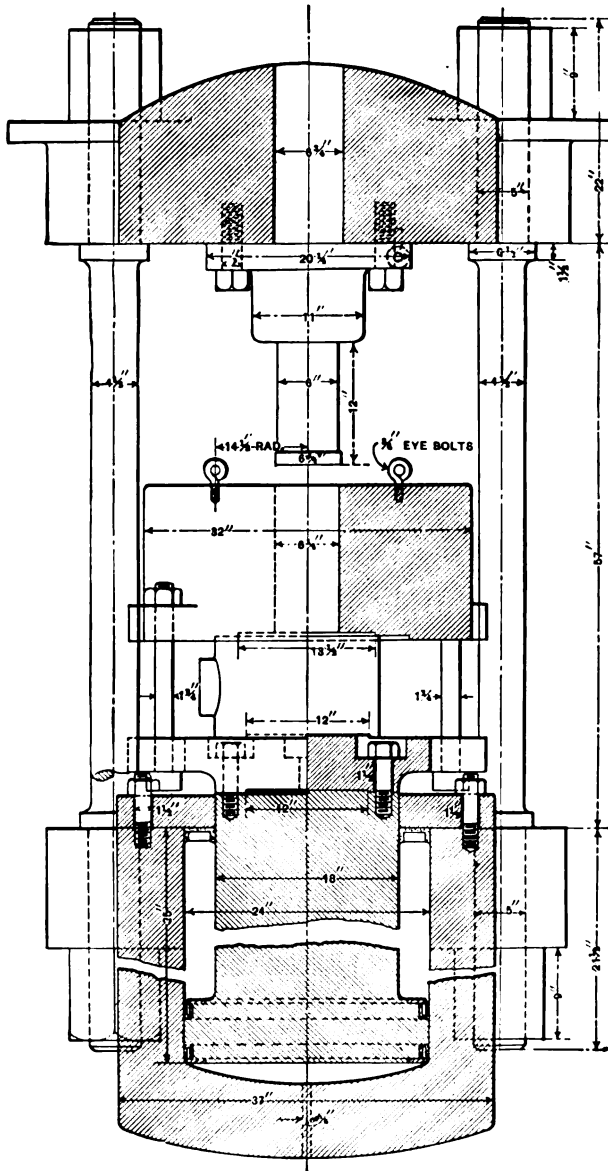
Lead-incasing Press.
