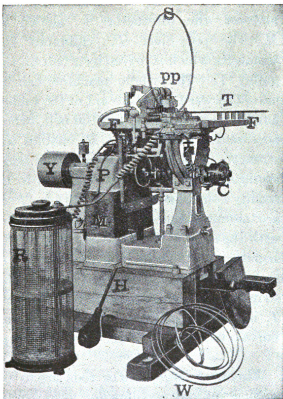
FIG. 59.—DIRECT-WELDING APPARATUS.
