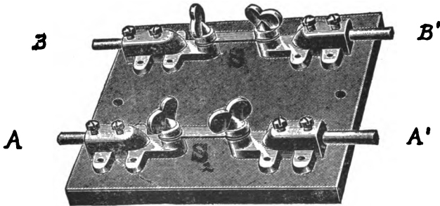
FIG. 10.—PAIR OF SAFETY STRIPS, MOUNTED ON FUSE-BLOCK.
