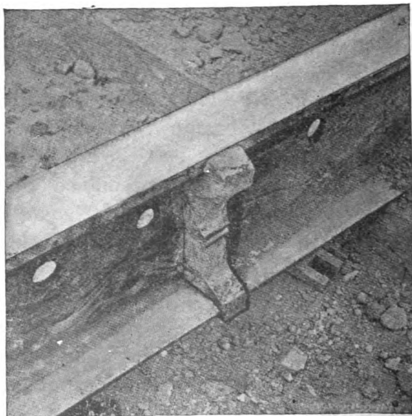
FIG. 76.—WELDED RAILS.
