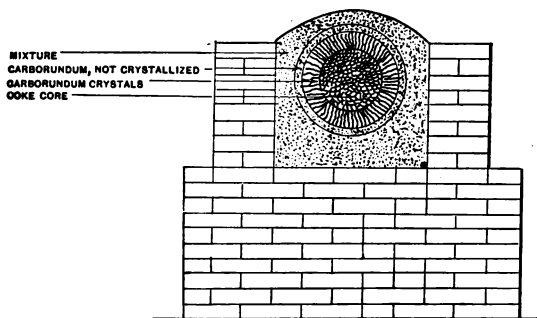
FIG. 80.—SECTION THROUGH FURNACE AFTER PASSAGE OF CURRENT.
