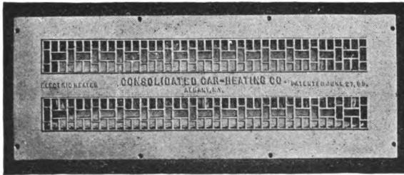
FIG. 23.—ELECTRIC CAR-HEATER.
