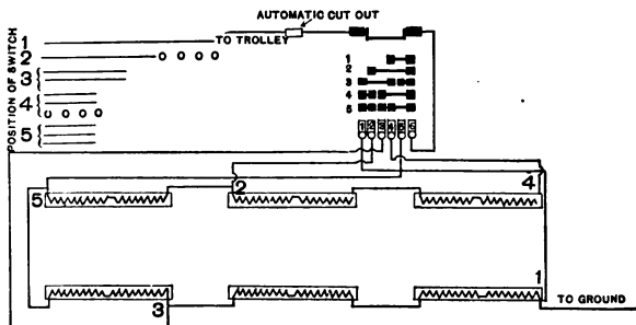
FIG. 28.—DIAGRAM OF WIRING FOR SIX ELECTRIC HEATER EQUIPMENT.
