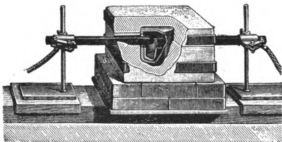
FIG. 77. —ELECTRIC FURNACE.
