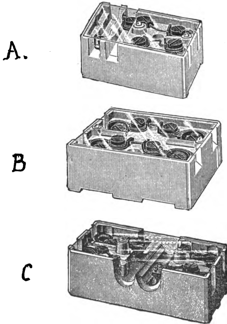
FIG. 12.—MICA-COVERED FUSE-BOXES.
