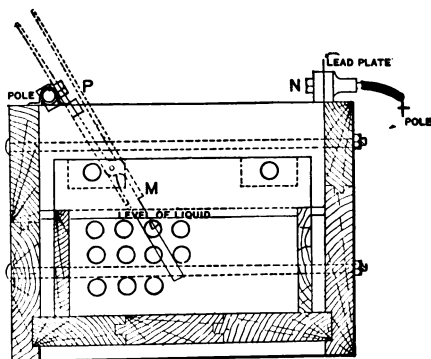
FIG. 85.—END VIEW OF HEATING TANK.
