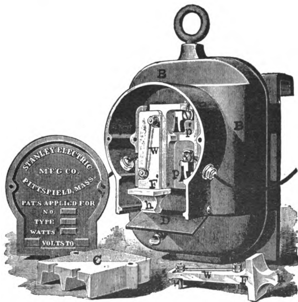
FIG. 20.—TRANSFORMER SAFETY FUSE-BOX
