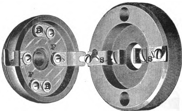
FIG. 16.—CEILING-FIXTURE FUSE-BLOCK.
