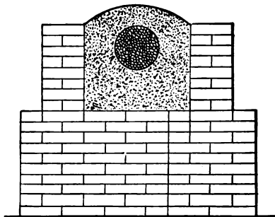
FIG. 79.—SECTION THROUGH FURNACE BEFORE PASSAGE OF CURRENT.
