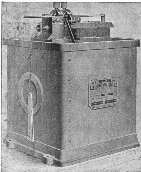
FIG. 65.—AUTOMATIC WELDER.
