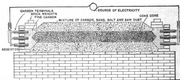
FIG. 78.—LONGITUDINAL SECTION OF CARBORUNDUM FURNACE.
