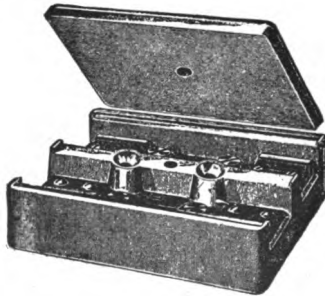
FIG. 14. — FUSE-BOX PROVIDED WITH PORCELAIN COVER.
