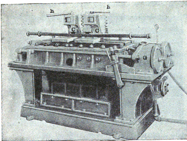
FIG. 67.—UNIVERSAL WELDER.
