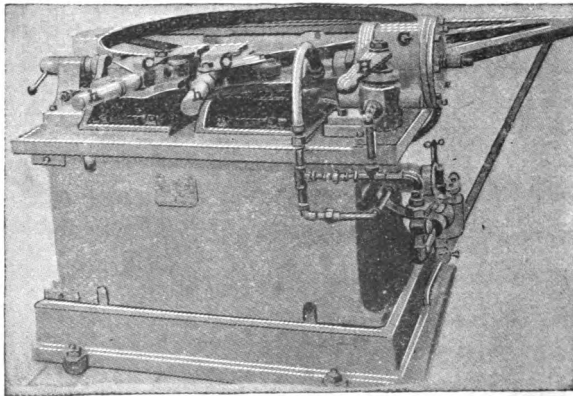
FIG. 66. - WELDER FOR CARRIAGE TIRES.
