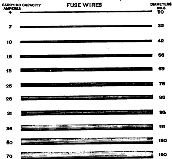
FIG. 4.—DIAMETER AND CARRYING CAPACITIES OF FUSE WIRES.
