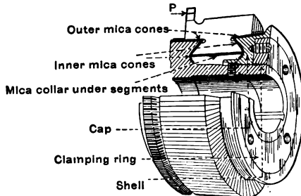
Fig. 33a. — SECTION VIEW OF COMMUTATOR.
