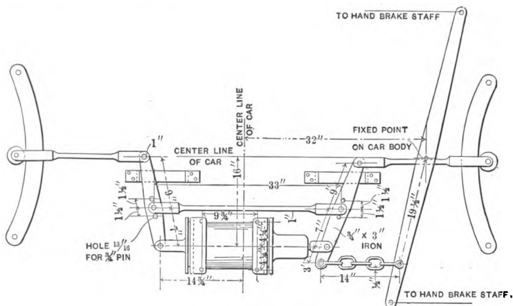
Fig. 149. — AIR BRAKE LEVERS.
