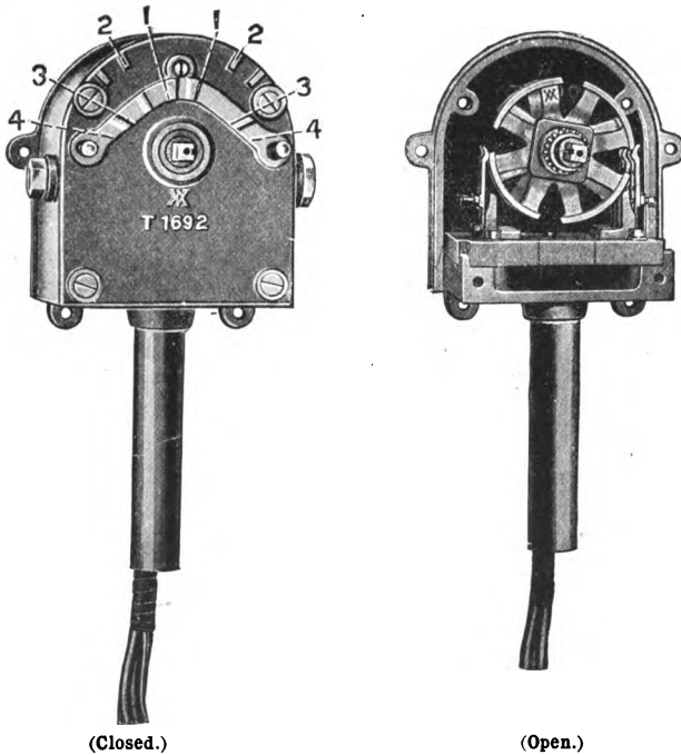
Fig. 79.—MULTIPLE CONTROL SWITCH.
