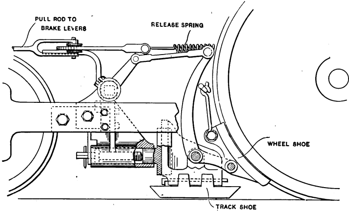
Fig. 145.—TRACK BRAKE.
