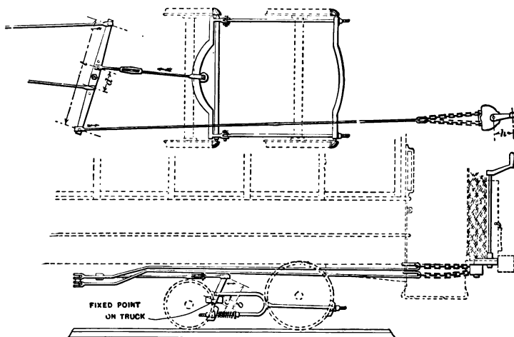
Fig. 144.—GEARED BRAKE.
