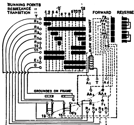
Fig. 73. — CONTROLLER CIRCUITS, K 10 CONTROL SYSTEM.
