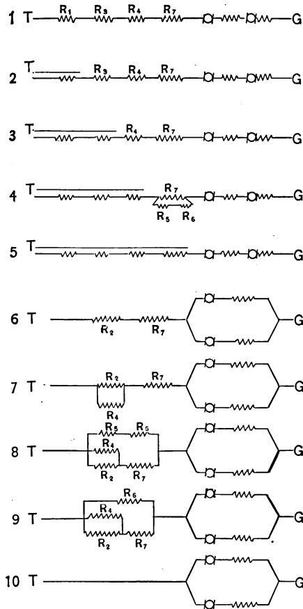
Fig. 71.—RESISTANCE COMBINATIONS TYPE M CONTROL.
