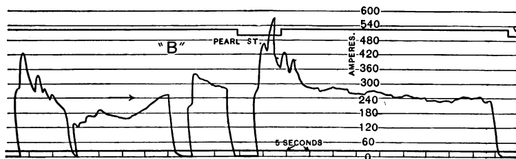
-Current curve taken by graphic recording ammeter on one of the Schenectady-Albany cars equipped with four GE-73 motors. This car was climbing a heavy grade and the motors were in series.
