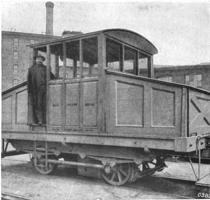
Fig. 162. — STORAGE-BATTERY LOCOMOTIVE.
