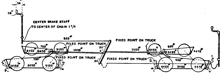
Fig. 142. — HAND BRAKE SYSTEM.
