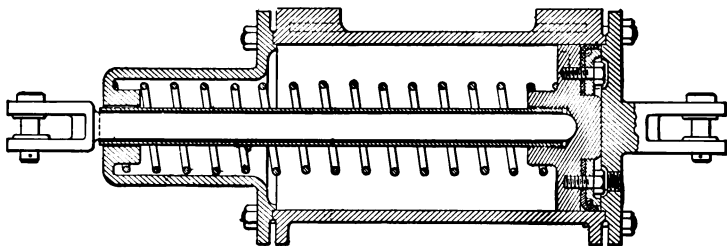
Fig. 147. — BRAKE CYLINDER.
