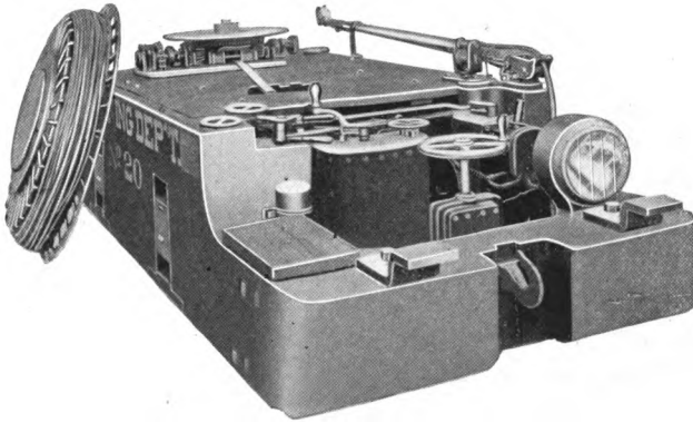
Fig. 159. —ELECTRIC MINING LOCOMOTIVE.
