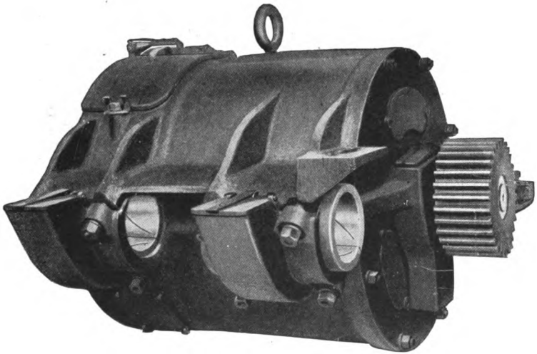
Fig. 59. — WESTINGHOUSE TYPE 91 A. C. MOTOR.
