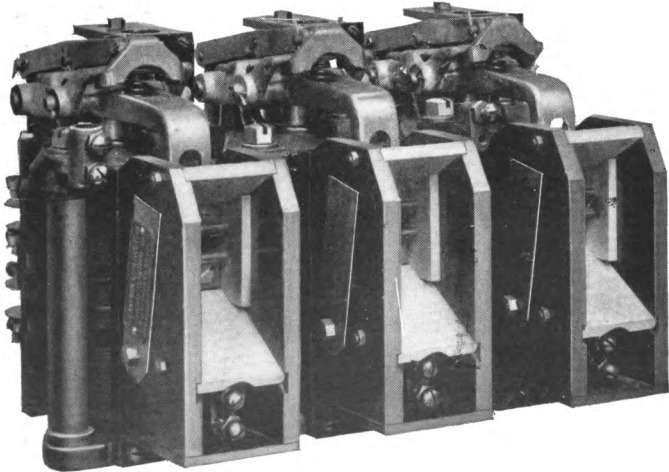
Fig. 98.—CONTACTOR WITH INTERLOCKING CONTACTS. (Rear View.)
