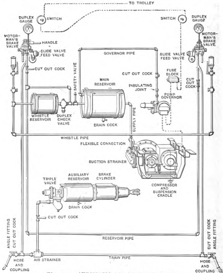
Fig. 151.—AUTOMATIC AIR BRAKE SYSTEM. (Installed on Interborough R. R., N.Y.)
