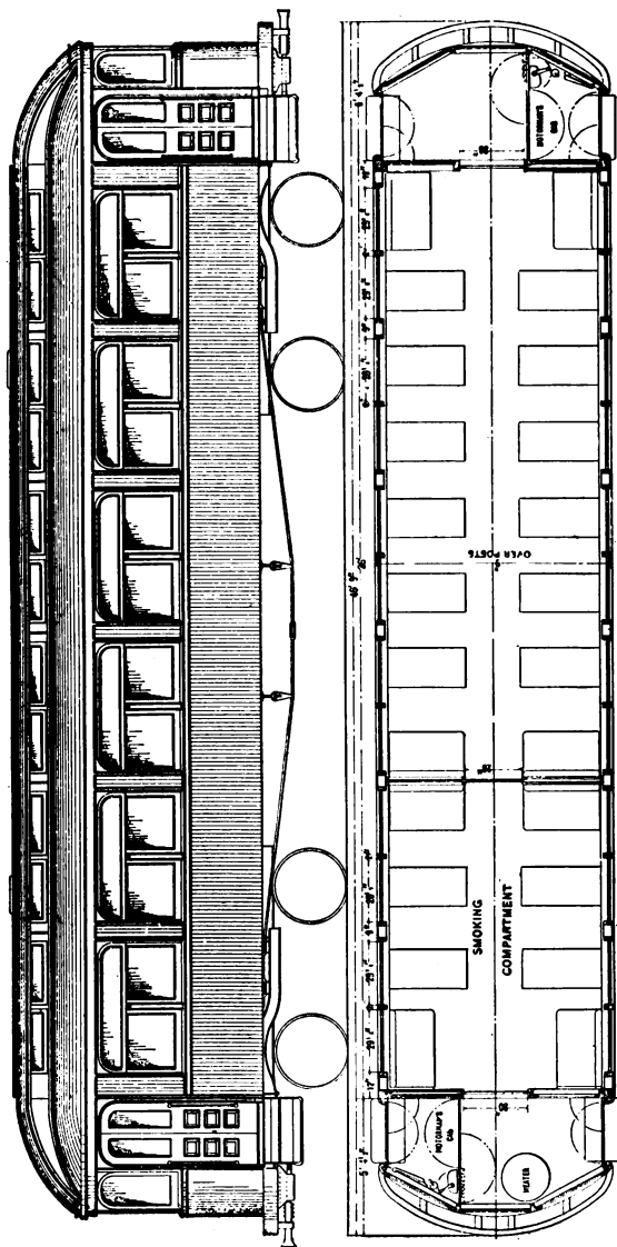
Figs. 107 and 108. — INTER-URBAN CAR.
