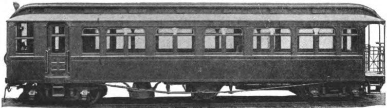
Fig. 87. — CAR SHOWING SWITCH GROUP IN POSITION.
