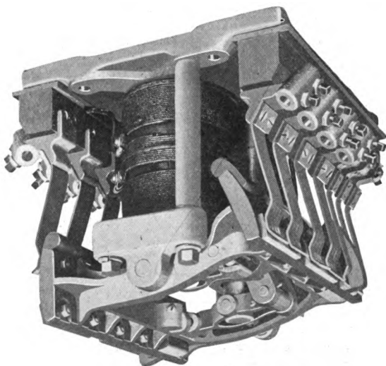
Fig. 69. — REVERSER, TYPE M CONTROL.
