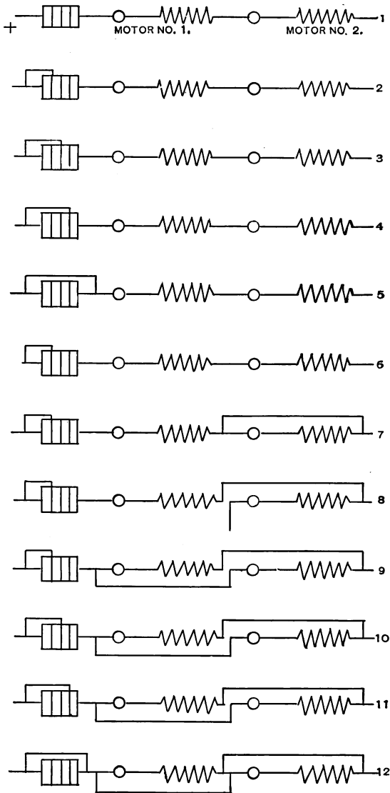
Fig. 75.—DIAGRAM OF K 10 MOTOR COMBINATIONS.
