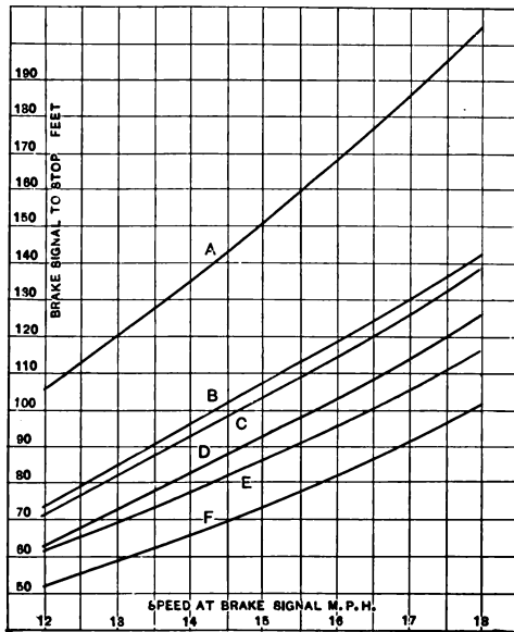
Fig. 140.—BRAKE TESTS.
