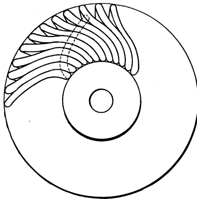
Fig. 31. — EICHEMEYER WINDING.
