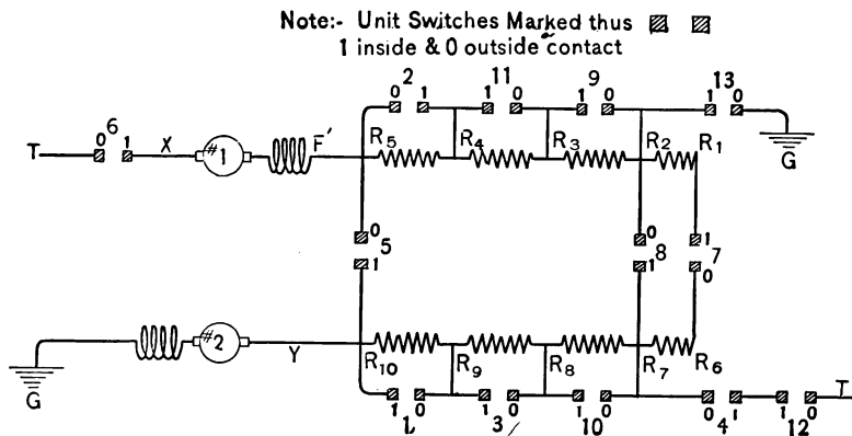
Fig. 92.—ELEMENTARY DIAGRAM OF CIRCUITS OF UNIT SWITCH CONTROL.
