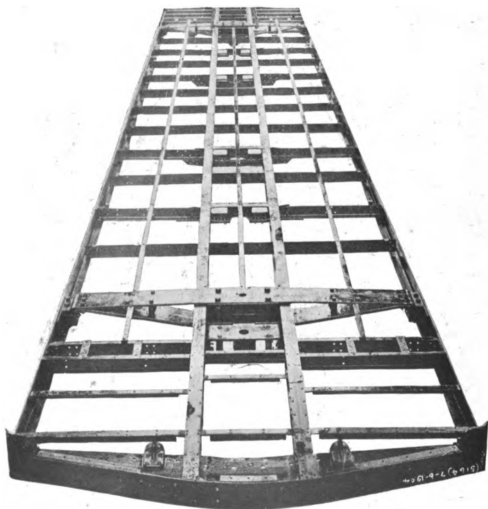
Fig. 117.—STEEL FLOOR FRAMING.
