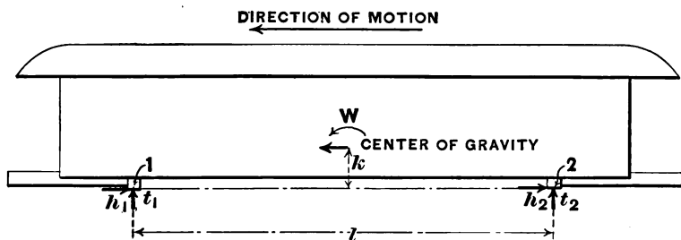
Fig. 135.—DIAGRAM OF FORCES ACTING UPON CAR BODY.
