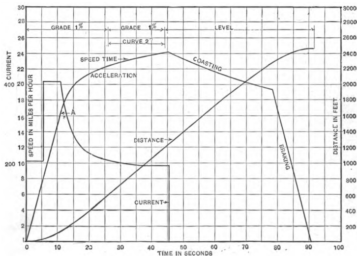
Fig. 19. — CALCULATED TRAIN CURVES.
