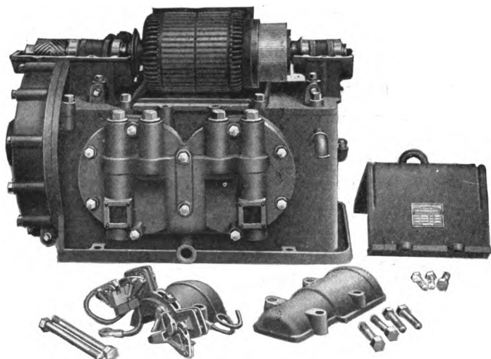
Fig. 153.—MOTOR DRIVEN AIR COMPRESSOR.
