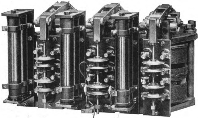
Fig. 97.—CONTACTOR WITH INTERLOCKING CONTACTS. (Front View.)
