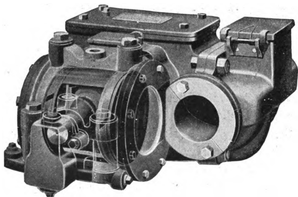
Fig. 155.—AIR COMPRESSOR AXLE DRIVER. (West. Traction Brake Co.)
