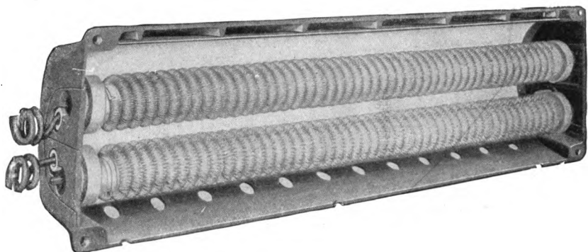
Fig. 111.—ELECTRIC HEATER COILS AND CASE.
