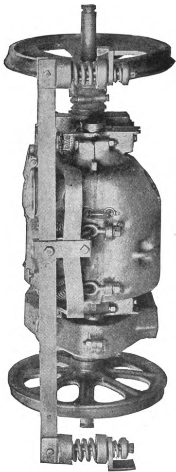
Fig. 42. - CRADLE SUSPENSION.
