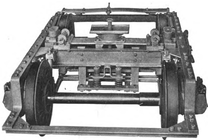
Fig. 128. — MOTOR SUSPENSION.
