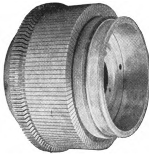
Fig. 33b. — COMMUTATOR COMPLETE.
