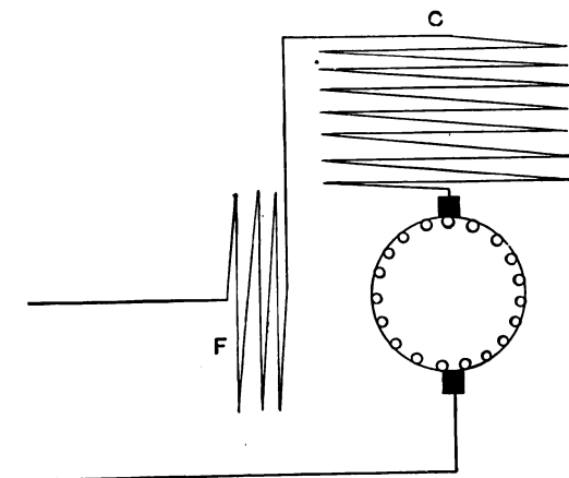
Fig. 48.—SINGLE PHASE MOTOR WITH REVERSE SERIES COMPENSATING WINDING.
