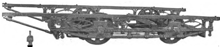
Fig. 123. — RIGID TRUCK.
