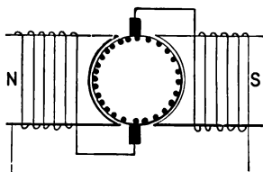
Fig. 51. — STRAIGHT SERIES DIRECT CURRENT MOTOR CIRCUITS.
