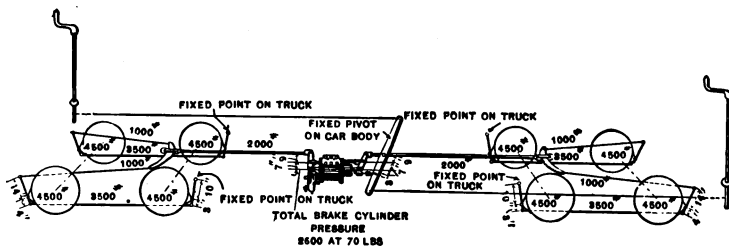
Fig. 148. —BRAKE CYLINDER AND LEVERS.
