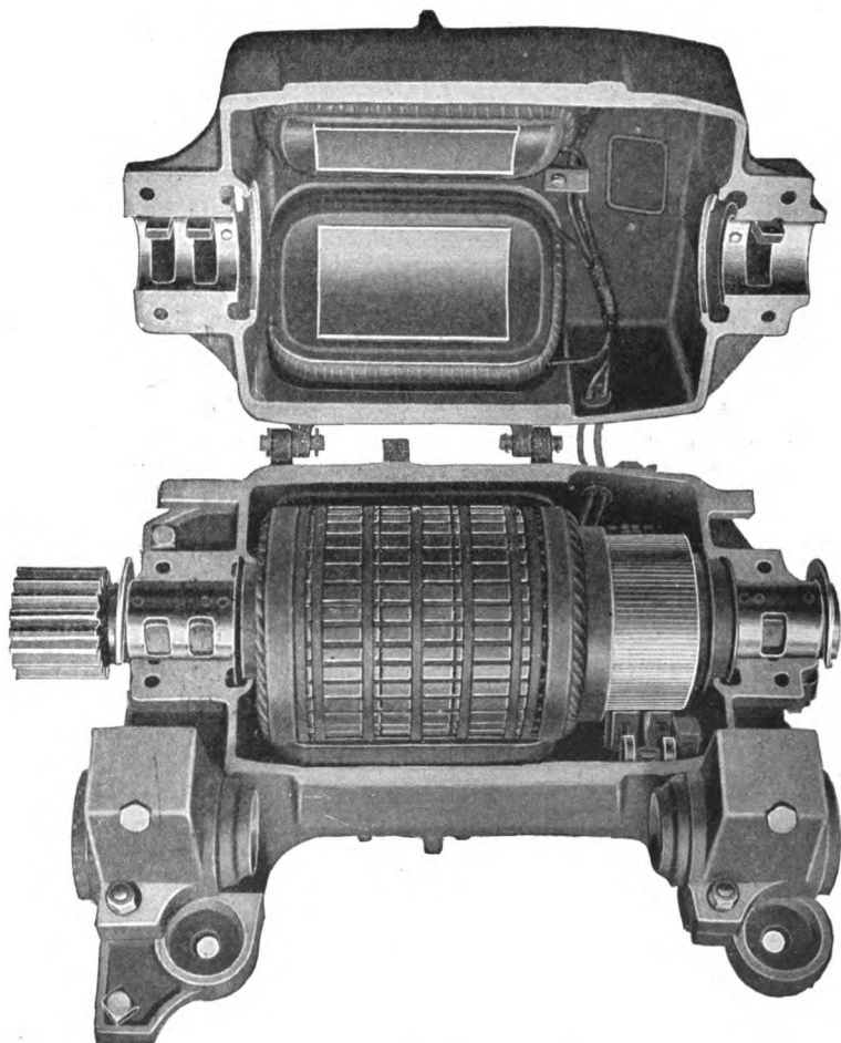
Fig. 46. — WESTINGHOUSE No. 56 RAILWAY MOTOR.
