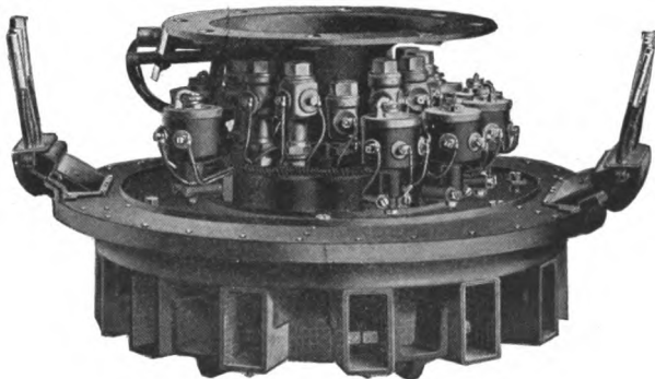
Fig. 85b. — THE SWITCH GROUP. (Covers Removed.)
