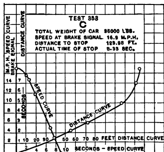
Fig. 141. — BRAKE TESTS.
