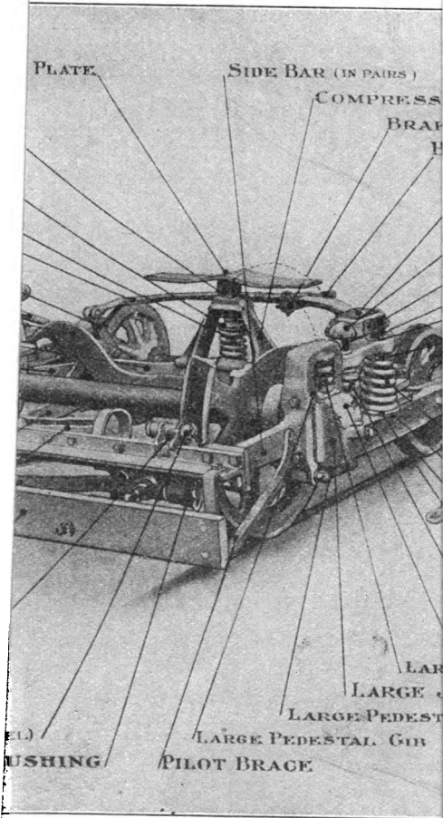
— MAXIMUM TRACTION TRUCK.
