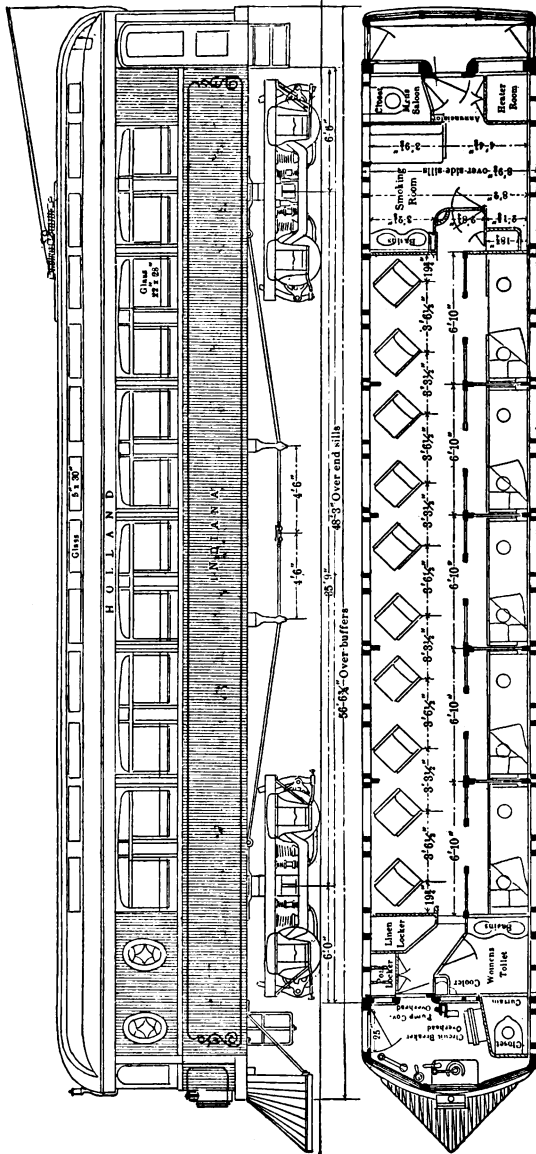
FIG. 106. — INTER-URBAN SLEEPING CAR.
