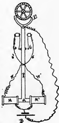
Fig. 38. ELECTRIC CLOCK.
