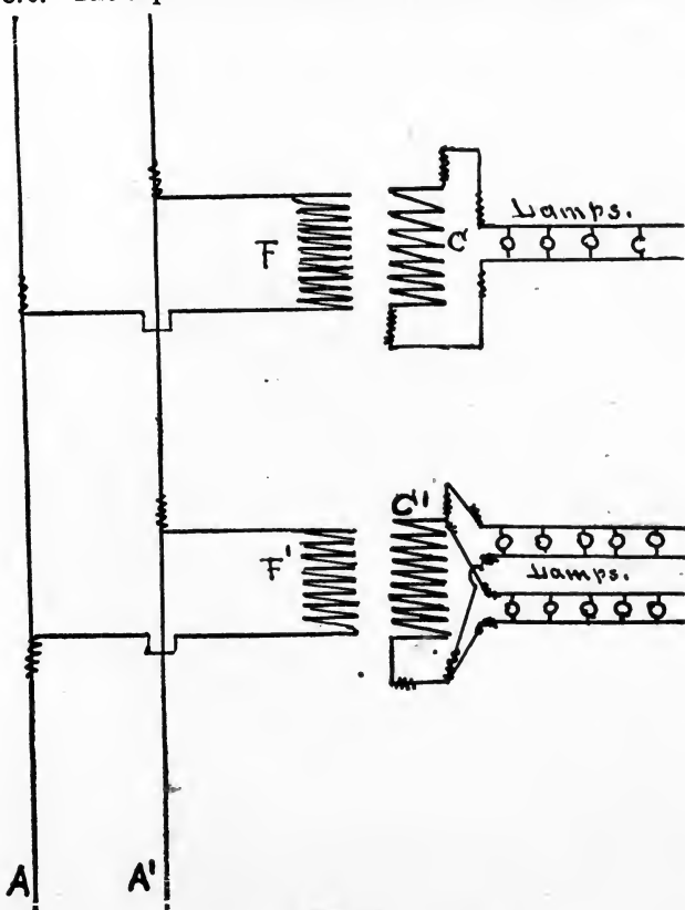
Fig. 104. TRANSFORMER CIRCUIT.
