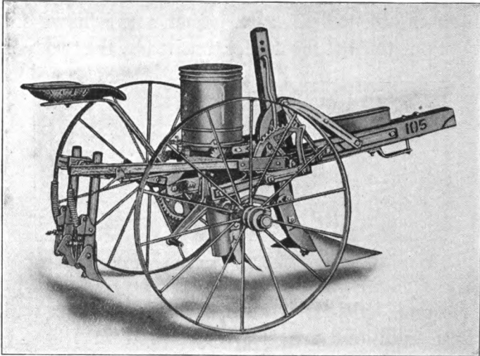
FIG. 150. COMBINED LISTER AND PLANTER
