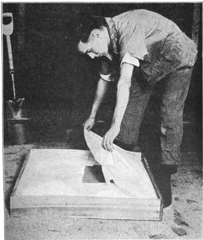
FIG. 101. COVERING THE TESTER
