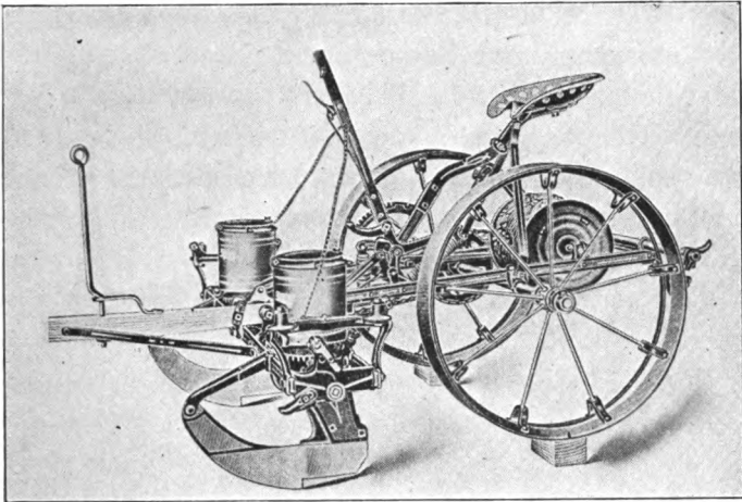
FIG. 153. CHECK-ROW PLANTER
