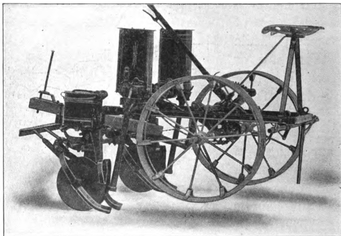
FIG. 144. DOUBLE-ROW PLANTER
