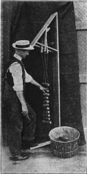
FIG. 82. STRINGING DEVICE
