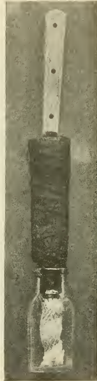
FIGURE 105. Sheath to hold knife. Two flat lamp wicks sewed together at their edges and covered with tape, the lower end immersed in alcohol, keep the knife blade sterile.
