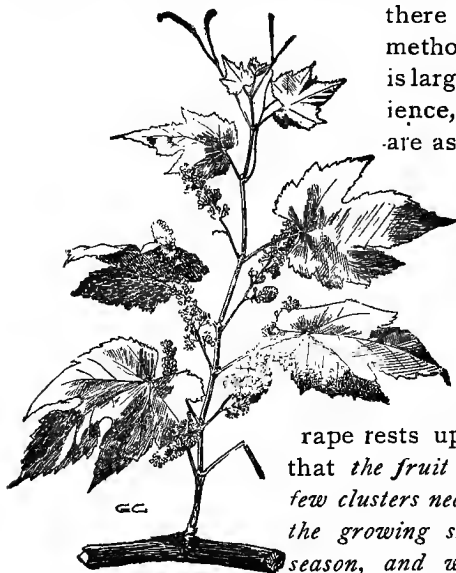
1. GRAPE SHOOT.
