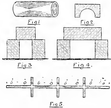
VENTILATING A POTATO CLAMP.
