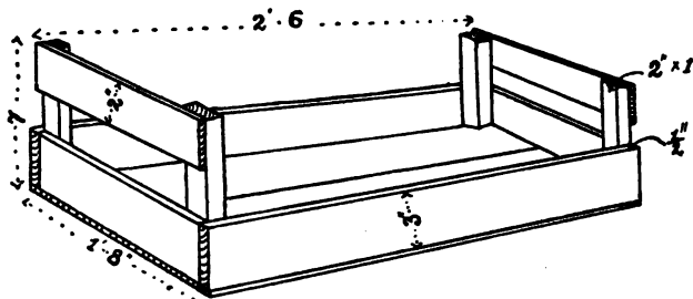
FIG. II.—A USEFUL POTATO TRAY FOR THE STORAGE AND SPROUTING OF SEED POTATOES
