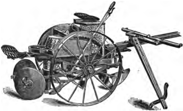
FIG. 28—THE ROBBINS IMPROVED PLANTER
