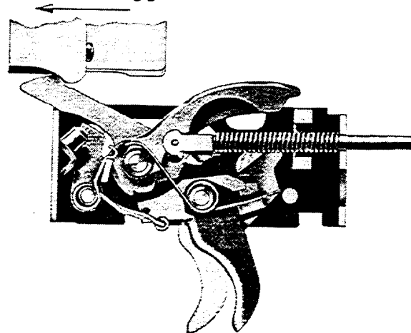
Ill.# 49A - Semiautomatic fire
