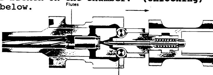
Ill.# 47B - Bolt group in unlocked position
