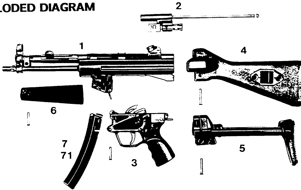
Exploded Diagram # 1 - Assembly Groups
